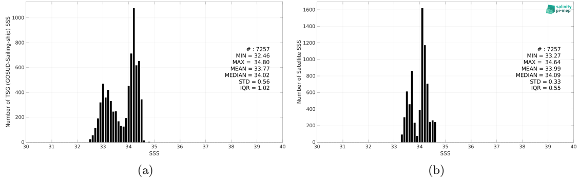
Figure 2: Histograms of SSS from TSG (GOSUD-Sailing-ship) (a) and SMOS SSS L3 v8 - 18 Days (CATDS-CEC-LOCEAN) (b) considering all match-up pairs per bins of 0.1 over the SPURS 2 Pi-MEP region and for the full satellite product period.
