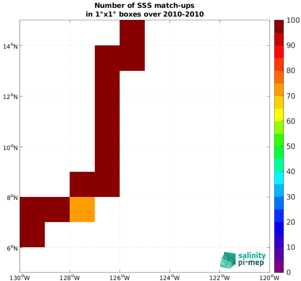
Figure 4: Number of SSS match-ups between TSG (GOSUD-Sailing-ship) SSS and the SMOS SSS L3 v8 - 18 Days (CATDS-CEC-LOCEAN) SSS product for the SPURS 2 Pi-MEP region over 1^\circ \times 1^\circ boxes and for the full satellite product period.
