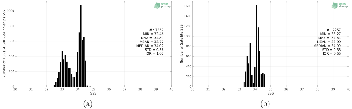
Figure 2: Histograms of SSS from TSG (GOSUD-Sailing-ship) (a) and SMOS SSS L3 v8 - 18 Days (CATDS-CECOS-LOCEAN) (b) considering all match-up pairs per bins of 0.1 over the SPURS 2 Pi-MEP region and for the full satellite product period.
