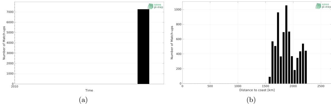
Figure 1: Number of match-ups between TSG (GOSUD-Sailing-ship) and SMOS SSS L3 v8 - 18 Days (CATDS-CECOS-LOCEAN) SSS as a function of time (a) and as function of the distance to coast (b) over the SPURS 2 Pi-MEP region and for the full satellite product period.
