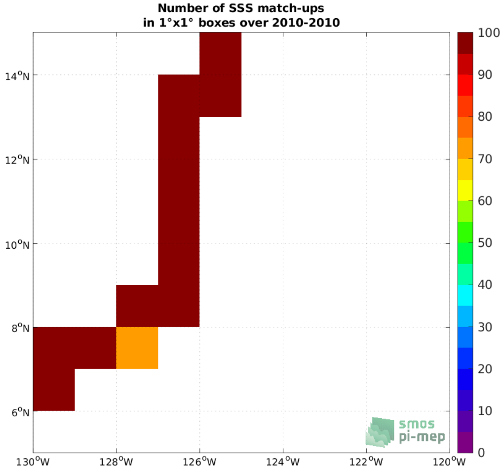
Figure 4: Number of SSS match-ups between TSG (GOSUD-Sailing-ship) SSS and the SMOS SSS L3 v8 - 18 Days (CATDS-CECOS-LOCEAN) SSS product for the SPURS 2 Pi-MEP region over 1^\circ \times 1^\circ boxes and for the full satellite product period.
