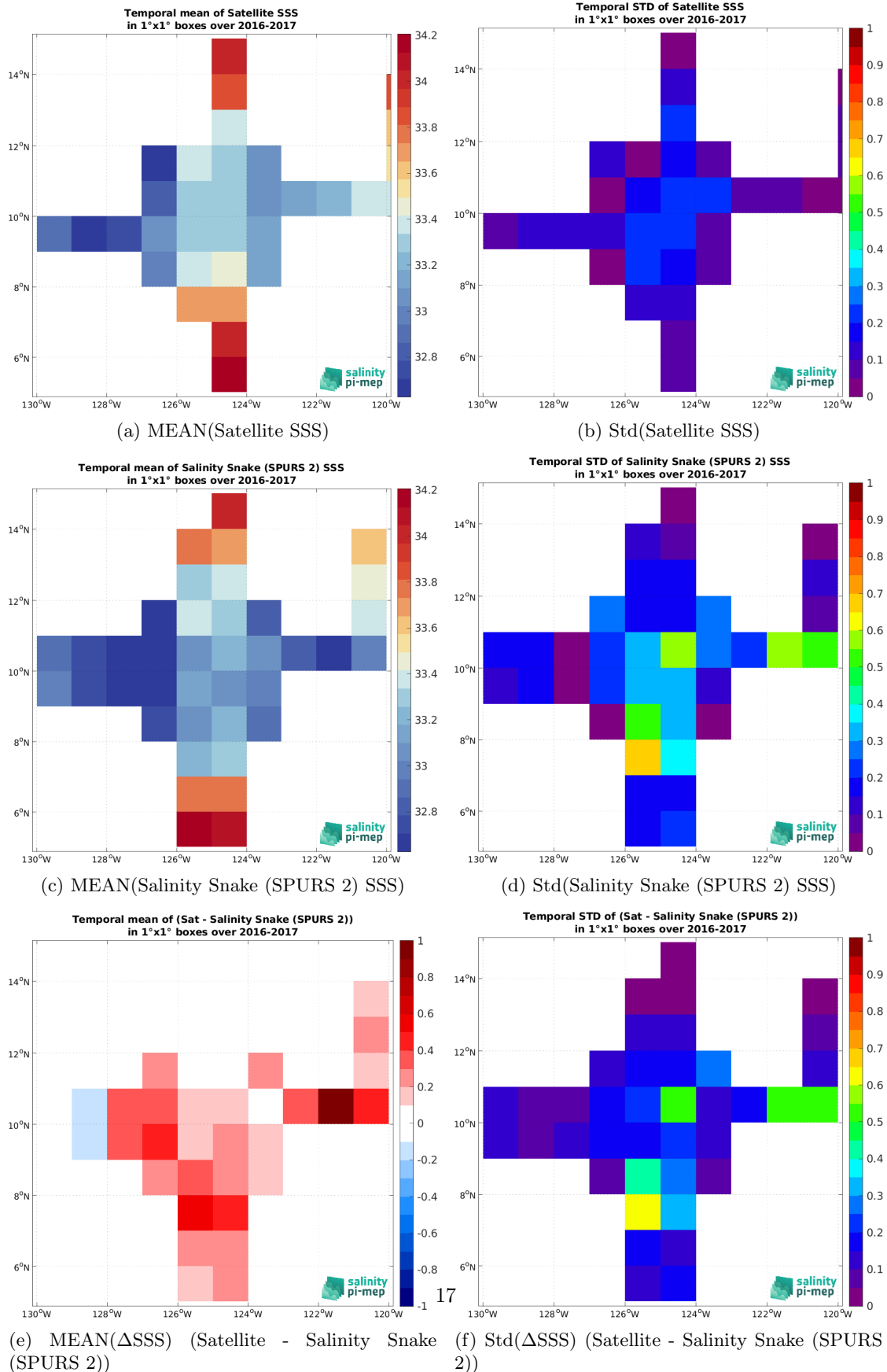
Figure 6: Temporal mean (left) and Std (right) of SSS from SMOS SSS L3 v8 - 18 Days (CATDS-CEC-LOCEAN) (top), Salinity Snake (SPURS 2) (middle), and of \Delta SSS (Satellite - Salinity Snake (SPURS 2)). Only match-up pairs are used to generate these maps.
