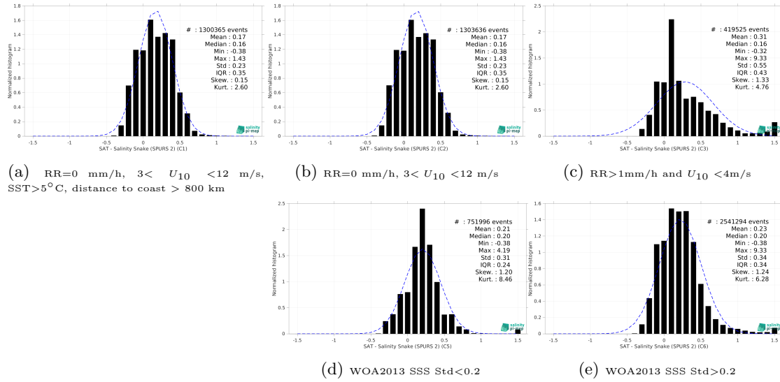
Figure 13: Normalized histogram of \Delta SSS (SMOS SSS L3 v8 - 18 Days (CATDS-CEC-LOCEAN) - Salinity Snake (SPURS 2)) for 5 different subdatasets corresponding to: RR=0 mm/h, 3 < U_{10} < 12 m/s, SST>5°C, distance to coast > 800 km (a), RR=0 mm/h, 3 < U_{10} < 12 m/s (b), RR>1mm/h and U_{10} < 4 m/s (c), WOA2013 SSS Std<0.2 (d), WOA2013 SSS Std>0.2 (e).
