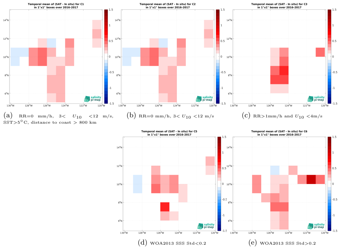
Figure 12: Temporal mean gridded over spatial boxes of size 1^\circ \times 1^\circ of \Delta SSS (SMOS SSS L3 v8 - 18 Days (CATDS-CEC-LOCEAN) - Salinity Snake (SPURS 2)) for 5 different subdatasets corresponding to: RR=0 mm/h, 3 < U_{10} < 12 m/s, SST > 5°C, distance to coast > 800 km (a), RR=0 mm/h, 3 < U_{10} < 12 m/s (b), RR > 1mm/h and U_{10} < 4 m/s (c), WOA2013 SSS Std < 0.2 (d), WOA2013 SSS Std > 0.2 (e).
