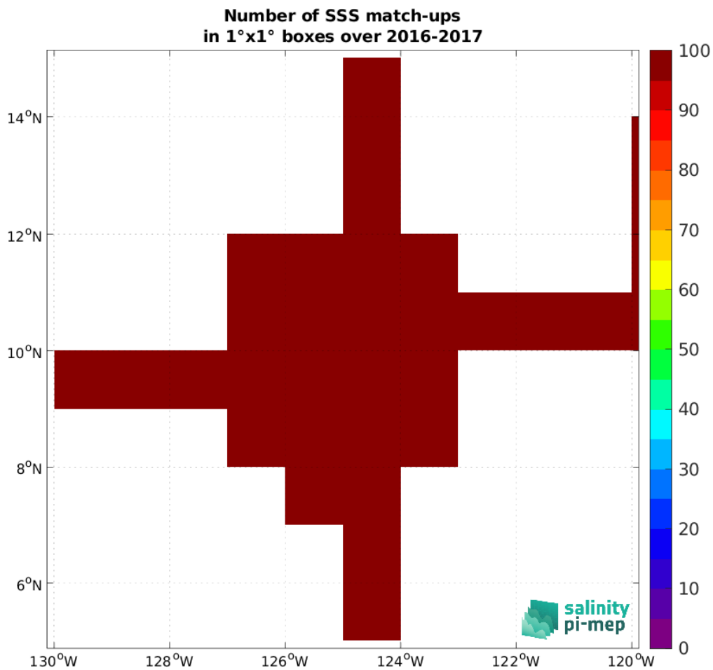
Figure 4: Number of SSS match-ups between Salinity Snake (SPURS 2) SSS and the SMOS SSS L3 v8 - 18 Days (CATDS-CEC-LOCEAN) SSS product for the SPURS 2 Pi-MEP region over 1^\circ \times 1^\circ boxes and for the full satellite product period.
