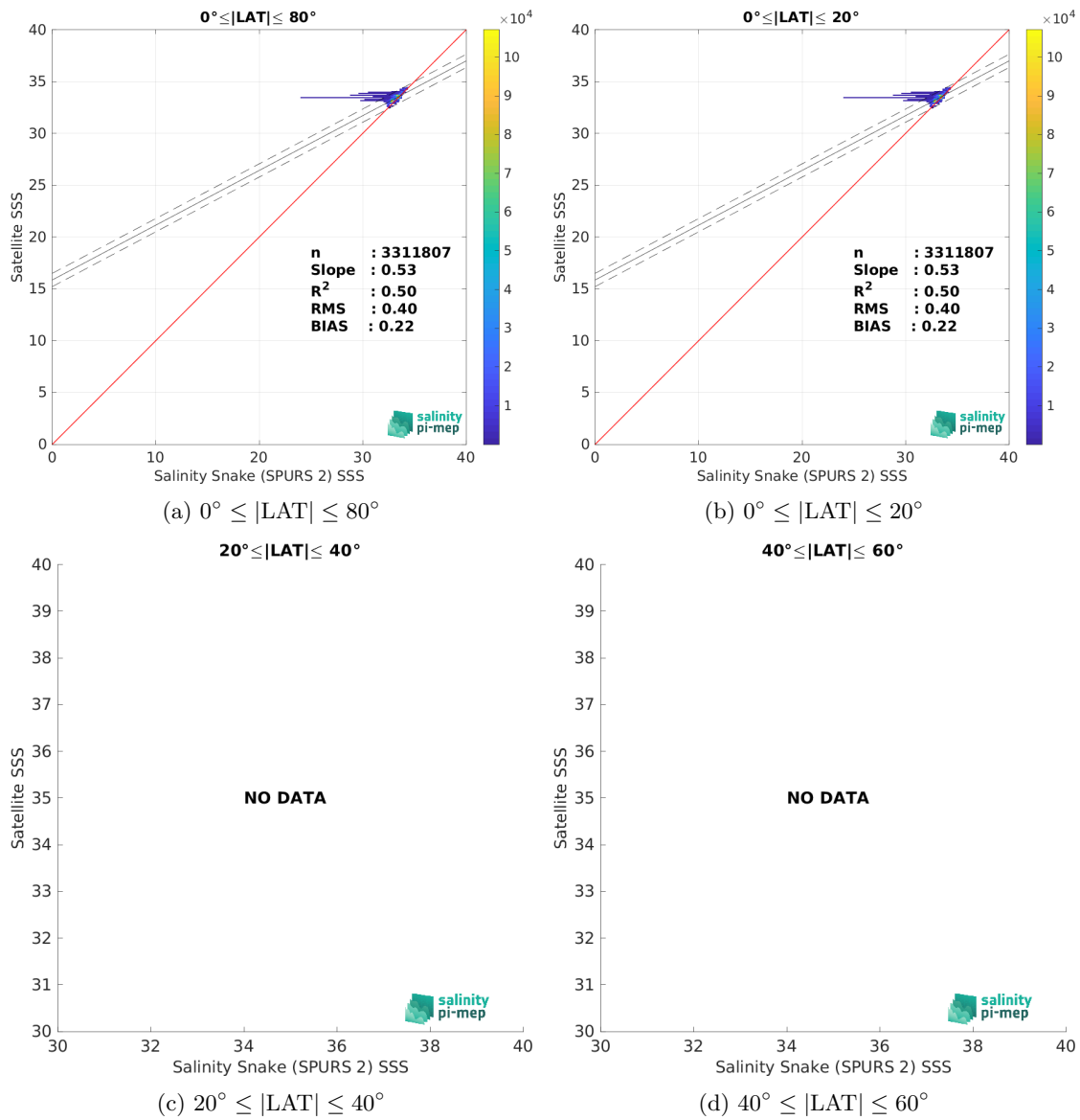
Figure 9: Contour maps of the concentration of SMOS SSS L3 v8 - 18 Days (CATDS-CEC-LOCEAN) SSS (y-axis) versus Salinity Snake (SPURS 2) SSS (x-axis) at match-up pairs for different latitude bands. For each plot, the red line shows x=y . The black thin and dashed lines indicate a linear fit through the data cloud and the \pm 95\% confidence levels, respectively. The number match-up pairs n , the slope and R^2 coefficient of the linear fit, the root mean square (RMS) and the mean bias between satellite and in situ data are indicated for each latitude band in each plots.
