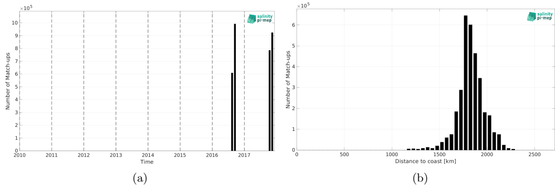
Figure 1: Number of match-ups between Salinity Snake (SPURS 2) and SMOS SSS L3 v8 - 18 Days (CATDS-CEC-LOCEAN) SSS as a function of time (a) and as function of the distance to coast (b) over the SPURS 2 Pi-MEP region and for the full satellite product period.
