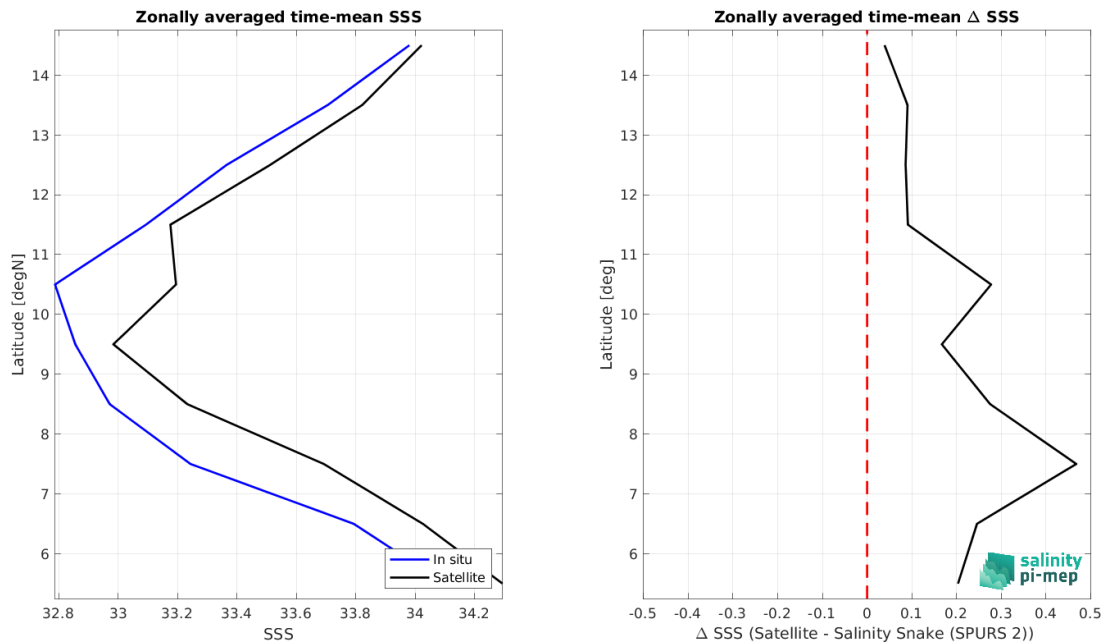
Figure 8: Left panel: Zonal mean SSS from SMOS SSS L3 v8 - 18 Days (CATDS-CEC-LOCEAN) satellite product (black) and from Salinity Snake (SPURS 2) (blue). Right panel: Zonal mean of \Delta SSS (Satellite - Salinity Snake (SPURS 2)) for all the collected Pi-MEP match-up pairs estimated over the full satellite product period.
