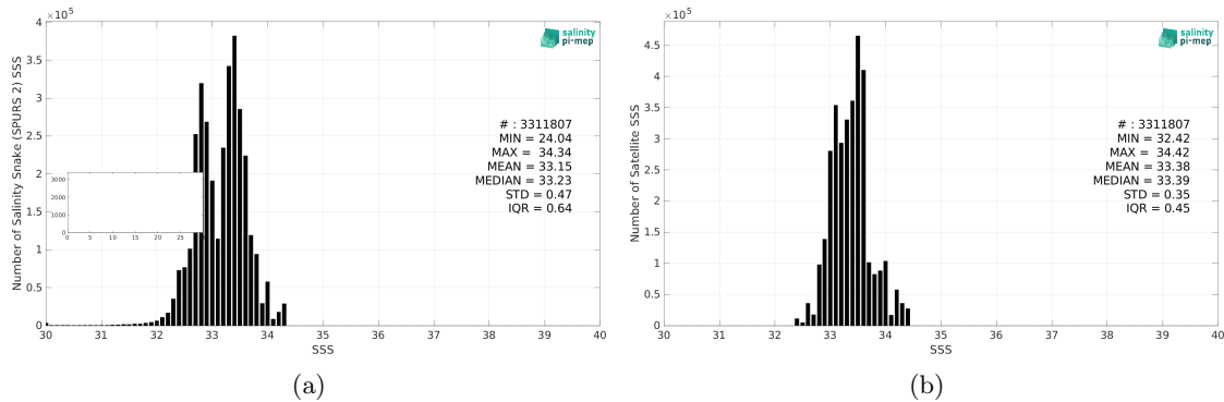
Figure 2: Histograms of SSS from Salinity Snake (SPURS 2) (a) and SMOS SSS L3 v8 - 18 Days (CATDS-CEC-LOCEAN) (b) considering all match-up pairs per bins of 0.1 over the SPURS 2 Pi-MEP region and for the full satellite product period.
