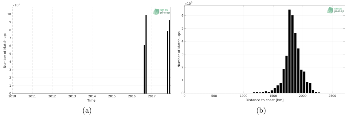
Figure 1: Number of match-ups between Salinity Snake (SPURS 2) and SMOS SSS L3 v8 - 18 Days (CATDS-CECOS-LOCEAN) SSS as a function of time (a) and as function of the distance to coast (b) over the SPURS 2 Pi-MEP region and for the full satellite product period.
