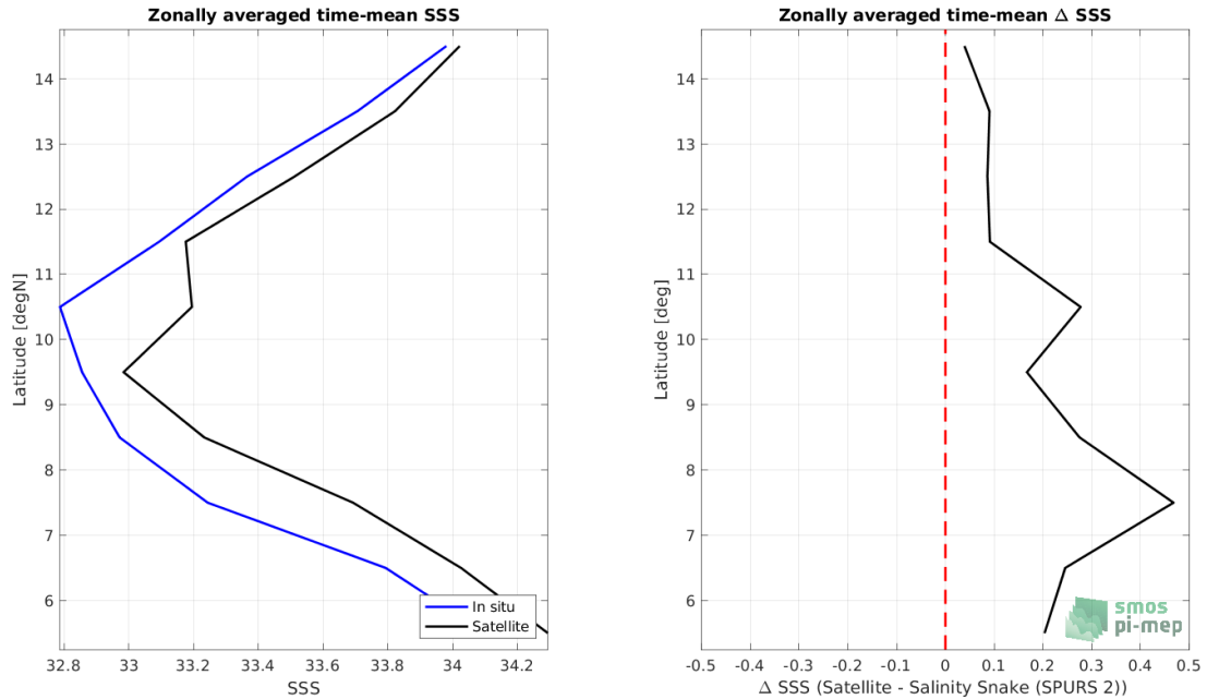
Figure 8: Left panel: Zonal mean SSS from SMOS SSS L3 v8 - 18 Days (CATDS-CECOS-LOCEAN) satellite product (black) and from Salinity Snake (SPURS 2) (blue). Right panel: Zonal mean of \Delta SSS (Satellite - Salinity Snake (SPURS 2)) for all the collected Pi-MEP match-up pairs estimated over the full satellite product period.
