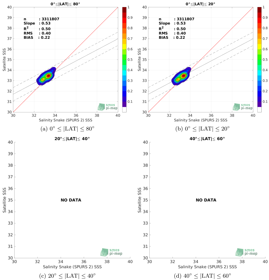
Figure 9: Contour maps of the concentration of SMOS SSS L3 v8 - 18 Days (CATDS-CECOS-LOCEAN) SSS (y-axis) versus Salinity Snake (SPURS 2) SSS (x-axis) at match-up pairs for different latitude bands. For each plot, the red line shows x=y . The black thin and dashed lines indicate a linear fit through the data cloud and the \pm 95\% confidence levels, respectively. The number match-up pairs n , the slope and R^2 coefficient of the linear fit, the root mean square (RMS) and the mean bias between satellite and in situ data are indicated for each latitude band in each plots.
