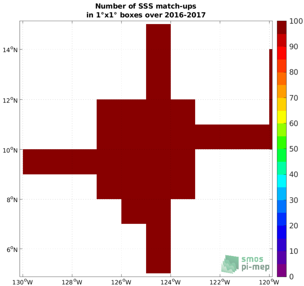
Figure 4: Number of SSS match-ups between Salinity Snake (SPURS 2) SSS and the SMOS SSS L3 v8 - 18 Days (CATDS-CECOS-LOCEAN) SSS product for the SPURS 2 Pi-MEP region over 1^\circ \times 1^\circ boxes and for the full satellite product period.
