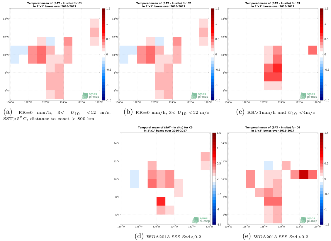
Figure 12: Temporal mean gridded over spatial boxes of size 1^\circ \times 1^\circ of \Delta SSS (SMOS SSS L3 v8 - 18 Days (CATDS-CECOS-LOCEAN) - Salinity Snake (SPURS 2)) for 5 different subdatasets corresponding to: RR=0 mm/h, 3 < U_{10} < 12 m/s, SST > 5°C, distance to coast > 800 km (a), RR=0 mm/h, 3 < U_{10} < 12 m/s (b), RR > 1mm/h and U_{10} < 4 m/s (c), WOA2013 SSS Std < 0.2 (d), WOA2013 SSS Std > 0.2 (e).
