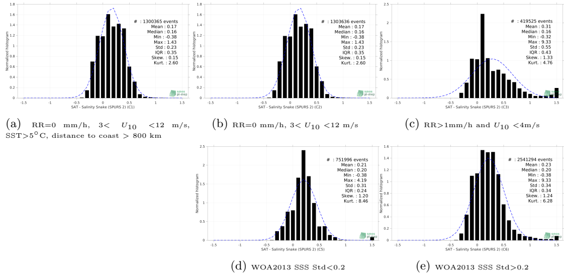
Figure 13: Normalized histogram of \Delta SSS (SMOS SSS L3 v8 - 18 Days (CATDS-CECOS-LOCEAN) - Salinity Snake (SPURS 2)) for 5 different subdatasets corresponding to: RR=0 mm/h, 3 < U_{10} < 12 m/s, SST > 5°C, distance to coast > 800 km (a), RR=0 mm/h, 3 < U_{10} < 12 m/s (b), RR > 1mm/h and U_{10} < 4 m/s (c), WOA2013 SSS Std < 0.2 (d), WOA2013 SSS Std > 0.2 (e).
