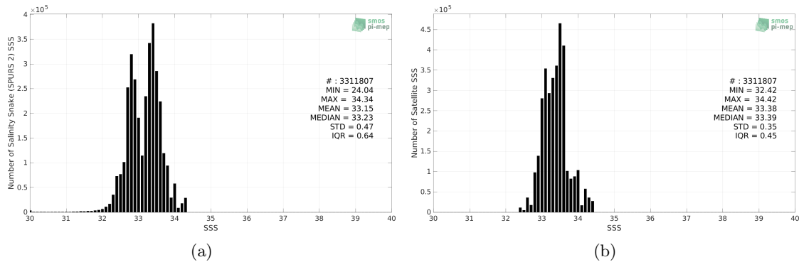
Figure 2: Histograms of SSS from Salinity Snake (SPURS 2) (a) and SMOS SSS L3 v8 - 18 Days (CATDS-CECOS-LOCEAN) (b) considering all match-up pairs per bins of 0.1 over the SPURS 2 Pi-MEP region and for the full satellite product period.
