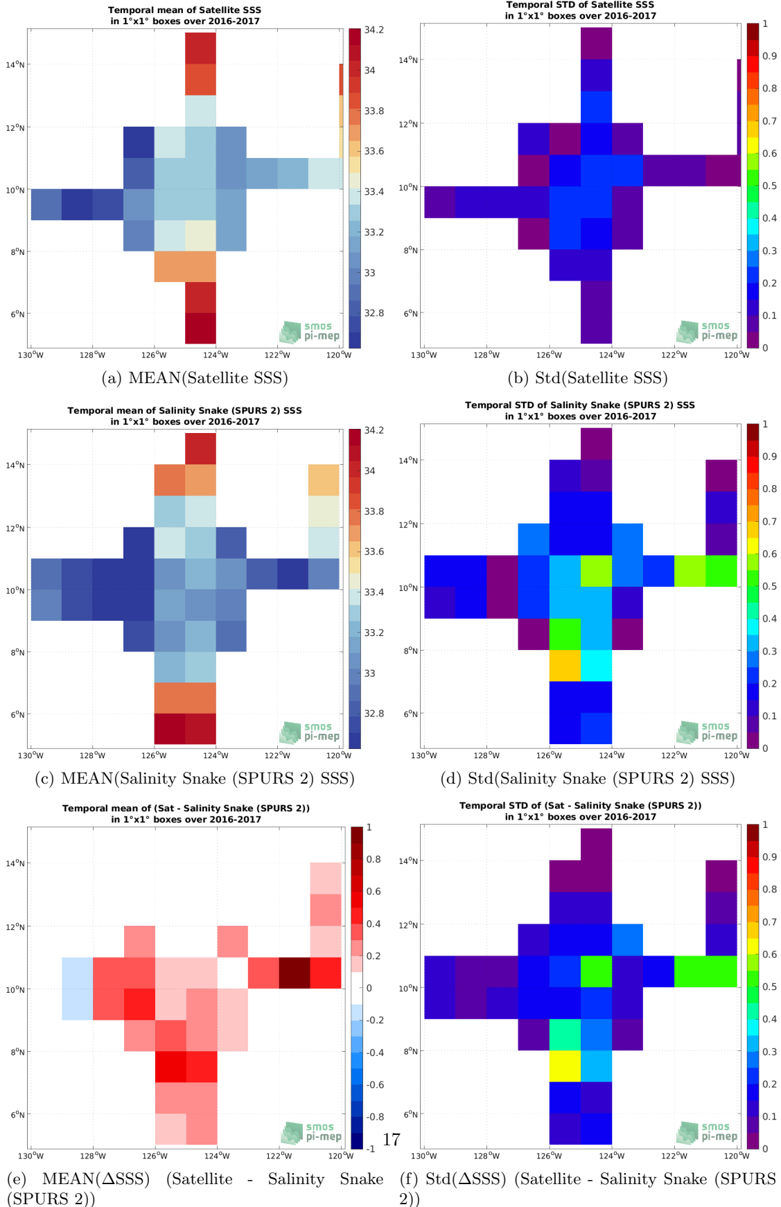
Figure 6: Temporal mean (left) and Std (right) of SSS from SMOS SSS L3 v8 - 18 Days (CATDS-CECOS-LOCEAN) (top), Salinity Snake (SPURS 2) (middle), and of \Delta SSS (Satellite - Salinity Snake (SPURS 2)). Only match-up pairs are used to generate these maps.
