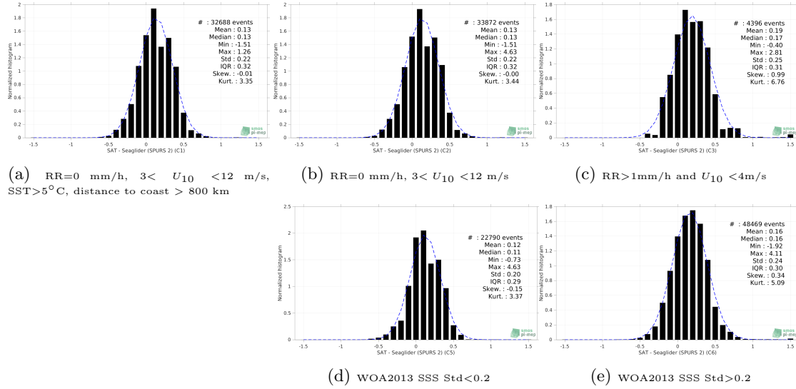
Figure 13: Normalized histogram of \Delta SSS (SMOS SSS L3 v8 - 18 Days (CATDS-CECOS-LOCEAN) - Seaglider (SPURS 2)) for 5 different subdatasets corresponding to: RR=0 mm/h, 3 < U_{10} < 12 m/s, SST > 5°C, distance to coast > 800 km (a), RR=0 mm/h, 3 < U_{10} < 12 m/s (b), RR > 1mm/h and U_{10} < 4 m/s (c), WOA2013 SSS Std < 0.2 (d), WOA2013 SSS Std > 0.2 (e).
