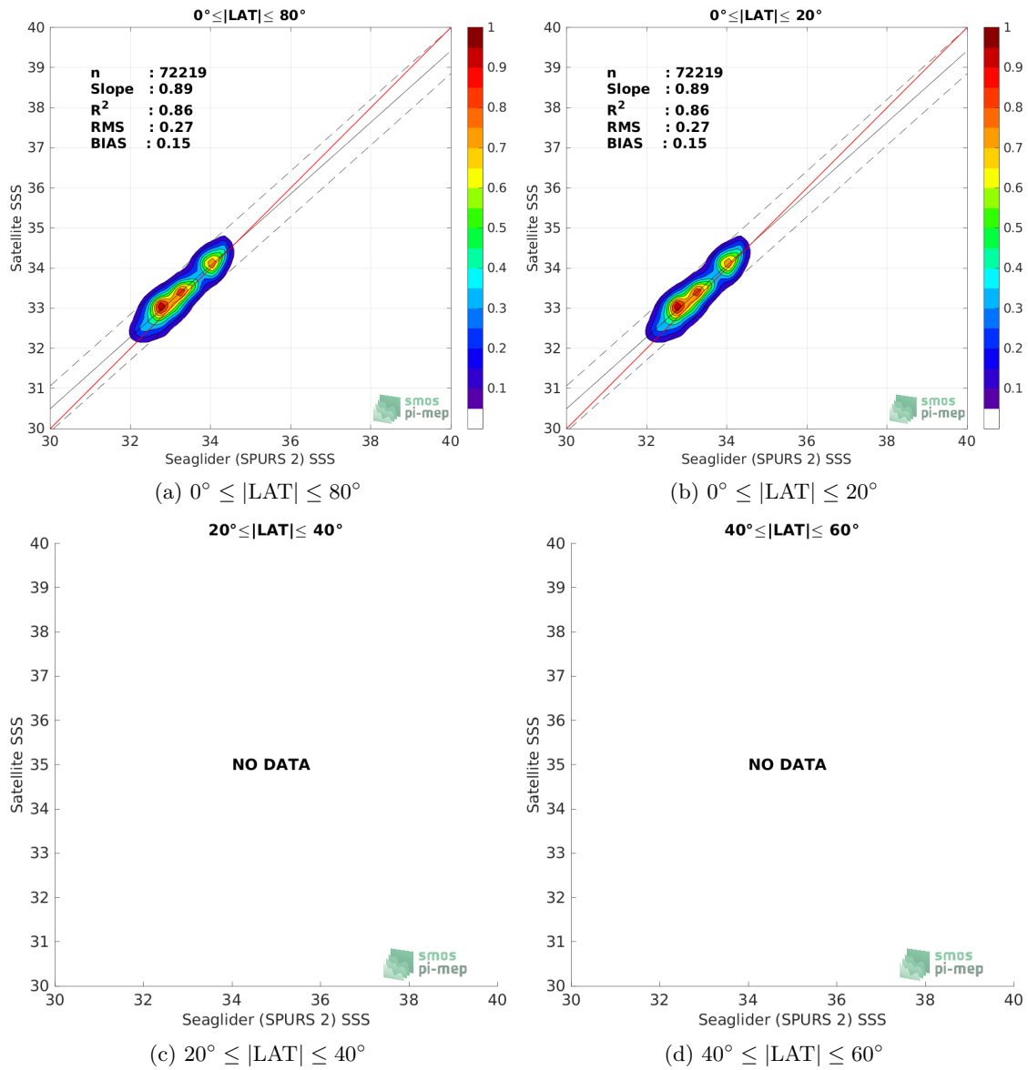
Figure 9: Contour maps of the concentration of SMOS SSS L3 v8 - 18 Days (CATDS-CECOS-LOCEAN) SSS (y-axis) versus Seaglider (SPURS 2) SSS (x-axis) at match-up pairs for different latitude bands. For each plot, the red line shows x=y . The black thin and dashed lines indicate a linear fit through the data cloud and the \pm 95\% confidence levels, respectively. The number match-up pairs n , the slope and R^2 coefficient of the linear fit, the root mean square (RMS) and the mean bias between satellite and in situ data are indicated for each latitude band in each plots.
