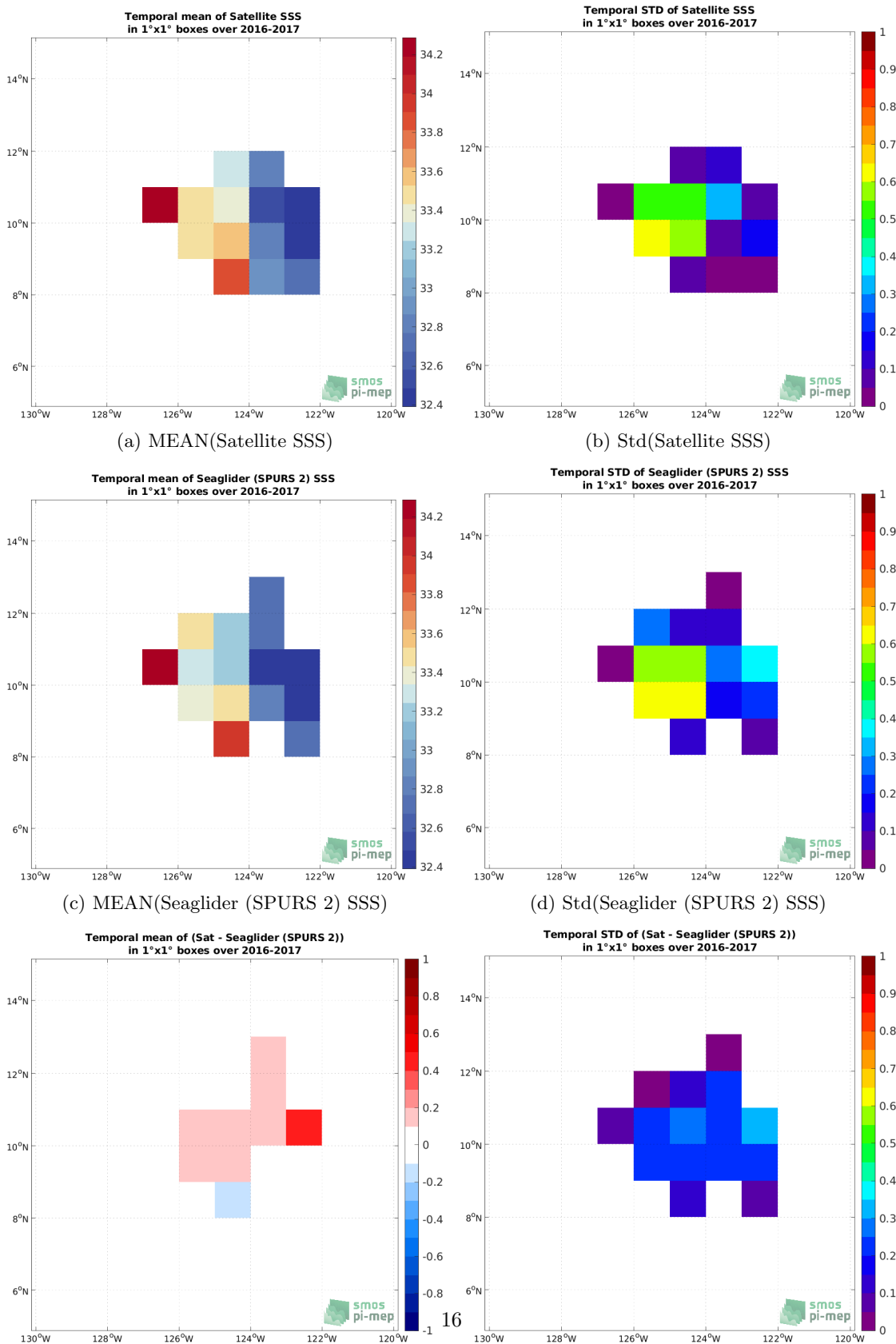
Figure 6: Temporal mean (left) and Std (right) of SSS from SMOS SSS L3 v8 - 18 Days (CATDS-CECOS-LOCEAN) (top), Seaglider (SPURS 2) (middle), and of \Delta SSS (Satellite - Seaglider (SPURS 2)). Only match-up pairs are used to generate these maps.
