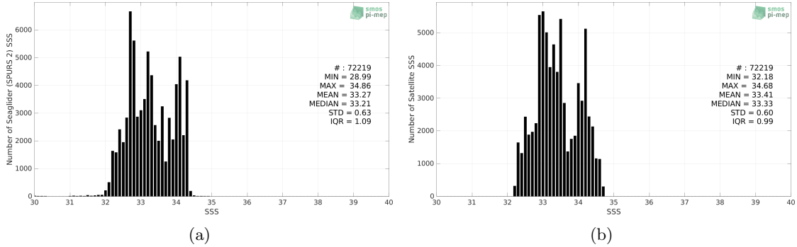
Figure 2: Histograms of SSS from Seaglider (SPURS 2) (a) and SMOS SSS L3 v8 - 18 Days (CATDS-CECOS-LOCEAN) (b) considering all match-up pairs per bins of 0.1 over the SPURS 2 Pi-MEP region and for the full satellite product period.
