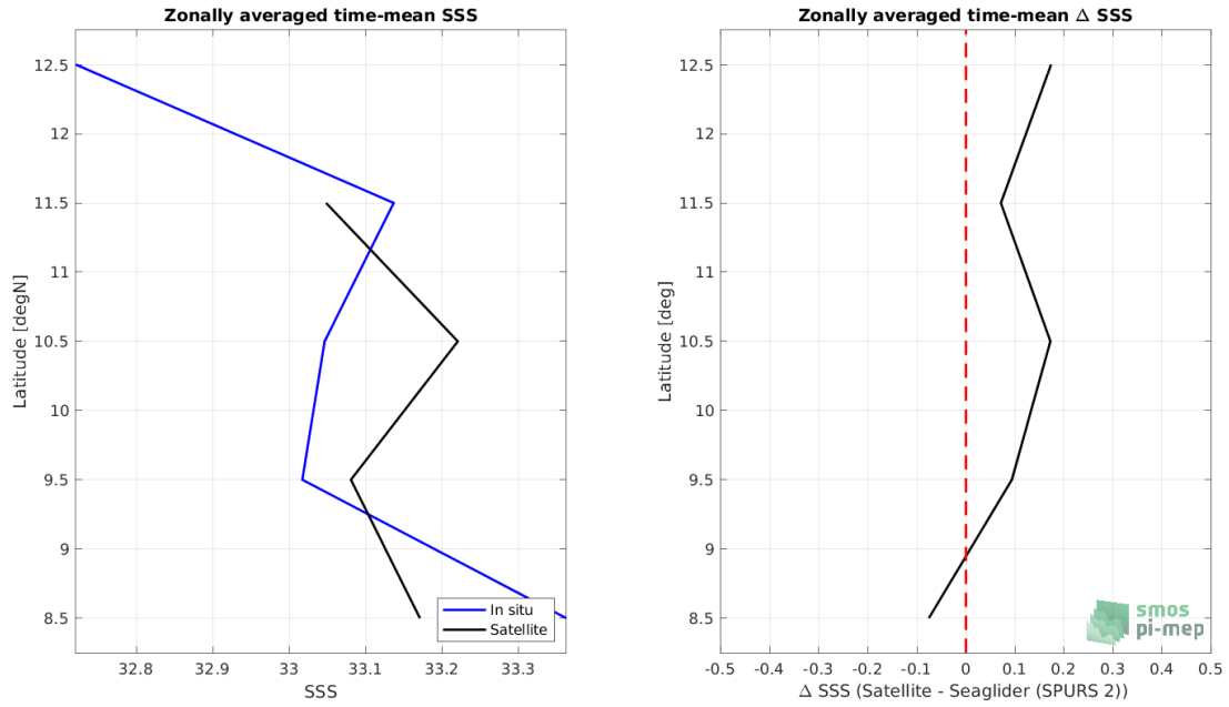
Figure 8: Left panel: Zonal mean SSS from SMOS SSS L3 v8 - 18 Days (CATDS-CECOS-LOCEAN) satellite product (black) and from Seaglider (SPURS 2) (blue). Right panel: Zonal mean of \Delta SSS (Satellite - Seaglider (SPURS 2)) for all the collected Pi-MEP match-up pairs estimated over the full satellite product period.
