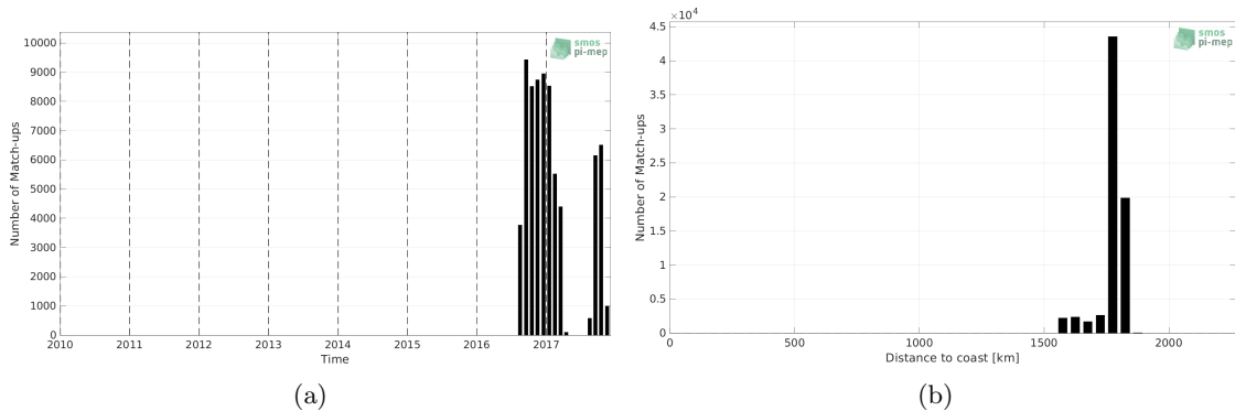
Figure 1: Number of match-ups between Seaglider (SPURS 2) and SMOS SSS L3 v8 - 18 Days (CATDS-CECOS-LOCEAN) SSS as a function of time (a) and as function of the distance to coast (b) over the SPURS 2 Pi-MEP region and for the full satellite product period.
