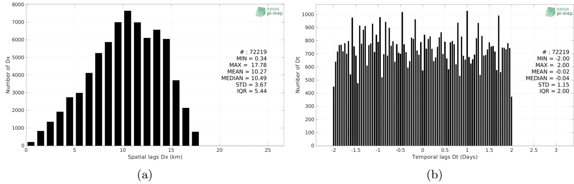
Figure 5: Histograms of the spatial (a) and temporal (b) lags between the location/time of the Seaglider (SPURS 2) measurement and the date of the corresponding SMOS SSS L3 v8 - 18 Days (CATDS-CECOS-LOCEAN) SSS pixel.
