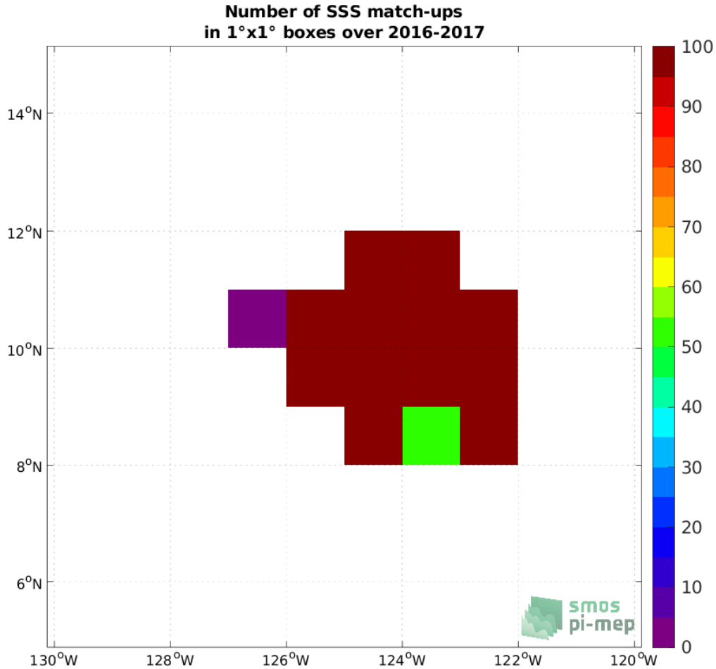
Figure 4: Number of SSS match-ups between Seaglider (SPURS 2) SSS and the SMOS SSS L3 v8 - 18 Days (CATDS-CECOS-LOCEAN) SSS product for the SPURS 2 Pi-MEP region over 1^\circ \times 1^\circ boxes and for the full satellite product period.
