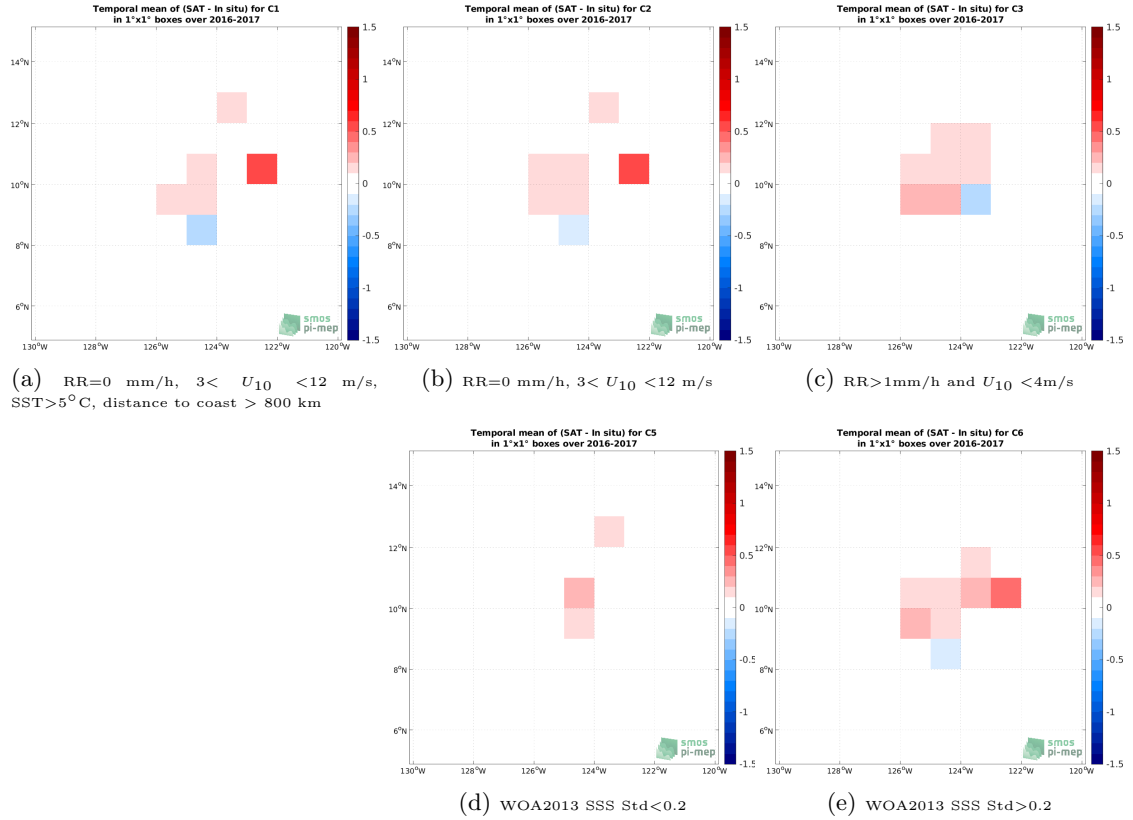
Figure 12: Temporal mean gridded over spatial boxes of size 1^{\circ}\times 1^{\circ} of \Delta\text{SSS} (SMOS SSS L3 v8 - 18 Days (CATDS-CECOS-LOCEAN) - Seaglider (SPURS 2)) for 5 different subdatasets corresponding to:RR=0 mm/h, 3 < U_{10} < 12 m/s, SST > 5^{\circ}\text{C} , distance to coast > 800 km (a), RR=0 mm/h, 3 < U_{10} < 12 m/s (b), RR > 1 mm/h and U_{10} < 4 m/s (c), WOA2013 SSS Std < 0.2 (d), WOA2013 SSS Std > 0.2 (e).
