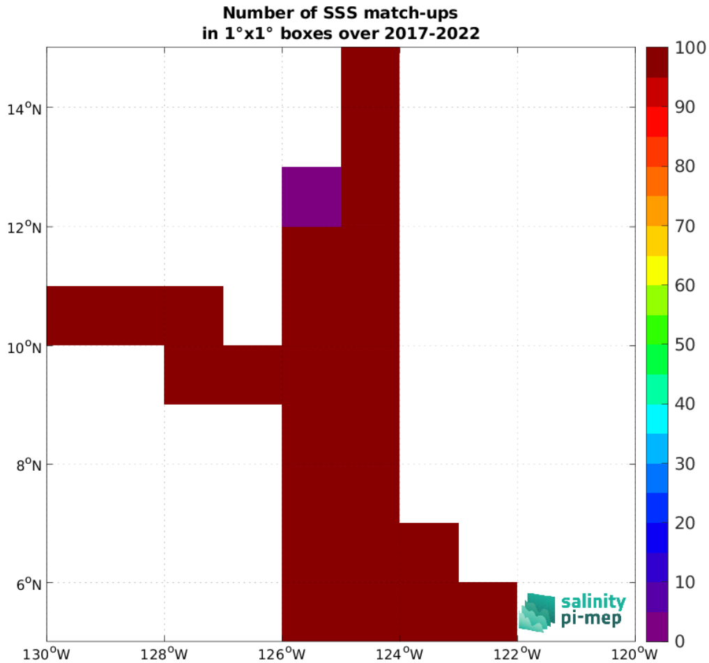
Figure 4: Number of SSS match-ups between Saildrone SSS and the SMOS SSS L3 v8 - 18 Days (CATDS-CEC-LOCEAN) SSS product for the SPURS 2 Pi-MEP region over 1^\circ \times 1^\circ boxes and for the full satellite product period.
