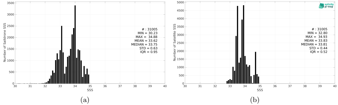
Figure 2: Histograms of SSS from Saildrone (a) and SMOS SSS L3 v8 - 18 Days (CATDS-CEC-LOCEAN) (b) considering all match-up pairs per bins of 0.1 over the SPURS 2 Pi-MEP region and for the full satellite product period.
