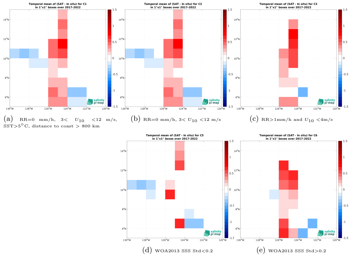
Figure 12: Temporal mean gridded over spatial boxes of size 1^\circ \times 1^\circ of \Delta SSS (SMOS SSS L3 v8 - 18 Days (CATDS-CEC-LOCEAN) - Sairdrone) for 5 different subdatasets corresponding to:RR=0 mm/h, 3 < U_{10} < 12 m/s, SST >5^\circ\text{C} , distance to coast > 800 km (a), RR=0 mm/h, 3 < U_{10} < 12 m/s (b), RR >1 mm/h and U_{10} < 4 m/s (c), WOA2013 SSS Std <0.2 (d), WOA2013 SSS Std >0.2 (e).
