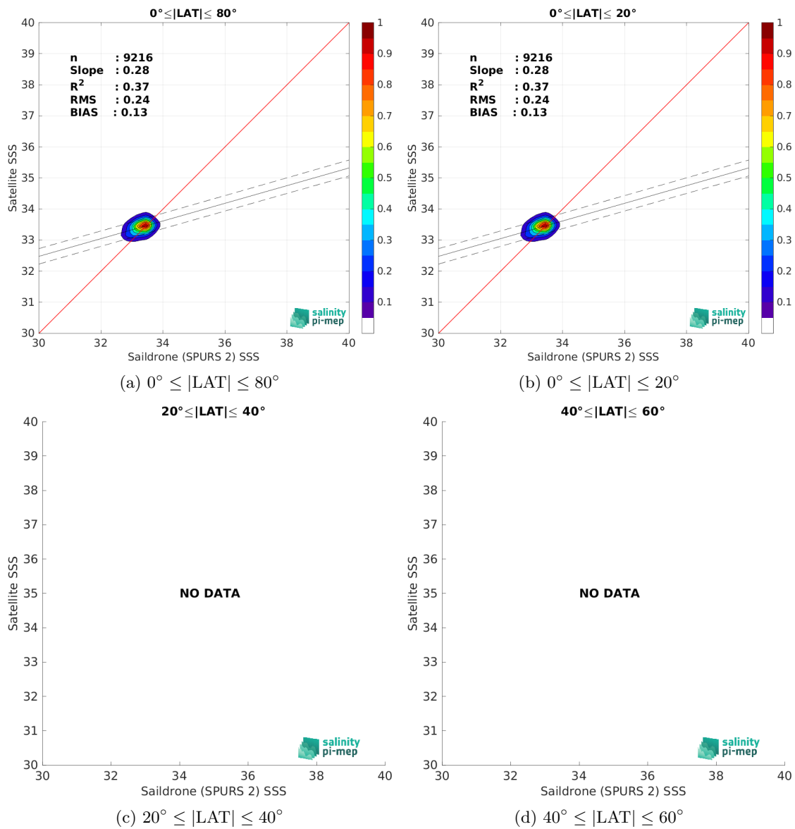
Figure 9: Contour maps of the concentration of SMOS SSS L3 v8 - 18 Days (CATDS-CEC-LOCEAN) SSS (y-axis) versus Saildrone (SPURS 2) SSS (x-axis) at match-up pairs for different latitude bands. For each plot, the red line shows x=y . The black thin and dashed lines indicate a linear fit through the data cloud and the \pm 95\% confidence levels, respectively. The number match-up pairs n , the slope and R^2 coefficient of the linear fit, the root mean square (RMS) and the mean bias between satellite and in situ data are indicated for each latitude band in each plots.
