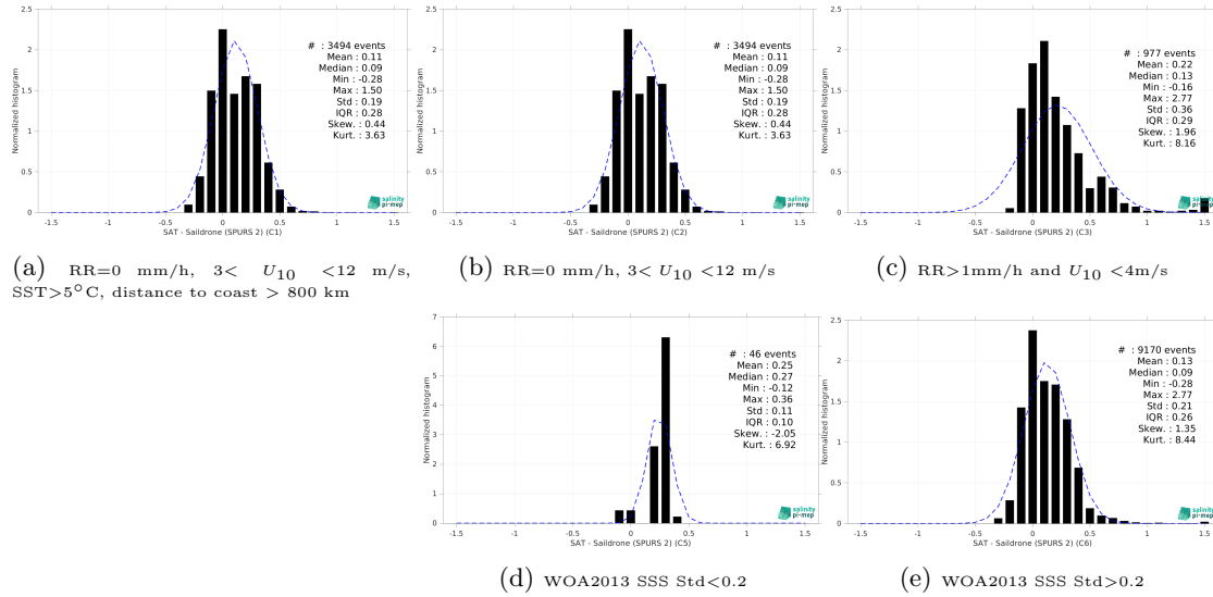
Figure 13: Normalized histogram of \Delta SSS (SMOS SSS L3 v8 - 18 Days (CATDS-CEC-LOCEAN) - Saildrone (SPURS 2)) for 5 different subdatasets corresponding to: RR=0 mm/h, 3 < U_{10} < 12 m/s, SST > 5°C, distance to coast > 800 km (a), RR=0 mm/h, 3 < U_{10} < 12 m/s (b), RR > 1mm/h and U_{10} < 4 m/s (c), WOA2013 SSS Std < 0.2 (d), WOA2013 SSS Std > 0.2 (e).
