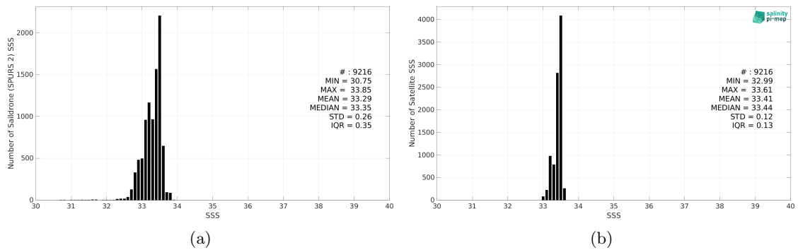
Figure 2: Histograms of SSS from Saildrone (SPURS 2) (a) and SMOS SSS L3 v8 - 18 Days (CATDS-CEC-LOCEAN) (b) considering all match-up pairs per bins of 0.1 over the SPURS 2 Pi-MEP region and for the full satellite product period.
