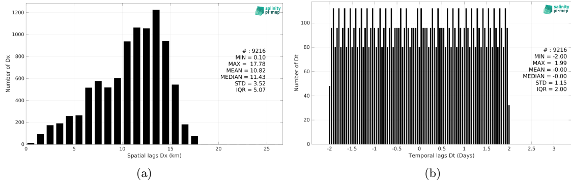
Figure 5: Histograms of the spatial (a) and temporal (b) lags between the location/time of the Saildrone (SPURS 2) measurement and the date of the corresponding SMOS SSS L3 v8 - 18 Days (CATDS-CEC-LOCEAN) SSS pixel.
