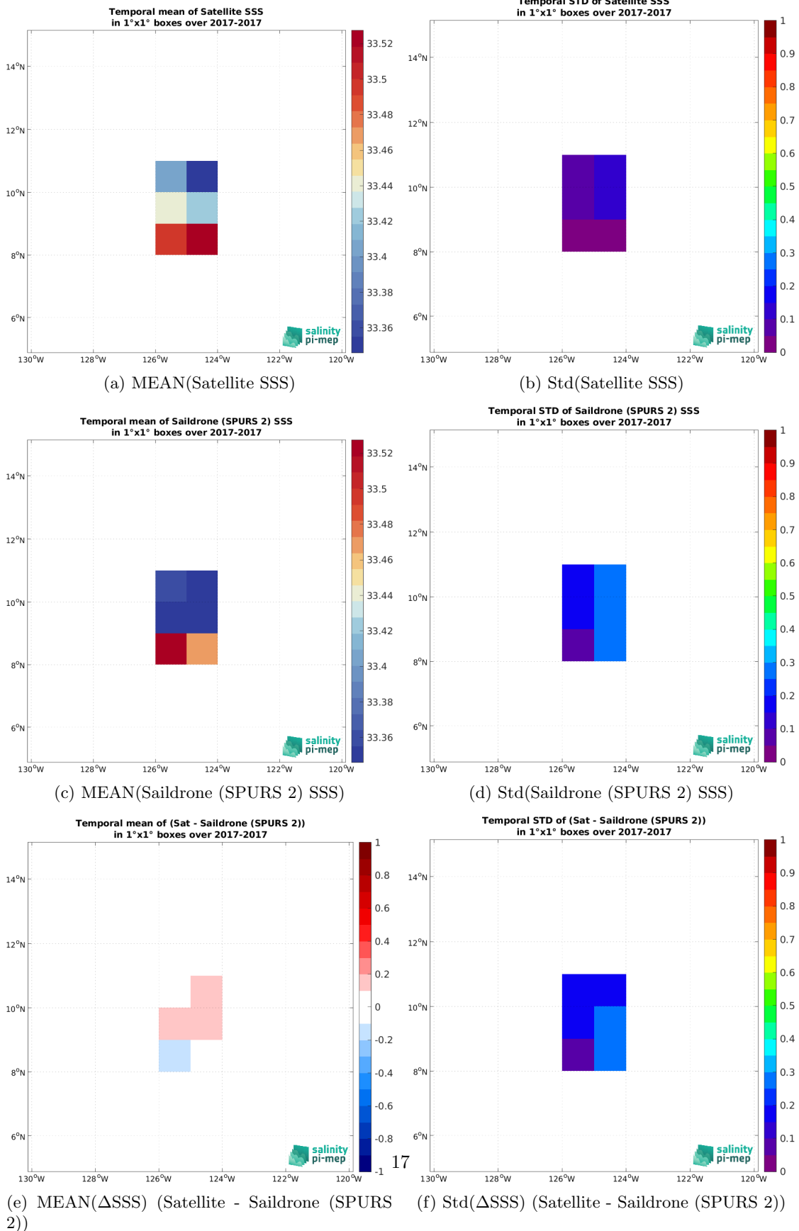
Figure 6: Temporal mean (left) and Std (right) of SSS from SMOS SSS L3 v8 - 18 Days (CATDS-CEC-LOCEAN) (top), Saildrone (SPURS 2) (middle), and of \Delta SSS (Satellite - Saildrone (SPURS 2)). Only match-up pairs are used to generate these maps.
