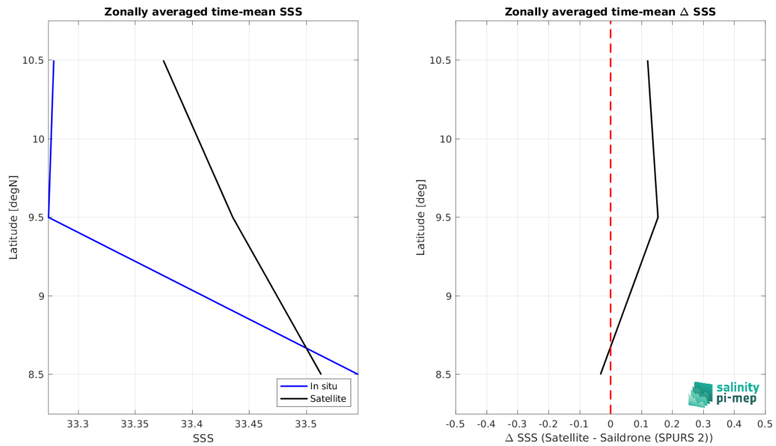
Figure 8: Left panel: Zonal mean SSS from SMOS SSS L3 v8 - 18 Days (CATDS-CEC-LOCEAN) satellite product (black) and from Sairdron (SPURS 2) (blue). Right panel: Zonal mean of \Delta SSS (Satellite - Sairdron (SPURS 2)) for all the collected Pi-MEP match-up pairs estimated over the full satellite product period.
