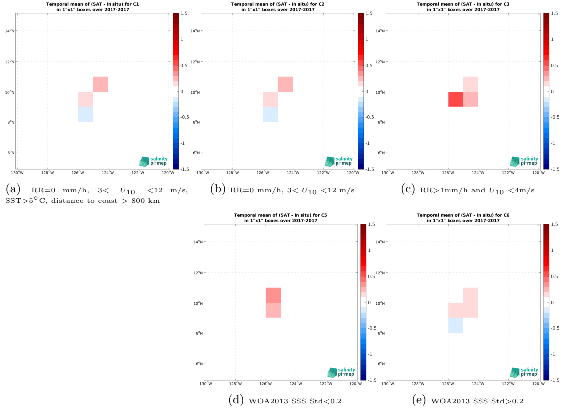
Figure 12: Temporal mean gridded over spatial boxes of size 1^{\circ}\times 1^{\circ} of \Delta\text{SSS} (SMOS SSS L3 v8 - 18 Days (CATDS-CEC-LOCEAN) - Saifdrone (SPURS 2)) for 5 different subdatasets corresponding to:RR=0 mm/h, 3 < U_{10} < 12 m/s, SST >5^{\circ}\text{C} , distance to coast > 800 km (a), RR=0 mm/h, 3 < U_{10} < 12 m/s (b), RR >1 mm/h and U_{10} < 4 m/s (c), WOA2013 SSS Std <0.2 (d), WOA2013 SSS Std >0.2 (e).
