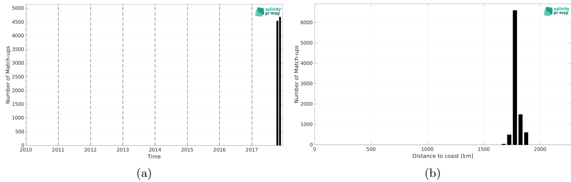
Figure 1: Number of match-ups between Saildrone (SPURS 2) and SMOS SSS L3 v8 - 18 Days (CATDS-CEC-LOCEAN) SSS as a function of time (a) and as function of the distance to coast (b) over the SPURS 2 Pi-MEP region and for the full satellite product period.
