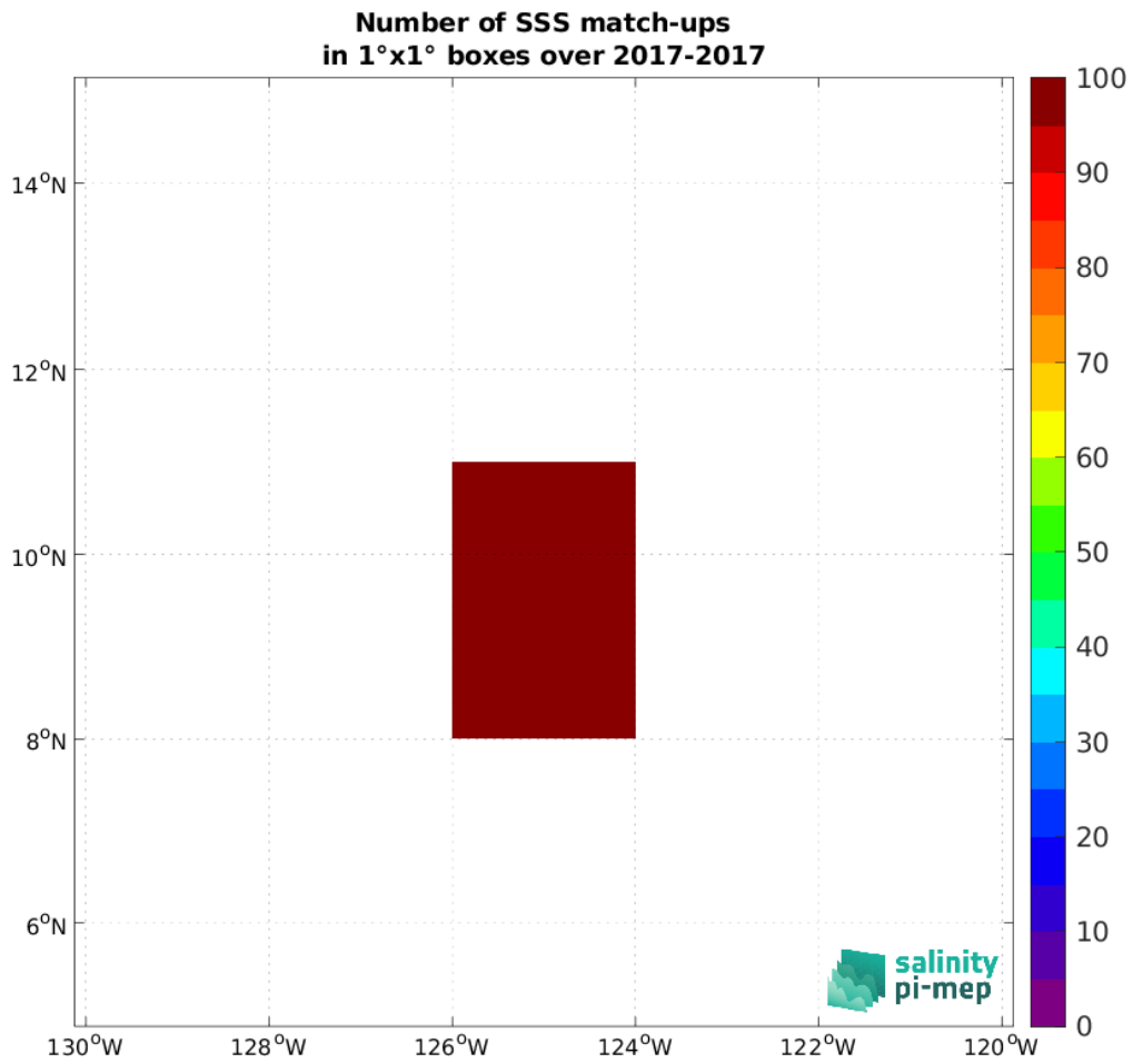
Figure 4: Number of SSS match-ups between Saildrone (SPURS 2) SSS and the SMOS SSS L3 v8 - 18 Days (CATDS-CEC-LOCEAN) SSS product for the SPURS 2 Pi-MEP region over 1°x1° boxes and for the full satellite product period.
