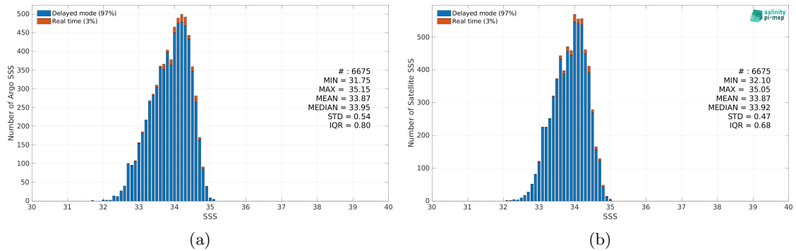
Figure 2: Histograms of SSS from Argo (a) and SMOS SSS L3 v8 - 18 Days (CATDS-CEC-LOCEAN) (b) considering all match-up pairs per bins of 0.1 over the SPURS 2 Pi-MEP region and for the full satellite product period.
