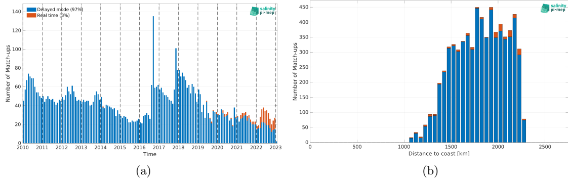
Figure 1: Number of match-ups between Argo and SMOS SSS L3 v8 - 18 Days (CATDS-CEC-LOCEAN) SSS as a function of time (a) and as function of the distance to coast (b) over the SPURS 2 Pi-MEP region and for the full satellite product period.
