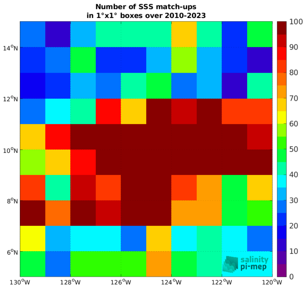
Figure 4: Number of SSS match-ups between Argo SSS and the SMOS SSS L3 v8 - 18 Days (CATDS-CEC-LOCEAN) SSS product for the SPURS 2 Pi-MEP region over 1°x1° boxes and for the full satellite product period.
