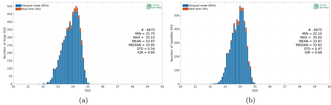
Figure 2: Histograms of SSS from Argo (a) and SMOS SSS L3 v8 - 18 Days (CATDS-CECOS-LOCEAN) (b) considering all match-up pairs per bins of 0.1 over the SPURS 2 Pi-MEP region and for the full satellite product period.
