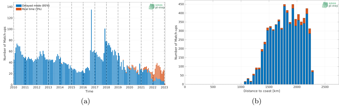
Figure 1: Number of match-ups between Argo and SMOS SSS L3 v8 - 18 Days (CATDS-CECOS-LOCEAN) SSS as a function of time (a) and as function of the distance to coast (b) over the SPURS 2 Pi-MEP region and for the full satellite product period.
