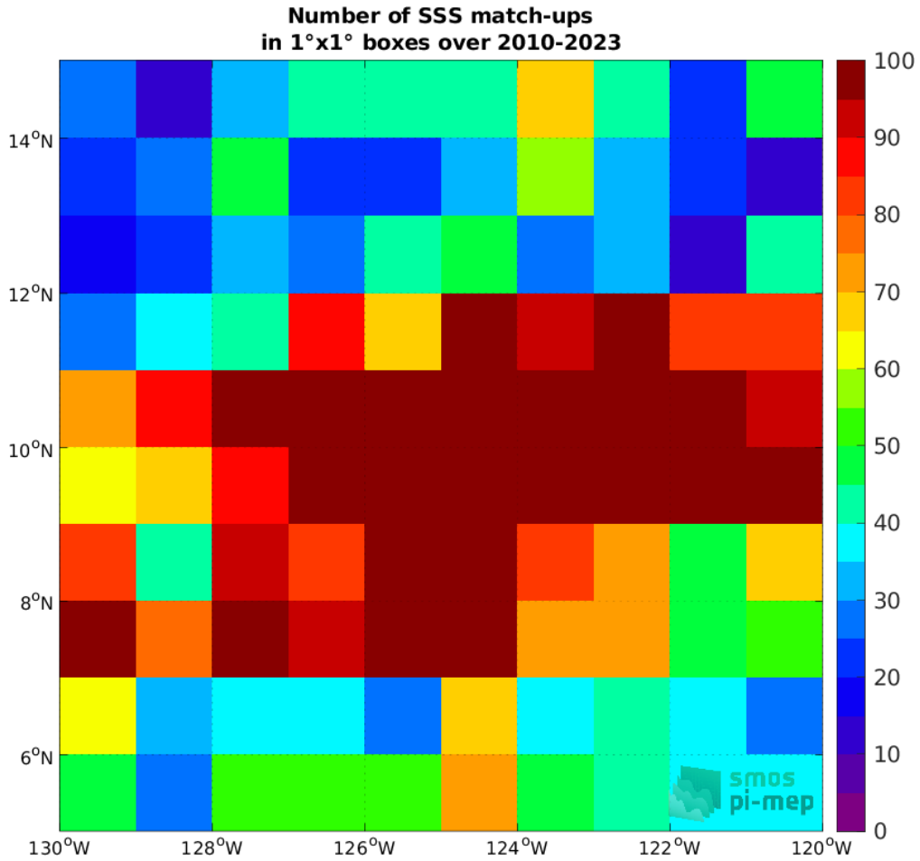
Figure 4: Number of SSS match-ups between Argo SSS and the SMOS SSS L3 v8 - 18 Days (CATDS-CECOS-LOCEAN) SSS product for the SPURS 2 Pi-MEP region over 1°x1° boxes and for the full satellite product period.
