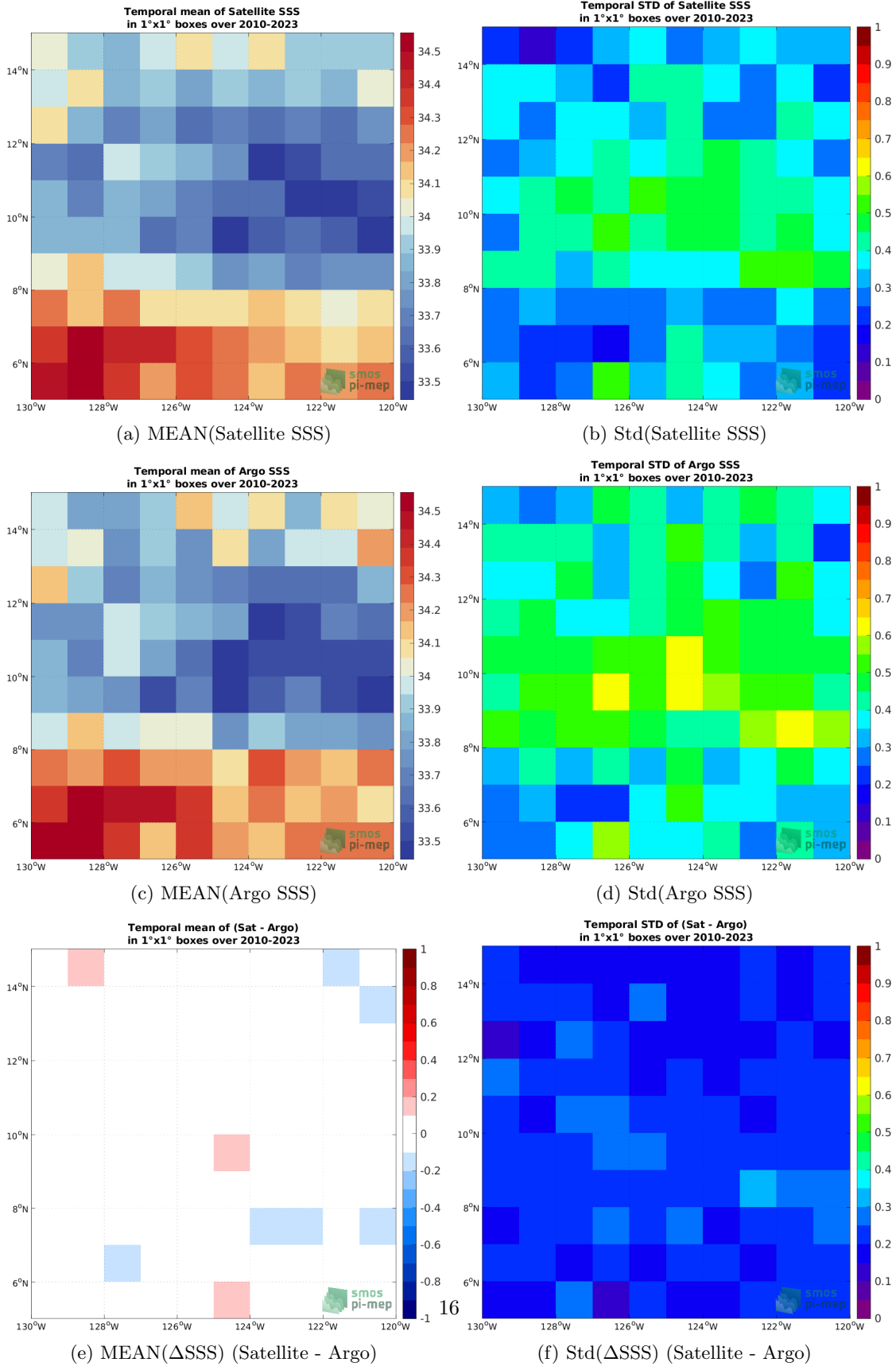
Figure 6: Temporal mean (left) and Std (right) of SSS from SMOS SSS L3 v8 - 18 Days (CATDS-CECOS-LOCEAN) (top), Argo (middle), and of \Delta SSS (Satellite - Argo). Only match-up pairs are used to generate these maps.
