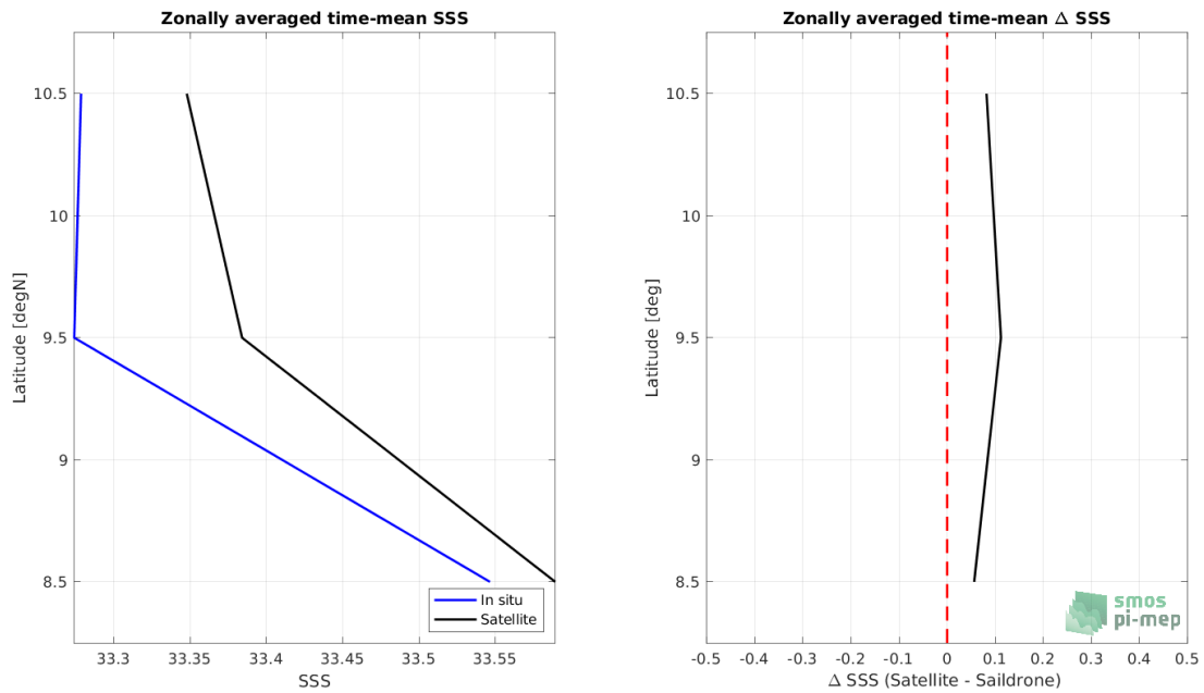
Figure 7: Left panel: Zonal mean SSS from SMOS SSS L3 v7 - 18 Days (CATDS-CECOS-LOCEAN) satellite product (black) and from Sairdrone (blue). Right panel: Zonal mean of \Delta SSS (Satellite - Sairdrone) for all the collected Pi-MEP match-up pairs estimated over the full satellite product period.
