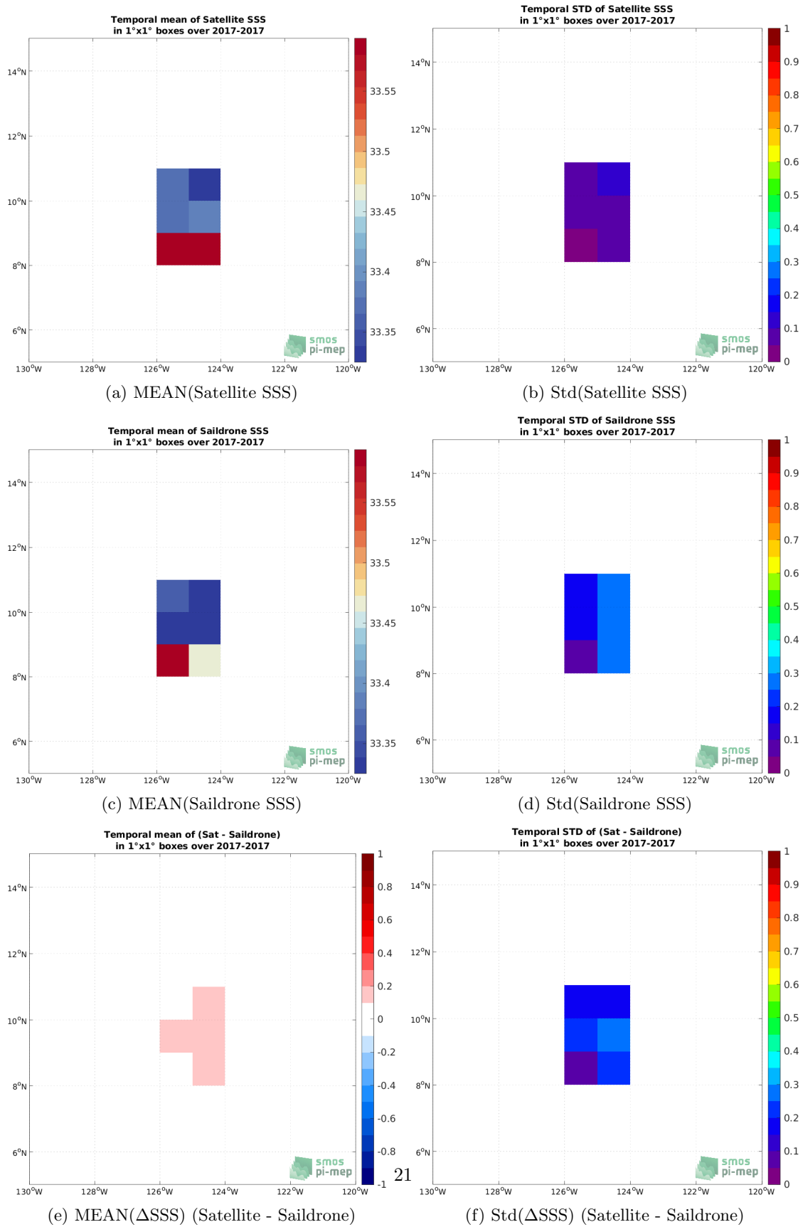
Figure 5: Temporal mean (left) and Std (right) of SSS from SMOS SSS L3 v7 - 18 Days (CATDS-CECOS-LOCEAN) (top), Saildrone (middle), and of \Delta SSS (Satellite - Saildrone). Only match-pairs are used to generate these maps.
