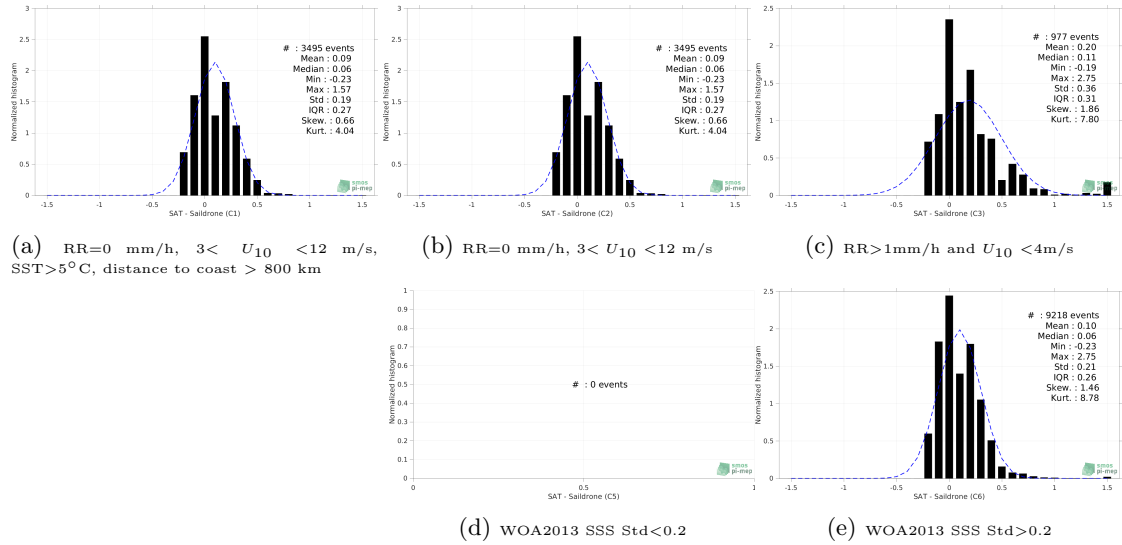
Figure 12: Normalized histogram of \Delta SSS (SMOS SSS L3 v7 - 18 Days (CATDS-CECOS-LOCEAN) - Saildrone) for 5 different subdatasets corresponding to: RR=0 mm/h, 3 < U_{10} < 12 m/s, SST > 5°C, distance to coast > 800 km (a), RR=0 mm/h, 3 < U_{10} < 12 m/s (b), RR > 1mm/h and U_{10} < 4 m/s (c), WOA2013 SSS Std < 0.2 (d), WOA2013 SSS Std > 0.2 (e).
