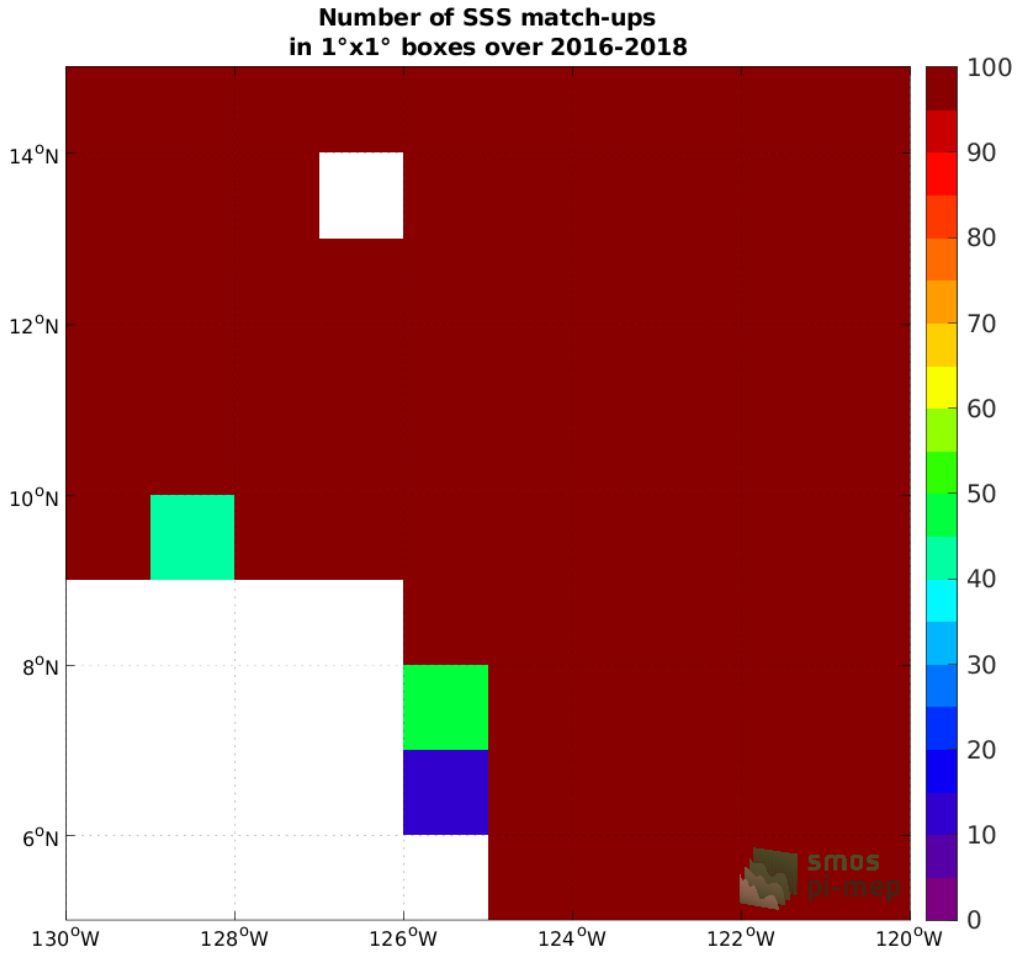
Figure 3: Number of SSS match-ups between Surface drifters SSS and the SMOS SSS L3 v7 - 18 Days (CATDS-CECOS-LOCEAN) SSS product for the SPURS 2 Pi-MEP region over 1°x1° boxes and for the full satellite product period.
