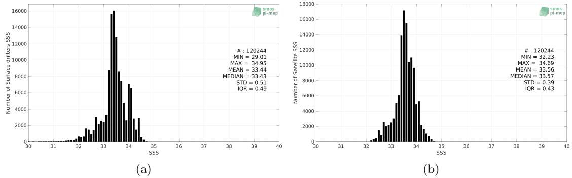
Figure 2: Histograms of SSS from Surface drifters (a) and SMOS SSS L3 v7 - 18 Days (CATDS-CECOS-LOCEAN) (b) considering all match-up pairs per bins of 0.1 over the SPURS 2 Pi-MEP region and for the full satellite product period.
