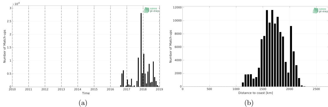
Figure 1: Number of match-ups between Surface drifters and SMOS SSS L3 v7 - 18 Days (CATDS-CECOS-LOCEAN) SSS as a function of time (a) and as function of the distance to coast (b) over the SPURS 2 Pi-MEP region and for the full satellite product period.
