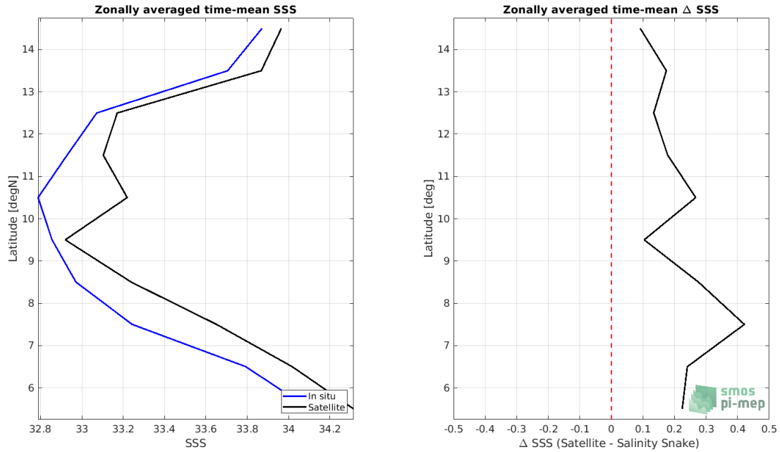
Figure 7: Left panel: Zonal mean SSS from SMOS SSS L3 v5 - 18 Days (CATDS-CECOS-LOCEAN) satellite product (black) and from Salinity Snake (blue). Right panel: Zonal mean of \Delta SSS (Satellite - Salinity Snake) for all the collected Pi-MEP match-up pairs estimated over the full satellite product period.
