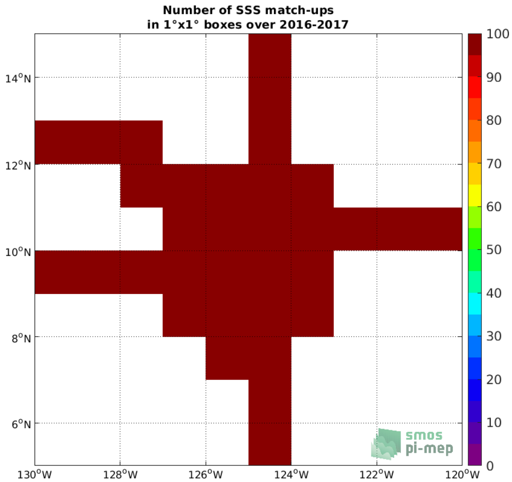
Figure 3: Number of SSS match-ups between Salinity Snake SSS and the SMOS SSS L3 v5 - 18 Days (CATDS-CECOS-LOCEAN) SSS product for the SPURS 2 Pi-MEP region over 1°x1° boxes and for the full satellite product period.
