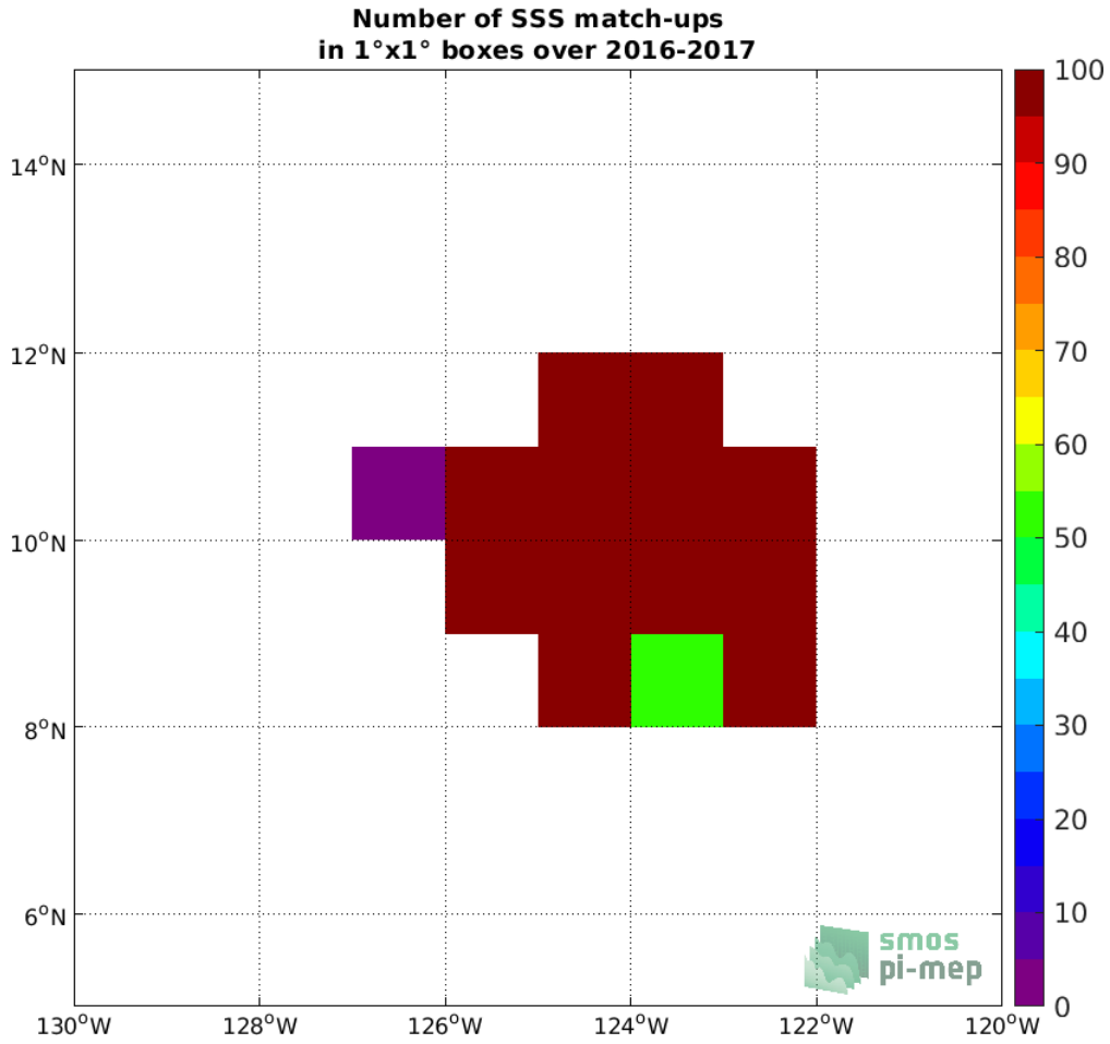
Figure 3: Number of SSS match-ups between Seaglider SSS and the SMOS SSS L3 v5 - 18 Days (CATDS-CECOS-LOCEAN) SSS product for the SPURS 2 Pi-MEP region over 1°x1° boxes and for the full satellite product period.
