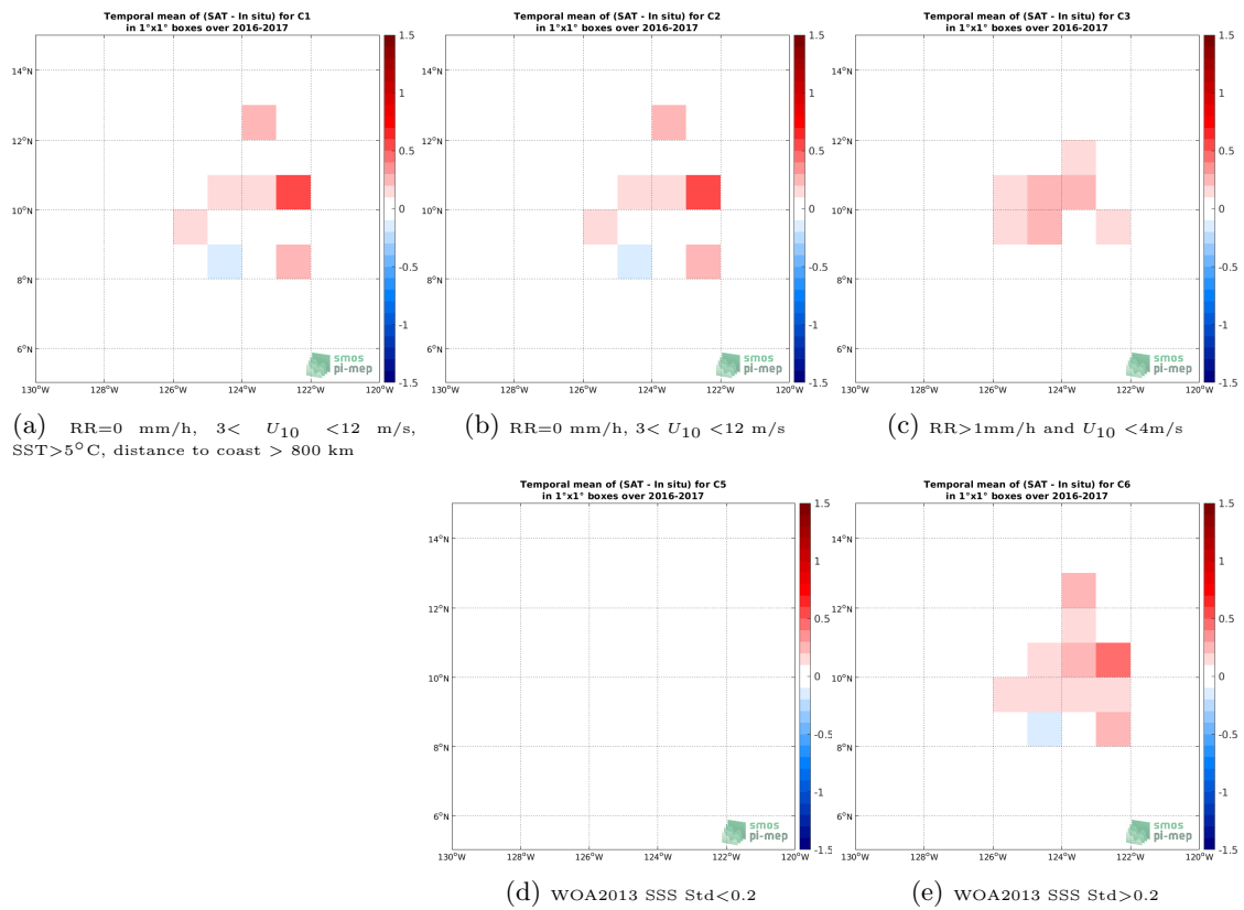
Figure 11: Temporal mean gridded over spatial boxes of size 1^\circ \times 1^\circ of \Delta SSS (SMOS SSS L3 v5 - 18 Days (CATDS-CECOS-LOCEAN) - Seaglider) for 5 different subdatasets corresponding to:RR=0 mm/h, 3 < U_{10} < 12 m/s, SST >5^\circ C, distance to coast > 800 km (a), RR=0 mm/h, 3 < U_{10} < 12 m/s (b), RR >1 mm/h and U_{10} < 4 m/s (c), WOA2013 SSS Std <0.2 (d), WOA2013 SSS Std >0.2 (e).
