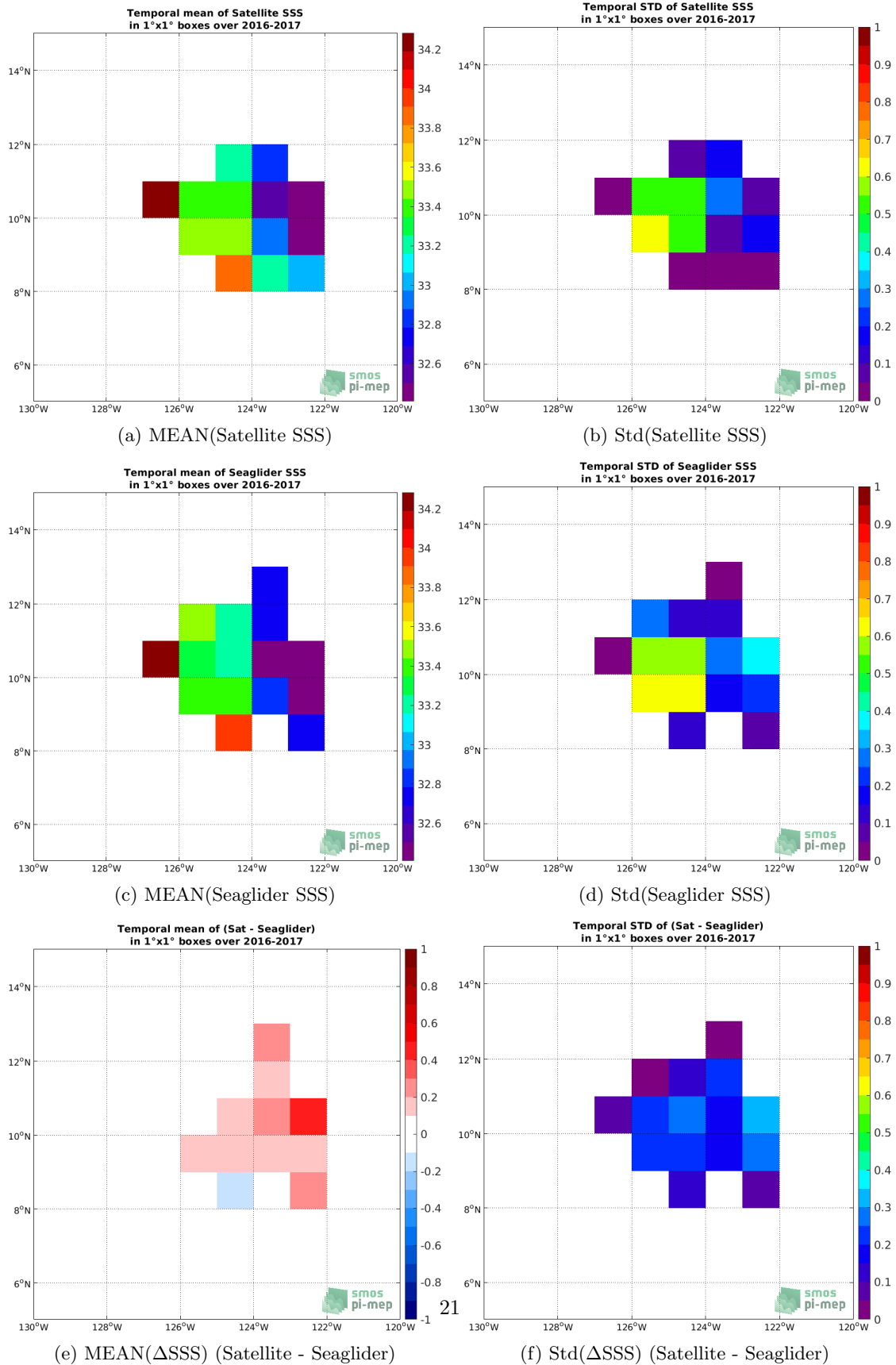
Figure 5: Temporal mean (left) and Std (right) of SSS from SMOS SSS L3 v5 - 18 Days (CATDS-CECOS-LOCEAN) (top), Seaglider (middle), and of \Delta SSS (Satellite - Seaglider). Only match-up pairs are used to generate these maps.
