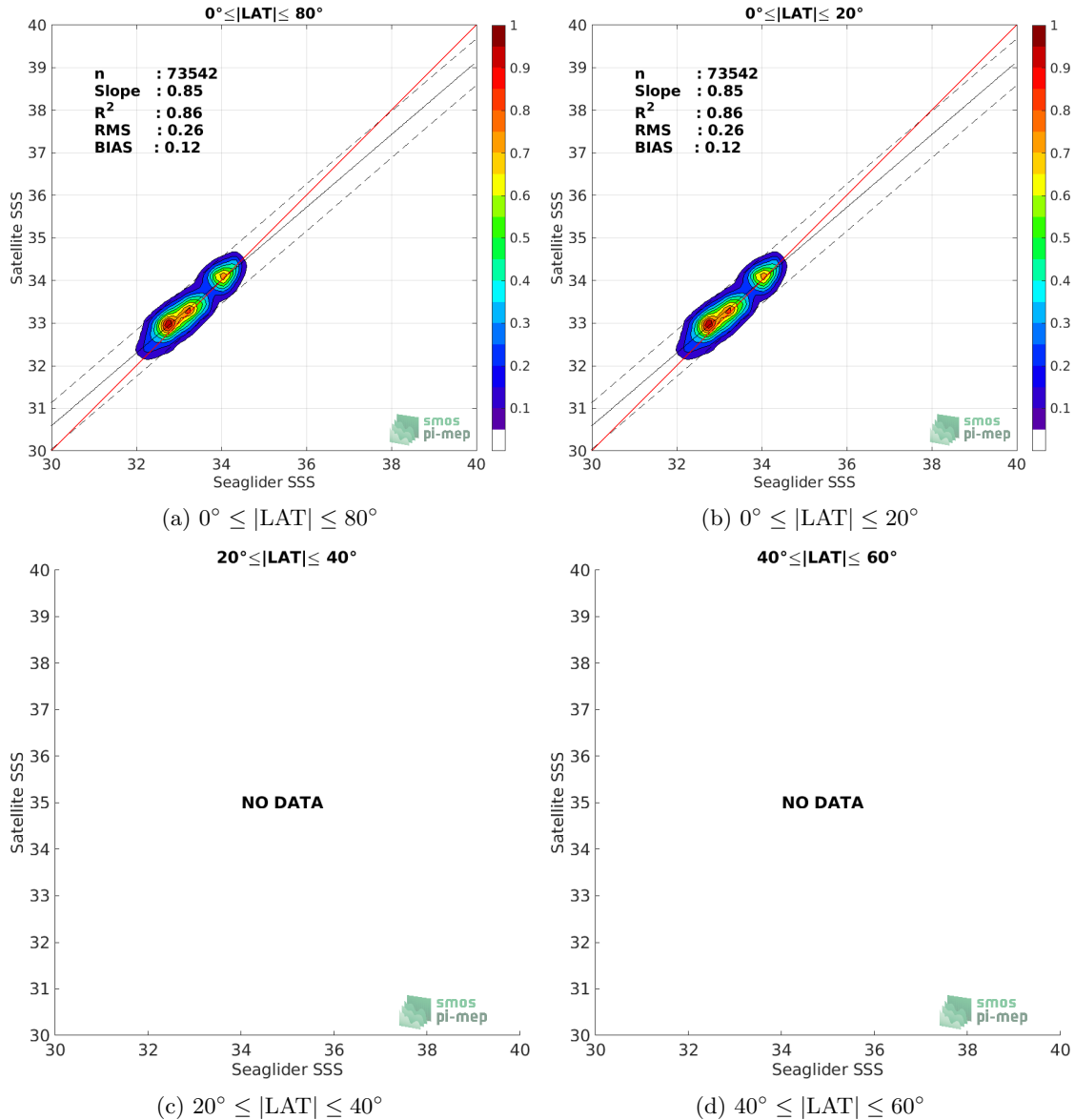
Figure 8: Contour maps of the concentration of SMOS SSS L3 v5 - 18 Days (CATDS-CECOS-LOCEAN) SSS (y-axis) versus Seaglider SSS (x-axis) at match-up pairs for different latitude bands. For each plot, the red line shows x=y . The black thin and dashed lines indicate a linear fit through the data cloud and the \pm 95\% confidence levels, respectively. The number match-up pairs n , the slope and R^2 coefficient of the linear fit, the root mean square (RMS) and the mean bias between satellite and in situ data are indicated for each latitude band in each plots.
