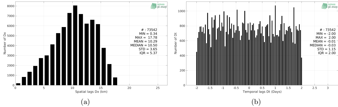
Figure 4: Histograms of the spatial (a) and temporal (b) lags between the location/time of the Seaglider measurement and the date of the corresponding SMOS SSS L3 v5 - 18 Days (CATDS-CECOS-LOCEAN) SSS pixel.
