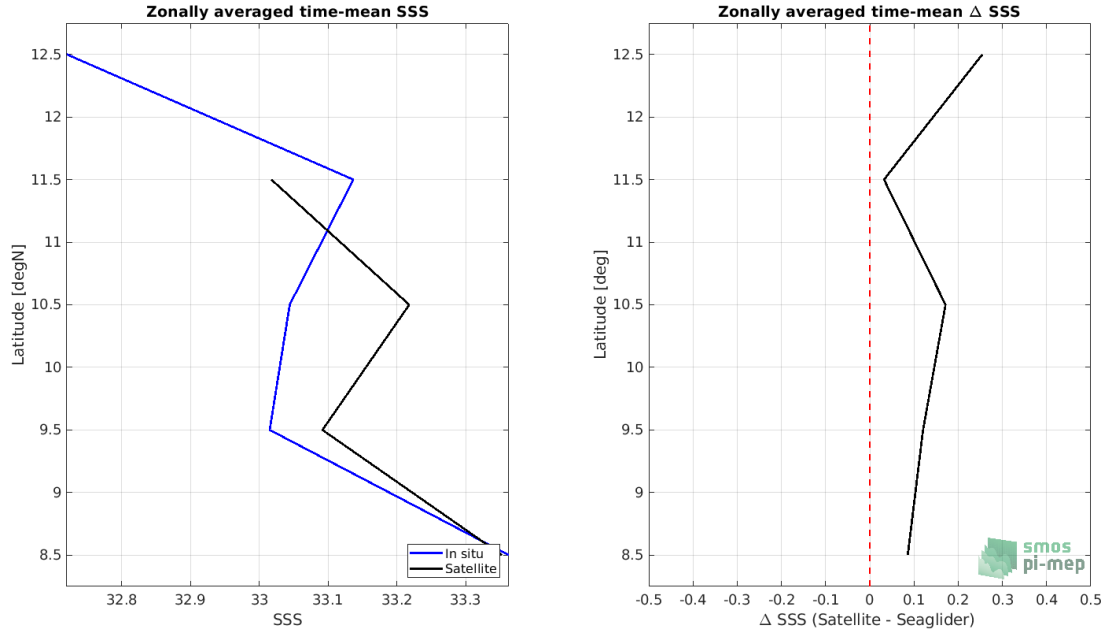
Figure 7: Left panel: Zonal mean SSS from SMOS SSS L3 v5 - 18 Days (CATDS-CECOS-LOCEAN) satellite product (black) and from Seaglider (blue). Right panel: Zonal mean of \Delta SSS (Satellite - Seaglider) for all the collected Pi-MEP match-up pairs estimated over the full satellite product period.
