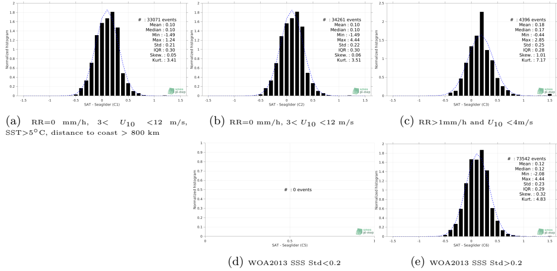
Figure 12: Normalized histogram of \Delta SSS (SMOS SSS L3 v5 - 18 Days (CATDS-CECOS-LOCEAN) - Seaglider) for 5 different subdatasets corresponding to: RR=0 mm/h, 3 < U_{10} < 12 m/s, SST>5°C, distance to coast > 800 km (a), RR=0 mm/h, 3 < U_{10} < 12 m/s (b), RR>1mm/h and U_{10} < 4 m/s (c), WOA2013 SSS Std<0.2 (d), WOA2013 SSS Std>0.2 (e).
