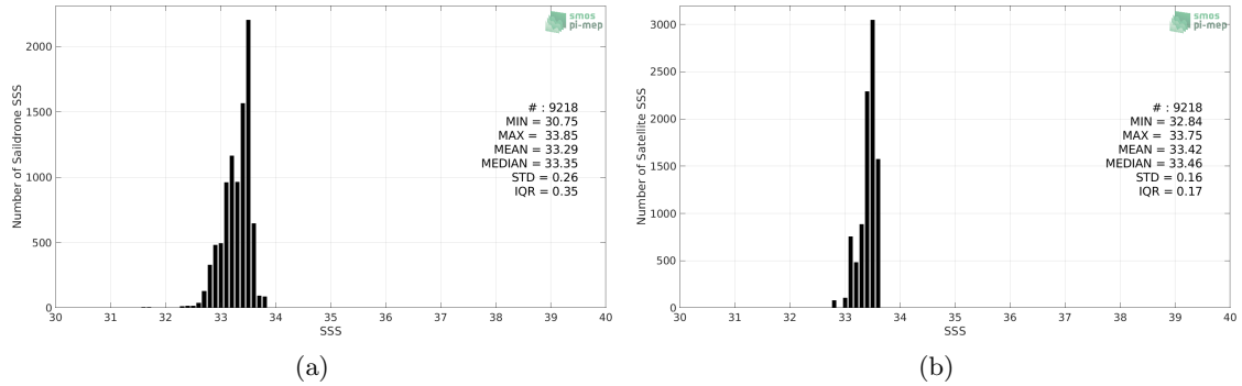
Figure 2: Histograms of SSS from Sairdrone (a) and SMOS SSS L3 v5 - 18 Days (CATDS-CECOS-LOCEAN) (b) considering all match-up pairs per bins of 0.1 over the SPURS 2 Pi-MEP region and for the full satellite product period.
