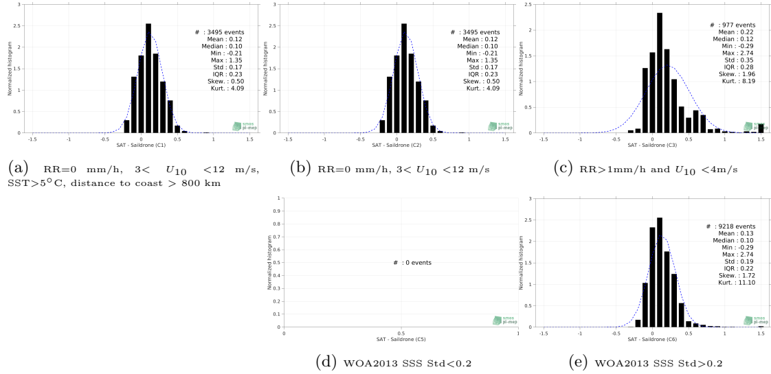
Figure 12: Normalized histogram of \Delta SSS (SMOS SSS L3 v5 - 18 Days (CATDS-CECOS-LOCEAN) - Saildrone) for 5 different subdatasets corresponding to: RR=0 mm/h, 3 < U_{10} < 12 m/s, SST > 5°C, distance to coast > 800 km (a), RR=0 mm/h, 3 < U_{10} < 12 m/s (b), RR > 1mm/h and U_{10} < 4 m/s (c), WOA2013 SSS Std < 0.2 (d), WOA2013 SSS Std > 0.2 (e).
