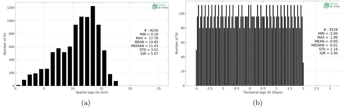
Figure 4: Histograms of the spatial (a) and temporal (b) lags between the location/time of the Saildrone measurement and the date of the corresponding SMOS SSS L3 v5 - 18 Days (CATDS-CECOS-LOCEAN) SSS pixel.
