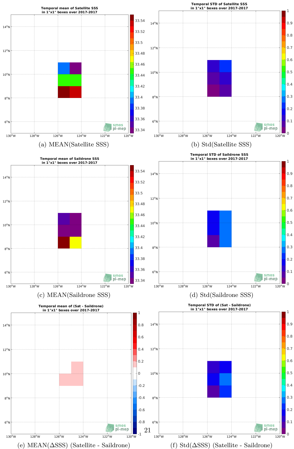
Figure 5: Temporal mean (left) and Std (right) of SSS from SMOS SSS L3 v5 - 18 Days (CATDS-CECOS-LOCEAN) (top), Saildrone (middle), and of \Delta SSS (Satellite - Saildrone). Only match-up pairs are used to generate these maps.
