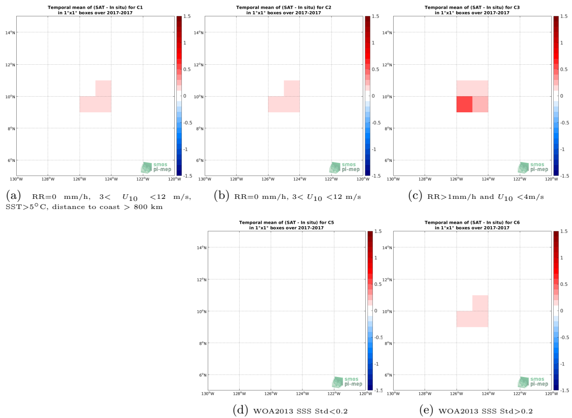
Figure 11: Temporal mean gridded over spatial boxes of size 1^\circ \times 1^\circ of \Delta SSS (SMOS SSS L3 v5 - 18 Days (CATDS-CECOS-LOCEAN) - Saildrone) for 5 different subdatasets corresponding to:RR=0 mm/h, 3 < U_{10} < 12 m/s, SST >5^\circ C, distance to coast > 800 km (a), RR=0 mm/h, 3 < U_{10} < 12 m/s (b), RR >1 mm/h and U_{10} < 4 m/s (c), WOA2013 SSS Std <0.2 (d), WOA2013 SSS Std >0.2 (e).
