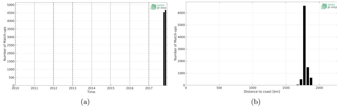
Figure 1: Number of match-ups between Saildrone and SMOS SSS L3 v5 - 18 Days (CATDS-CECOS-LOCEAN) SSS as a function of time (a) and as function of the distance to coast (b) over the SPURS 2 Pi-MEP region and for the full satellite product period.
