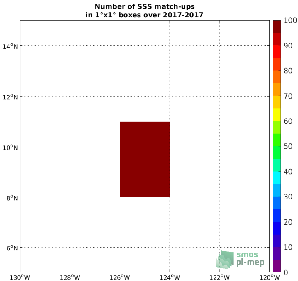
Figure 3: Number of SSS match-ups between Sairdrone SSS and the SMOS SSS L3 v5 - 18 Days (CATDS-CECOS-LOCEAN) SSS product for the SPURS 2 Pi-MEP region over 1°x1° boxes and for the full satellite product period.
