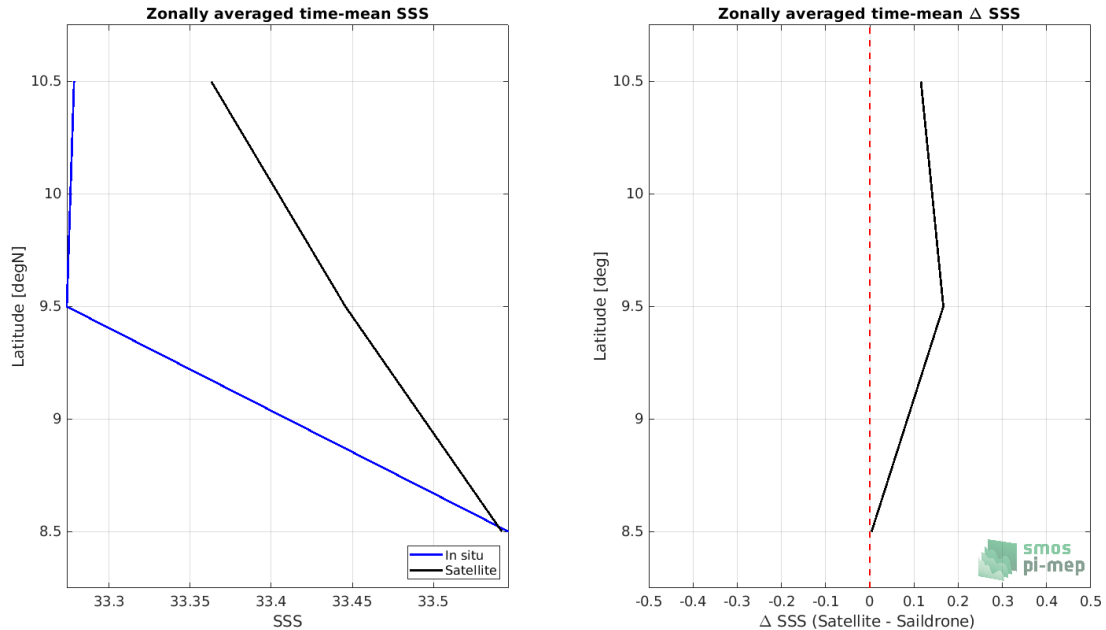
Figure 7: Left panel: Zonal mean SSS from SMOS SSS L3 v5 - 18 Days (CATDS-CECOS-LOCEAN) satellite product (black) and from Sairdrone (blue). Right panel: Zonal mean of \Delta SSS (Satellite - Sairdrone) for all the collected Pi-MEP match-up pairs estimated over the full satellite product period.
