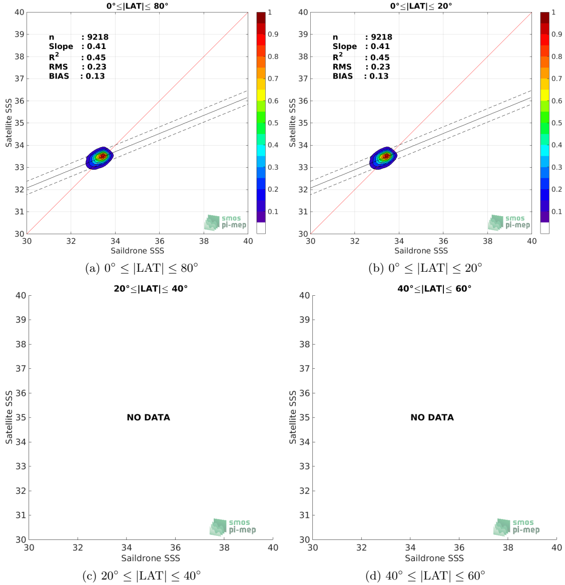
Figure 9: Contour maps of the concentration of SMOS SSS L3 v5 - 18 Days (CATDS-CECOS-LOCEAN) SSS (y-axis) versus Saildrone SSS (x-axis) at match-up pairs for different latitude bands. For each plot, the red line shows x=y . The black thin and dashed lines indicate a linear fit through the data cloud and the \pm 95\% confidence levels, respectively. The number match-up pairs n , the slope and R^2 coefficient of the linear fit, the root mean square (RMS) and the mean bias between satellite and in situ data are indicated for each latitude band in each plots.
