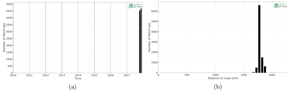
Figure 1: Number of match-ups between Sairdrone and SMOS SSS L3 v5 - 18 Days (CATDS-CECOS-LOCEAN) SSS as a function of time (a) and as function of the distance to coast (b) over the SPURS 2 Pi-MEP region and for the full satellite product period.
