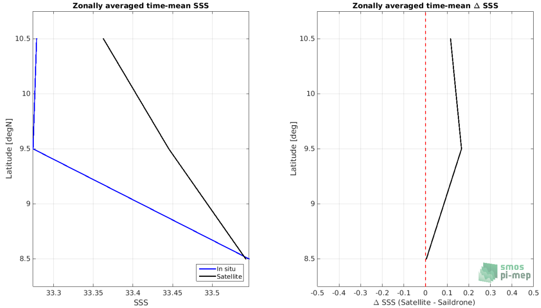
Figure 8: Left panel: Zonal mean SSS from SMOS SSS L3 v5 - 18 Days (CATDS-CECOS-LOCEAN) satellite product (black) and from Sairdrone (blue). Right panel: Zonal mean of \Delta SSS (Satellite - Sairdrone) for all the collected Pi-MEP match-up pairs estimated over the full satellite product period.
