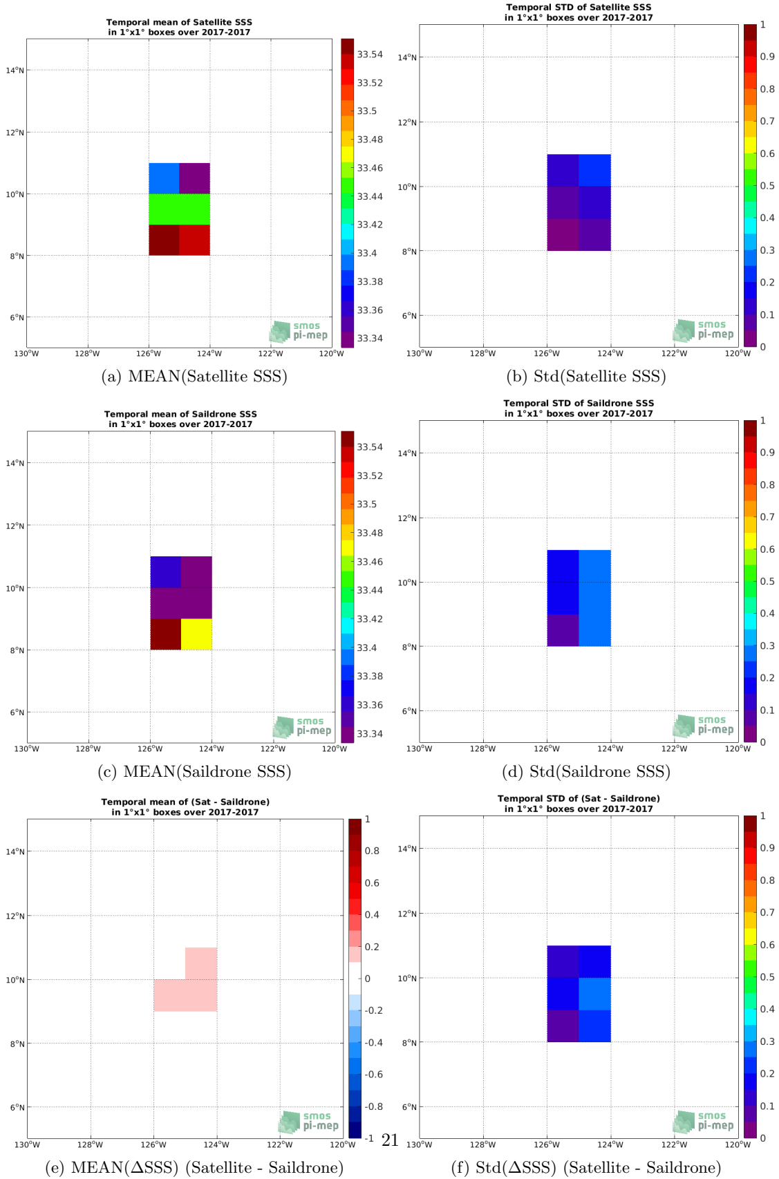
Figure 6: Temporal mean (left) and Std (right) of SSS from SMOS SSS L3 v5 - 18 Days (CATDS-CECOS-LOCEAN) (top), Saildrone (middle), and of \Delta SSS (Satellite - Saildrone). Only match-pairs are used to generate these maps.
