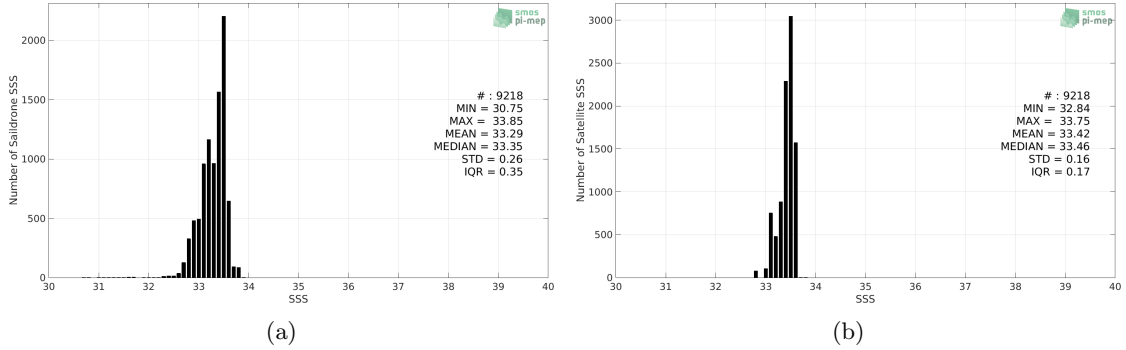
Figure 2: Histograms of SSS from Saildrone (a) and SMOS SSS L3 v5 - 18 Days (CATDS-CECOS-LOCEAN) (b) considering all match-up pairs per bins of 0.1 over the SPURS 2 Pi-MEP region and for the full satellite product period.
