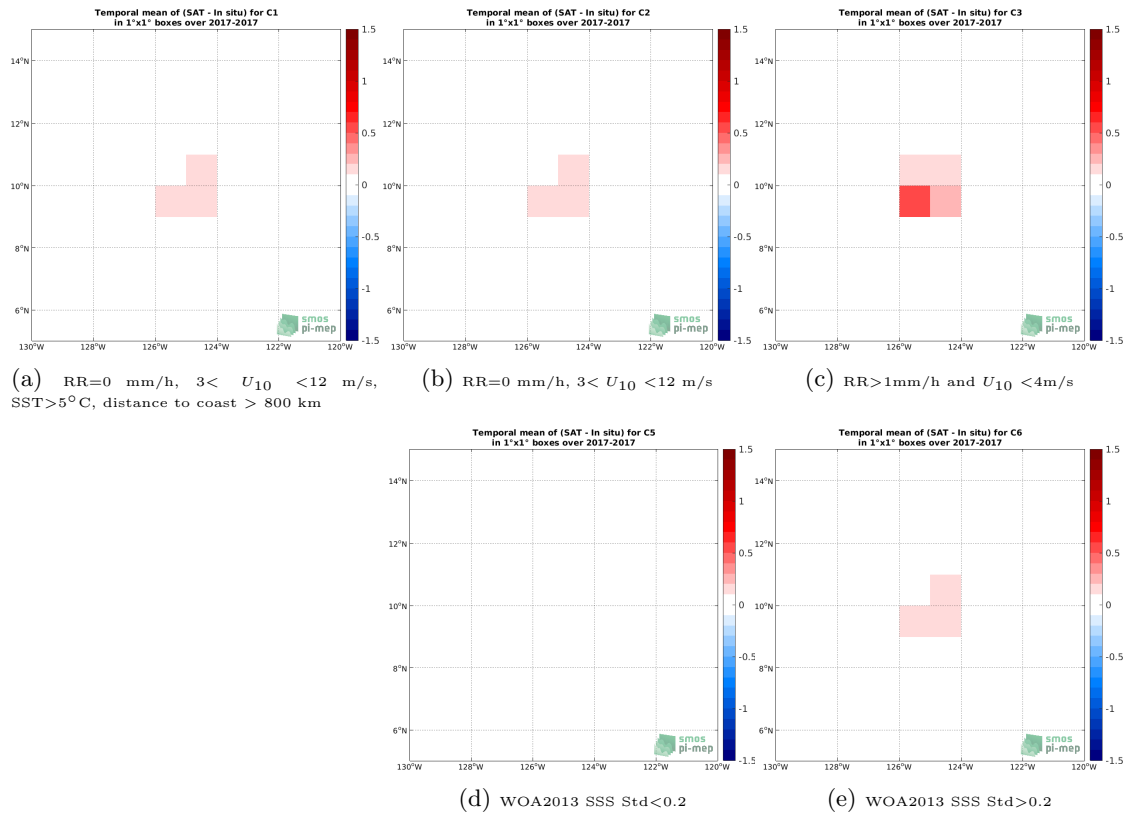
Figure 12: Temporal mean gridded over spatial boxes of size 1^\circ \times 1^\circ of \Delta\text{SSS} (SMOS SSS L3 v5 - 18 Days (CATDS-CECOS-LOCEAN) - Sairdrone) for 5 different subdatasets corresponding to:RR=0 mm/h, 3 < U_{10} < 12 m/s, SST >5^\circ\text{C} , distance to coast > 800 km (a), RR=0 mm/h, 3 < U_{10} < 12 m/s (b), RR >1 mm/h and U_{10} < 4 m/s (c), WOA2013 SSS Std <0.2 (d), WOA2013 SSS Std >0.2 (e).
