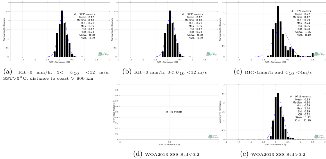
Figure 13: Normalized histogram of \Delta\text{SSS} (SMOS SSS L3 v5 - 18 Days (CATDS-CECOS-LOCEAN) - Saildrone) for 5 different subdatasets corresponding to: RR=0 mm/h, 3 < U_{10} < 12 m/s, SST > 5^{\circ}\text{C} , distance to coast > 800 km (a), RR=0 mm/h, 3 < U_{10} < 12 m/s (b), RR > 1\text{mm/h} and U_{10} < 4\text{m/s} (c), WOA2013 SSS Std < 0.2 (d), WOA2013 SSS Std > 0.2 (e).
