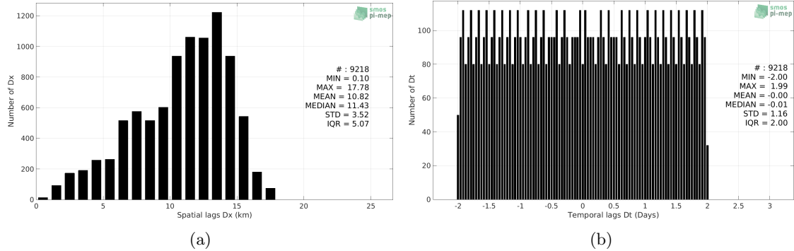
Figure 5: Histograms of the spatial (a) and temporal (b) lags between the time of the Saildrone measurements and the date of the corresponding SMOS SSS L3 v5 - 18 Days (CATDS-CECOS-LOCEAN) SSS product.
