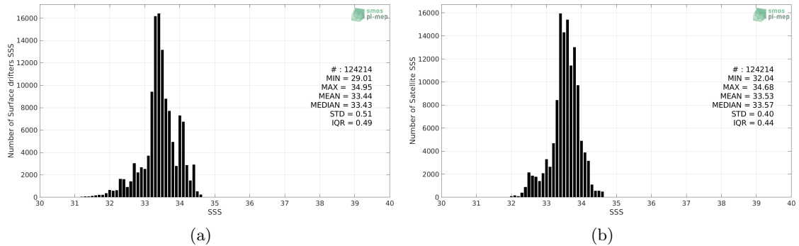
Figure 2: Histograms of SSS from Surface drifters (a) and SMOS SSS L3 v5 - 18 Days (CATDS-CECOS-LOCEAN) (b) considering all match-up pairs per bins of 0.1 over the SPURS 2 Pi-MEP region and for the full satellite product period.
