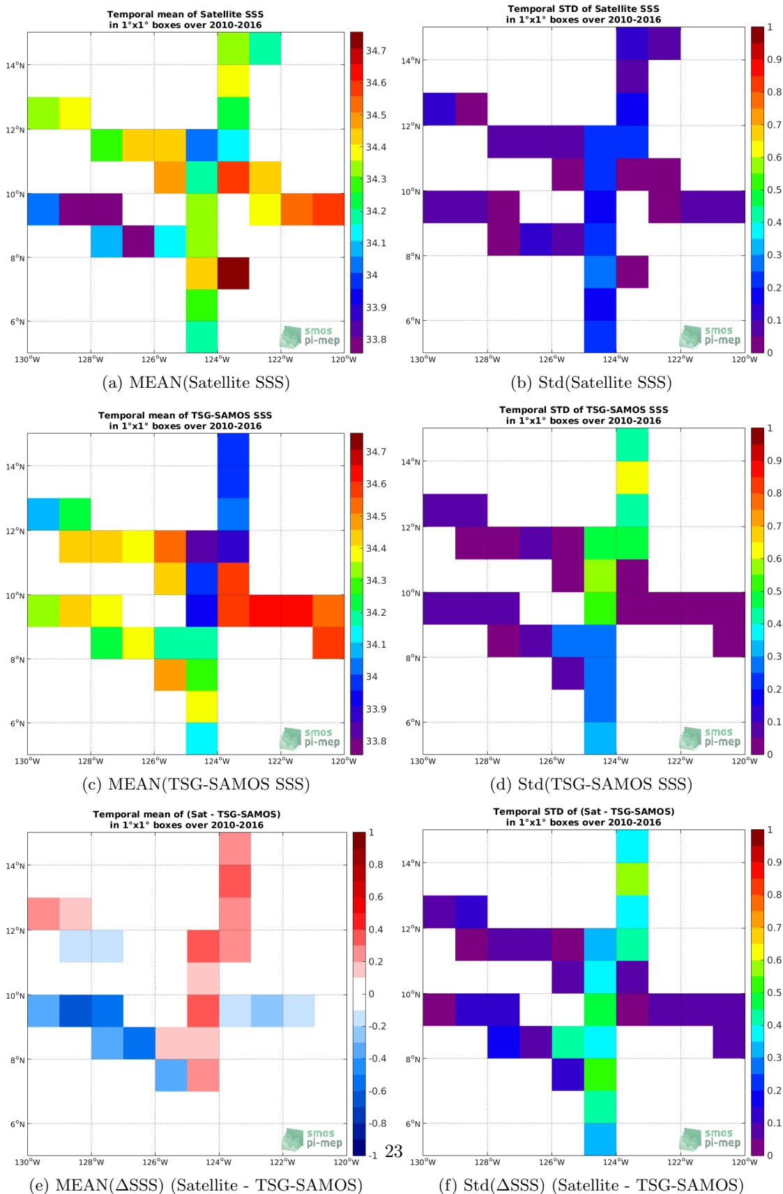
Figure 6: Temporal mean (left) and Std (right) of SSS from SMOS L3 v2 - Monthly - 0.25 Deg (CATDS-CECOS-IFREMER) (top), TSG-SAMOS (middle), and of \Delta SSS (Satellite - TSG-SAMOS). Only match-up pairs are used to generate these maps.
