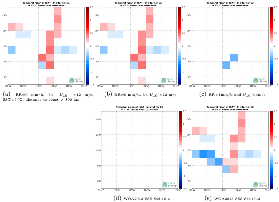
Figure 12: Temporal mean gridded over spatial boxes of size 1^{\circ}\times 1^{\circ} of \Delta\text{SSS} (SMOS L3 v2 - Monthly - 0.25 Deg (CATDS-CECOS-IFREMER) - TSG-SAMOS) for 5 different subdatasets corresponding to:RR=0 mm/h, 3 < U_{10} < 12 m/s, SST >5^{\circ}\text{C} , distance to coast > 800 km (a), RR=0 mm/h, 3 < U_{10} < 12 m/s (b), RR >1 mm/h and U_{10} < 4 m/s (c), WOA2013 SSS Std <0.2 (d), WOA2013 SSS Std >0.2 (e).
