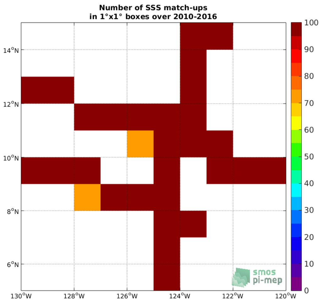
Figure 4: Number of SSS match-ups between TSG-SAMOS SSS and the SMOS L3 v2 - Monthly - 0.25 Deg (CATDS-CECOS-IFREMER) SSS product for the SPURS 2 Pi-MEP region over 1°x1° boxes and for the full satellite product period.
