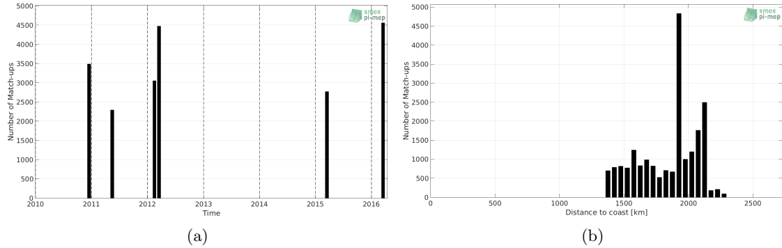
Figure 1: Number of match-ups between TSG-SAMOS and SMOS L3 v2 - Monthly - 0.25 Deg (CATDS-CECOS-IFREMER) SSS as a function of time (a) and as function of the distance to coast (b) over the SPURS 2 Pi-MEP region and for the full satellite product period.
