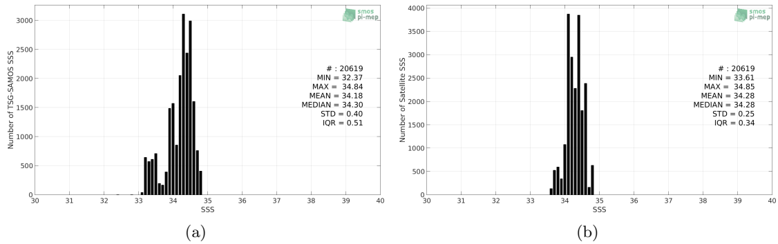
Figure 2: Histograms of SSS from TSG-SAMOS (a) and SMOS L3 v2 - Monthly - 0.25 Deg (CATDS-CECOS-IFREMER) (b) considering all match-up pairs per bins of 0.1 over the SPURS 2 Pi-MEP region and for the full satellite product period.
