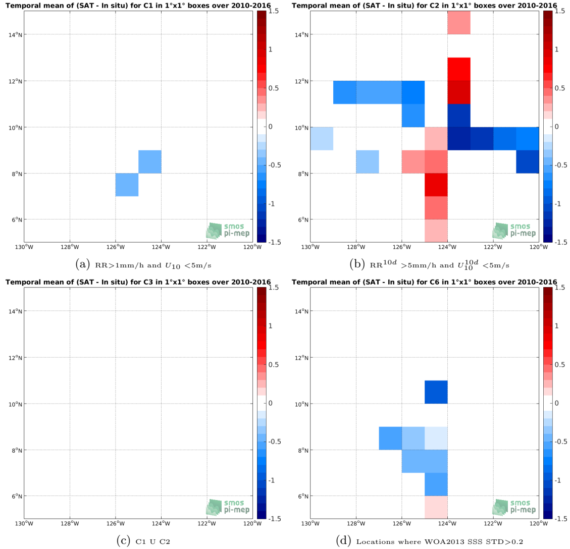
Figure 12: Temporal mean gridded over spatial boxes of size 1^\circ \times 1^\circ of \Delta SSS (SMOS-L3-CATDS-IFREMER-CECOS-V2-MONTHLY-0.25DEG - TSG-SAMOS) for 4 different subdatasets corresponding to: RR > 1mm/h and U_{10} < 5\text{m/s} (a), RR 10d > 5mm/h and U_{10}^{10d} < 5\text{m/s} (b), C1 U C2 (c), Locations where WOA2013 SSS STD > 0.2 (d).
