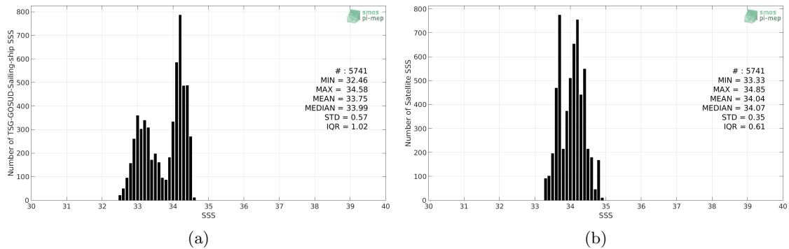
Figure 2: Histograms of SSS from TSG-GOSUD-Sailing-ship (a) and SMOS L3 v2 - Monthly - 0.25 Deg (CATDS-CECOS-IFREMER) (b) considering all match-up pairs per bins of 0.1 over the SPURS 2 Pi-MEP region and for the full satellite product period.
