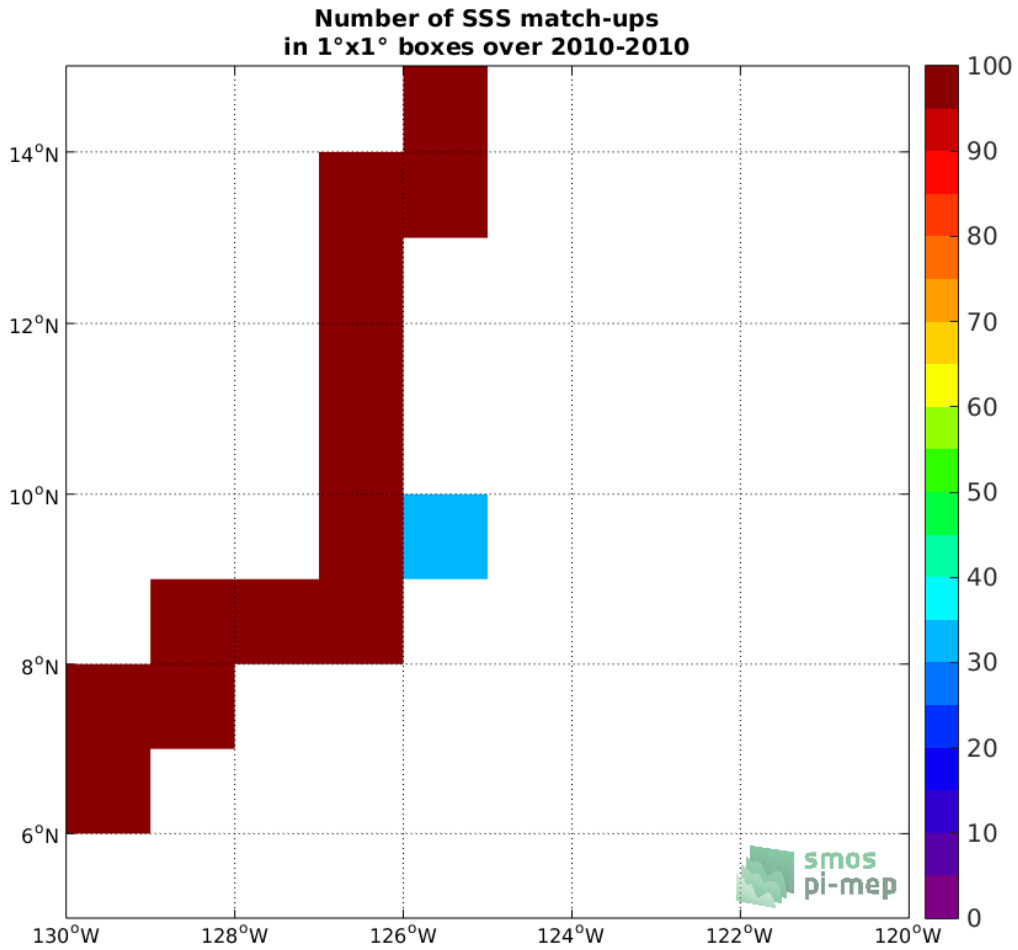
Figure 4: Number of SSS match-ups between TSG-GOSUD-Sailing-ship SSS and the SMOS L3 v2 - Monthly - 0.25 Deg (CATDS-CECOS-IFREMER) SSS product for the SPURS 2 Pi-MEP region over 1°x1° boxes and for the full satellite product period.
