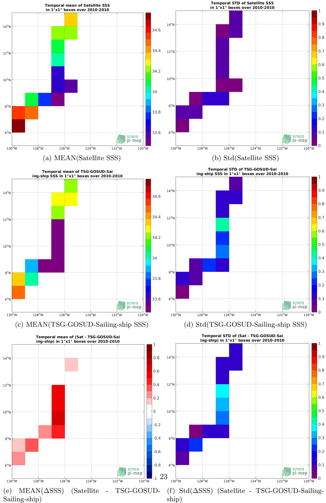
Figure 6: Temporal mean (left) and Std (right) of SSS from SMOS L3 v2 - Monthly - 0.25 Deg (CATDS-CECOS-IFREMER) (top), TSG-GOSUD-Sailing-ship (middle), and of \Delta SSS (Satellite - TSG-GOSUD-Sailing-ship). Only match-up pairs are used to generate these maps.
