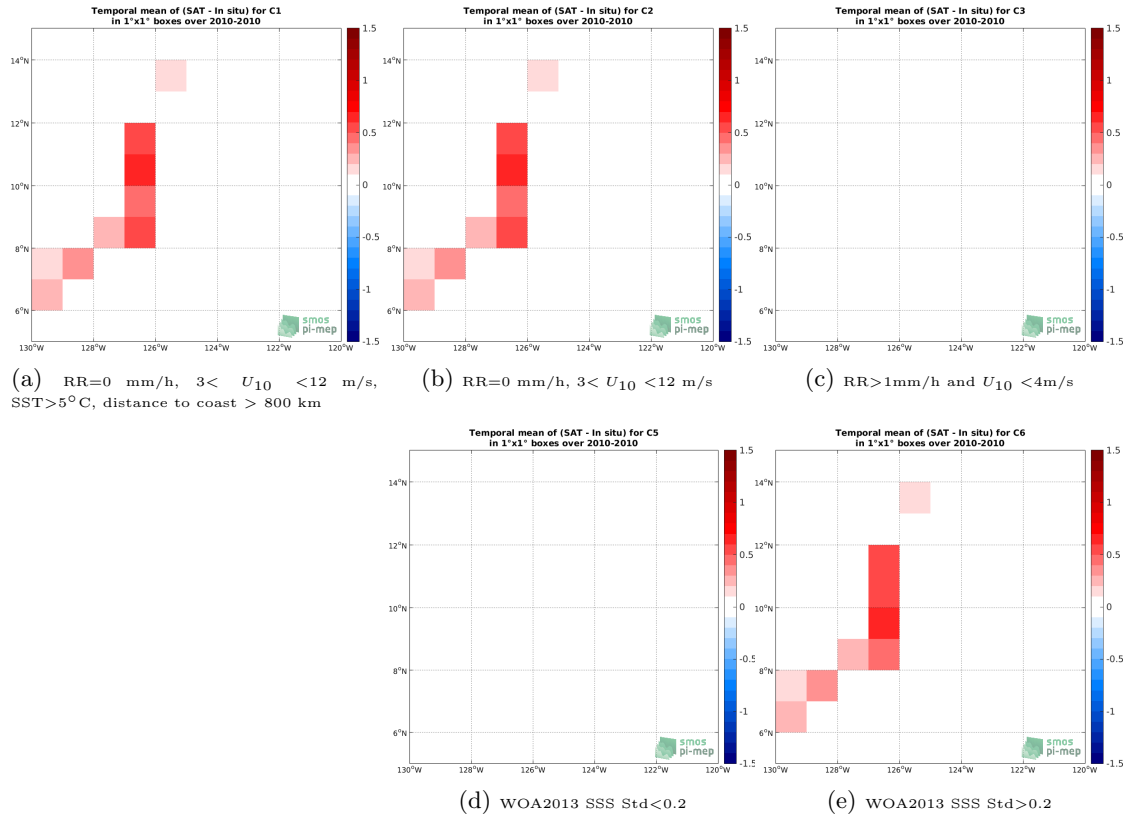
Figure 12: Temporal mean gridded over spatial boxes of size 1^{\circ} \times 1^{\circ} of \Delta SSS (SMOS L3 v2 - Monthly - 0.25 Deg (CATDS-CECOS-IFREMER) - TSG-GOSUD-Sailing-ship) for 5 different subdatasets corresponding to:RR=0 mm/h, 3 < U_{10} < 12 m/s, SST>5°C, distance to coast > 800 km (a), RR=0 mm/h, 3 < U_{10} < 12 m/s (b), RR>1mm/h and U_{10} < 4 m/s (c), WOA2013 SSS Std<0.2 (d), WOA2013 SSS Std>0.2 (e).
