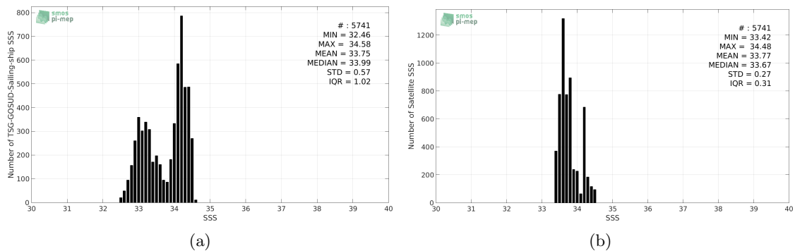
Figure 2: Histograms of SSS from TSG-GOSUD-Sailing-ship (a) and SMOS-L3-CATDS-IFREMER-CECOS-V2-MONTHLY-0.25DEG (b) considering all match-up pairs per bins of 0.1 over the SPURS 2 Pi-MEP region and for the full satellite product period.
