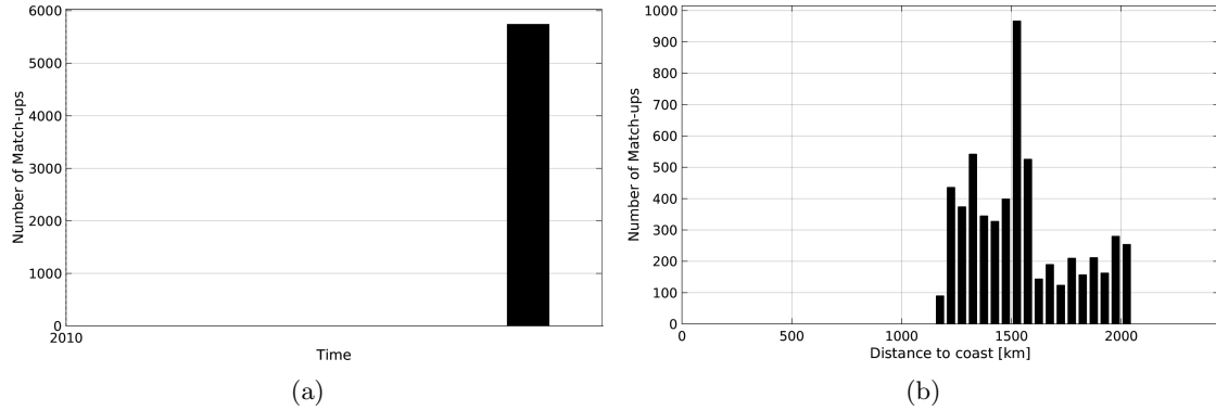
Figure 1: Number of match-ups between TSG-GOSUD-Sailing-ship and SMOS-L3-CATDS-IFREMER-CECOS-V2-MONTHLY-0.25DEG SSS as a function of time (a) and as function of the distance to coast (b) over the SPURS 2 Pi-MEP region and for the full satellite product period.
