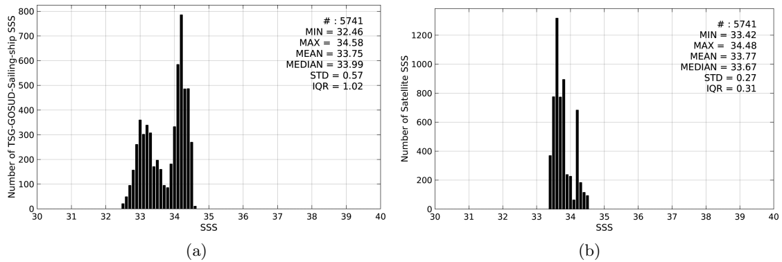
Figure 2: Histograms of SSS from TSG-GOSUD-Sailing-ship (a) and SMOS-L3-CATDS-IFREMER-CECOS-V2-MONTHLY-0.25DEG (b) considering all match-up pairs per bins of 0.1 over the SPURS 2 Pi-MEP region and for the full satellite product period.
