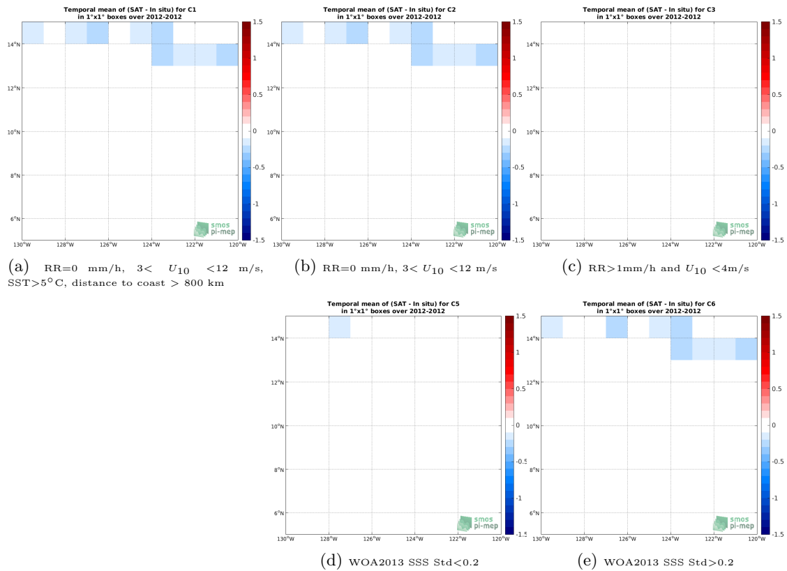
Figure 12: Temporal mean gridded over spatial boxes of size 1^{\circ} \times 1^{\circ} of \Delta SSS (SMOS L3 v2 - Monthly - 0.25 Deg (CATDS-CECOS-IFREMER) - TSG-GOSUD-Research-vessel) for 5 different subdatasets corresponding to:RR=0 mm/h, 3 < U_{10} < 12 m/s, SST>5°C, distance to coast > 800 km (a), RR=0 mm/h, 3 < U_{10} < 12 m/s (b), RR>1mm/h and U_{10} < 4 m/s (c), WOA2013 SSS Std<0.2 (d), WOA2013 SSS Std>0.2 (e).
