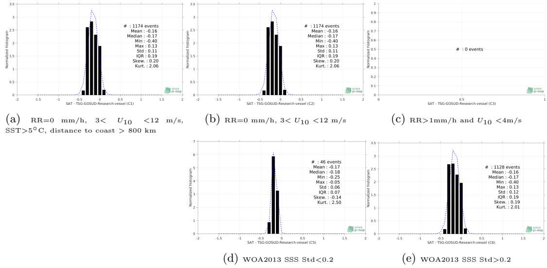
Figure 13: Normalized histogram of \Delta SSS (SMOS L3 v2 - Monthly - 0.25 Deg (CATDS-CECOS-IFREMER) - TSG-GOSUD-Research-vessel) for 5 different subdatasets corresponding to: RR=0 mm/h, 3 < U_{10} < 12 m/s, SST > 5°C, distance to coast > 800 km (a), RR=0 mm/h, 3 < U_{10} < 12 m/s (b), RR > 1mm/h and U_{10} < 4 m/s (c), WOA2013 SSS Std < 0.2 (d), WOA2013 SSS Std > 0.2 (e).
