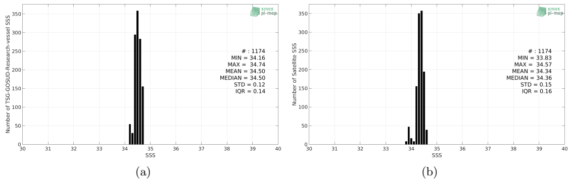
Figure 2: Histograms of SSS from TSG-GOSUD-Research-vessel (a) and SMOS L3 v2 - Monthly - 0.25 Deg (CATDS-CECOS-IFREMER) (b) considering all match-up pairs per bins of 0.1 over the SPURS 2 Pi-MEP region and for the full satellite product period.
