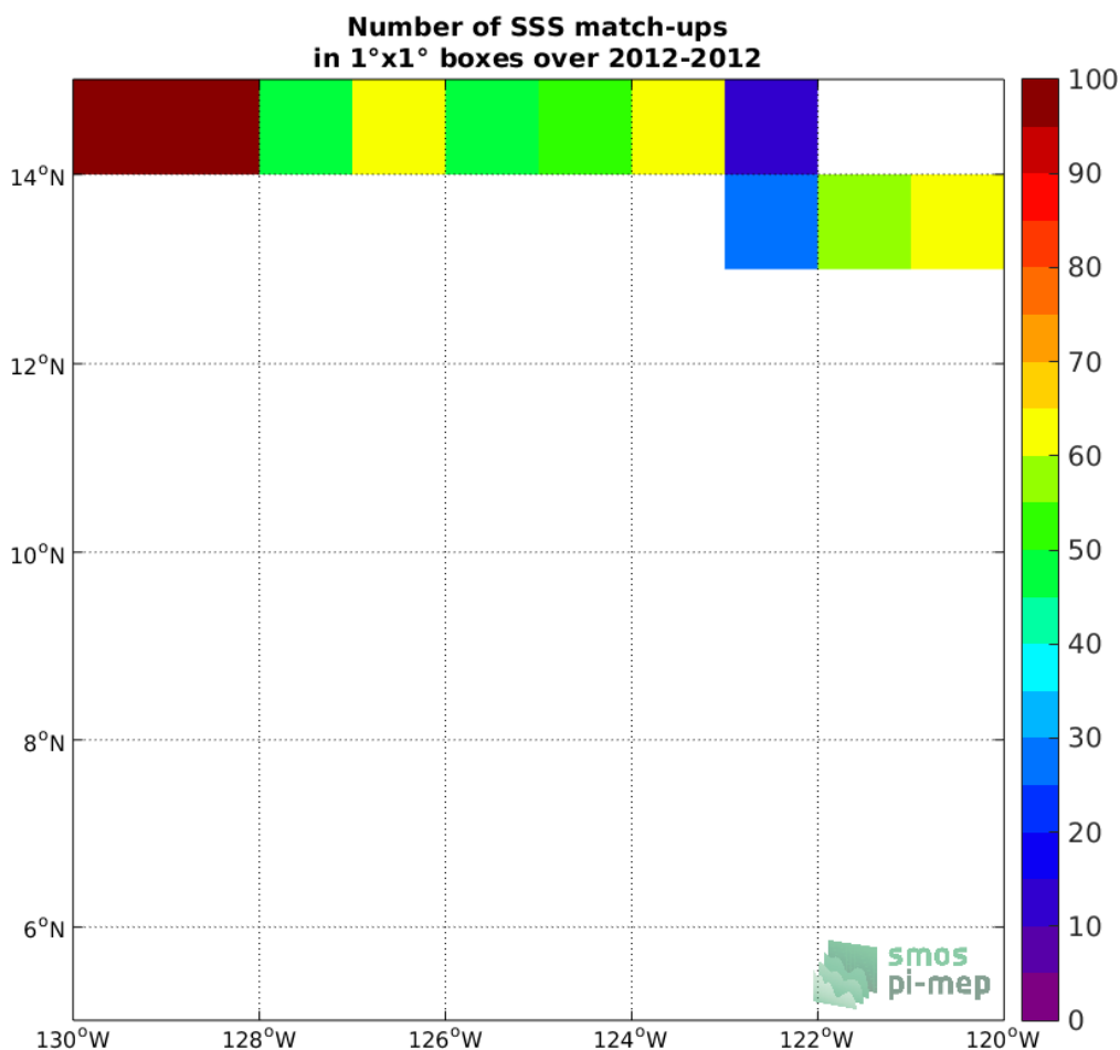
Figure 4: Number of SSS match-ups between TSG-GOSUD-Research-vessel SSS and the SMOS L3 v2 - Monthly - 0.25 Deg (CATDS-CECOS-IFREMER) SSS product for the SPURS 2 Pi-MEP region over 1°x1° boxes and for the full satellite product period.
