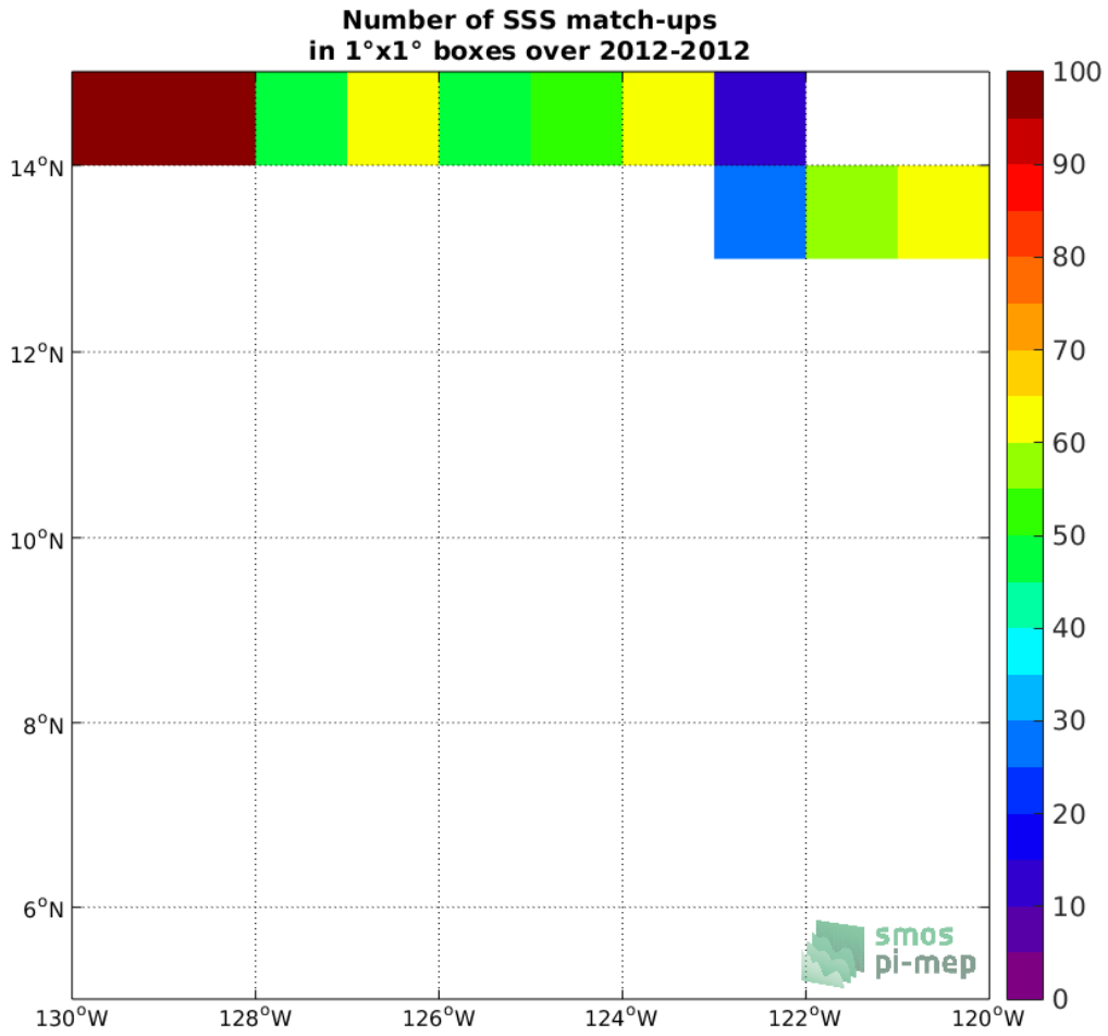
Figure 4: Number of SSS match-ups between TSG-GOSUD-Research-vessel SSS and the SMOS-L3-CATDS-IFREMER-CECOS-V2-MONTHLY-0.25DEG SSS product for the SPURS 2 Pi-MEP region over 1°x1° boxes and for the full satellite product period.
