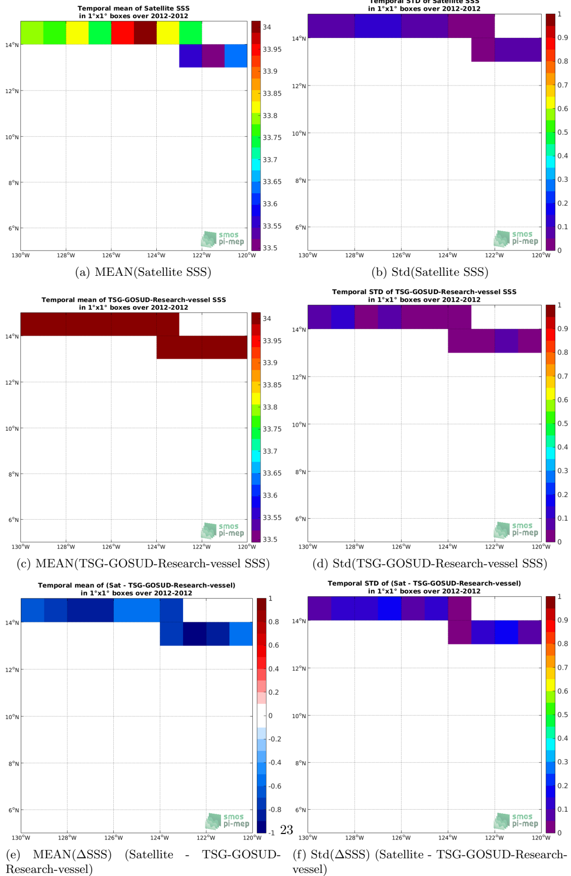
Figure 6: Temporal mean (left) and Std (right) of SSS from SMOS-L3-CATDS-IFREMER-CECOS-V2-MONTHLY-0.25DEG (top), TSG-GOSUD-Research-vessel (middle), and of \Delta SSS (Satellite - TSG-GOSUD-Research-vessel). Only match-up pairs are used to generate these maps.
