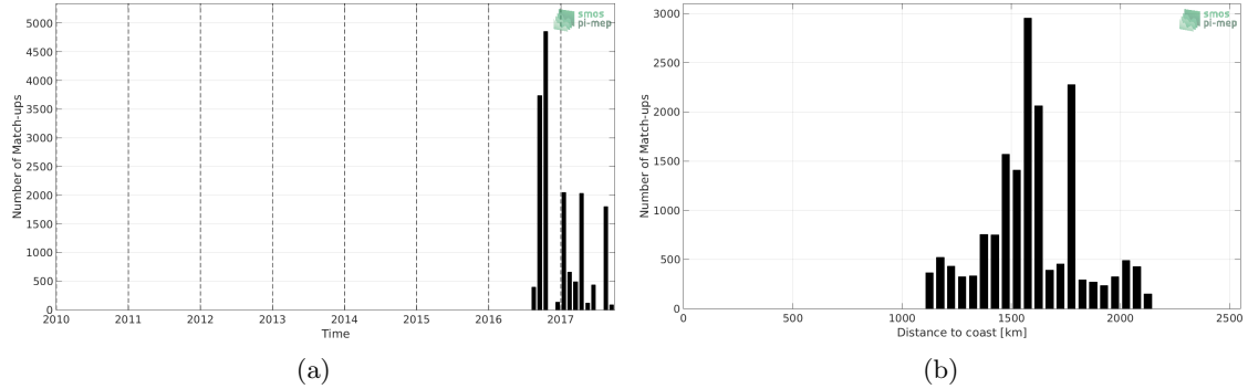
Figure 1: Number of match-ups between Surface drifters and SMOS L3 v2 - Monthly - 0.25 Deg (CATDS-CECOS-IFREMER) SSS as a function of time (a) and as function of the distance to coast (b) over the SPURS 2 Pi-MEP region and for the full satellite product period.
