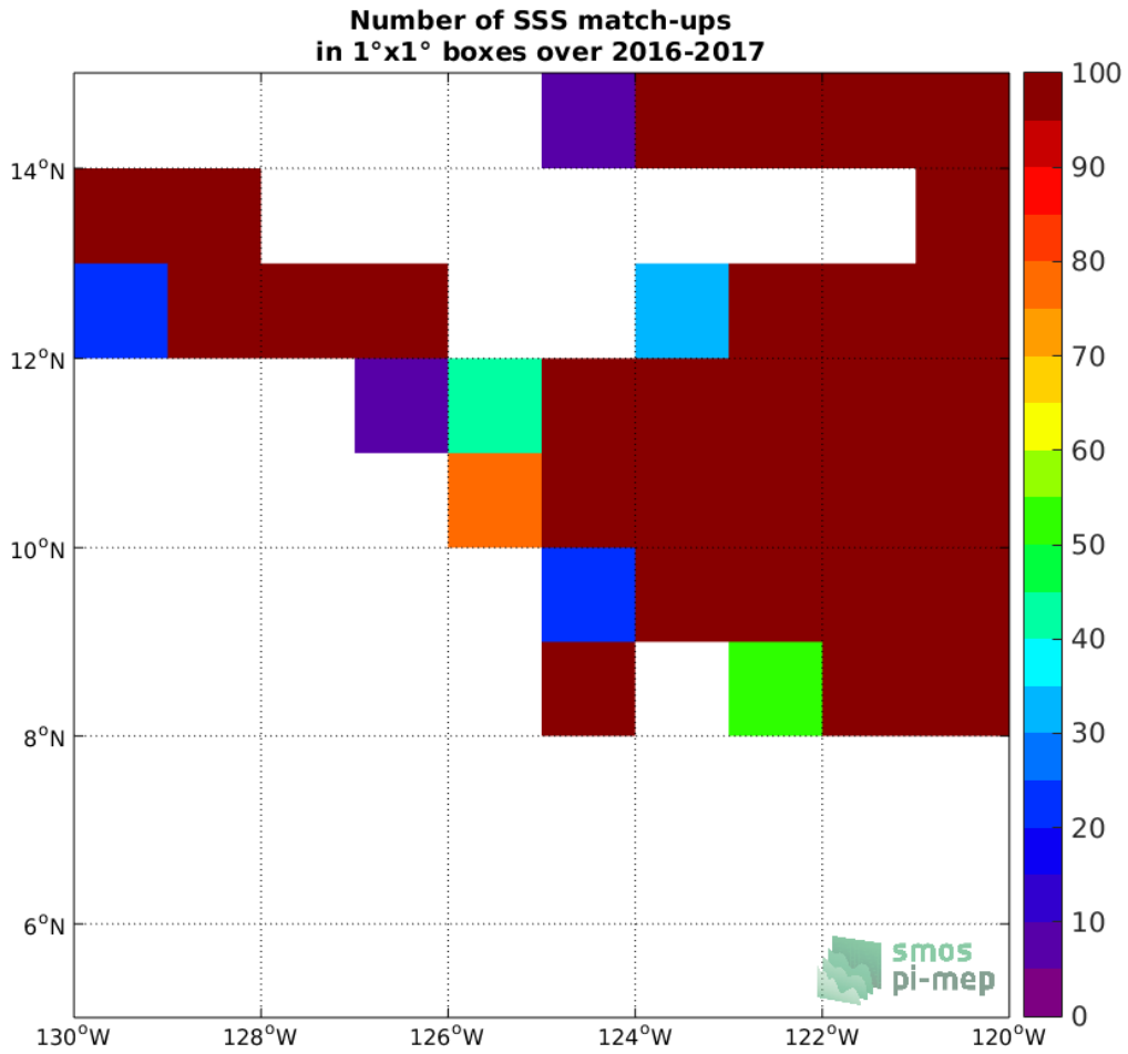
Figure 3: Number of SSS match-ups between Surface drifters SSS and the SMOS L3 v2 - Monthly - 0.25 Deg (CATDS-CECOS-IFREMER) SSS product for the SPURS 2 Pi-MEP region over 1°x1° boxes and for the full satellite product period.
