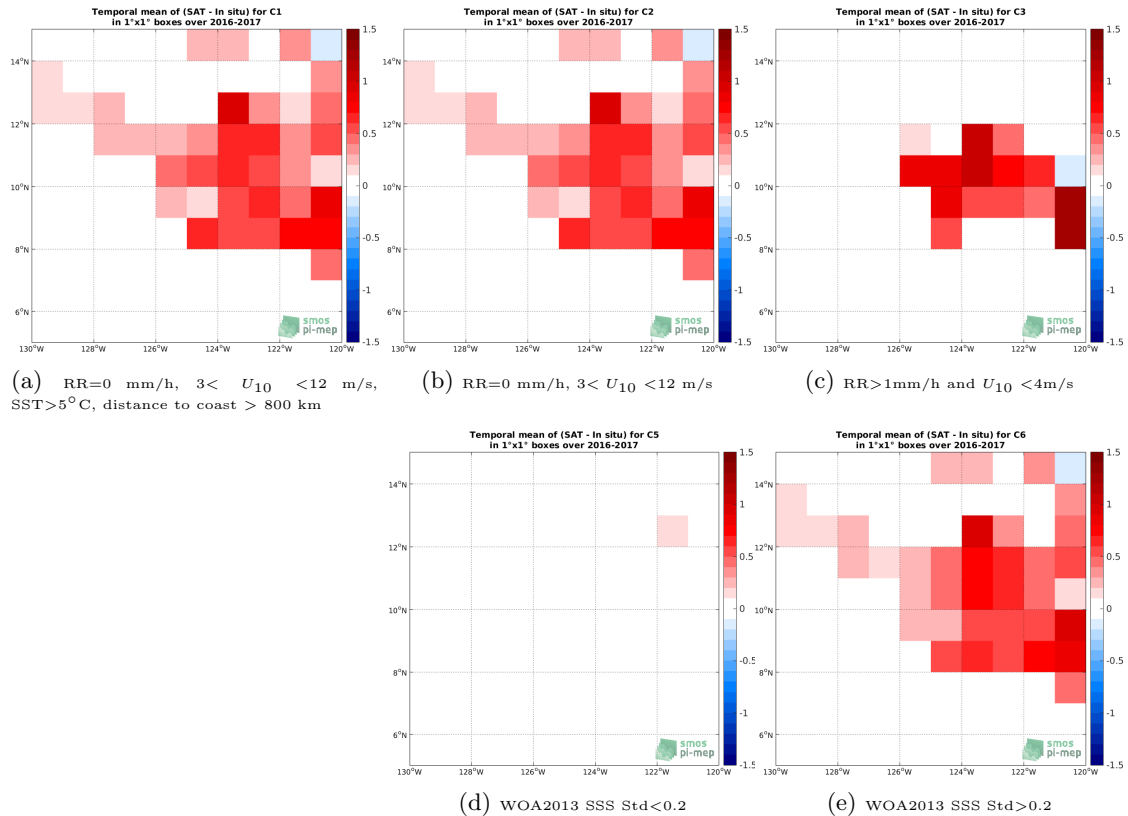
Figure 11: Temporal mean gridded over spatial boxes of size 1^{\circ}\times 1^{\circ} of \Delta\text{SSS} (SMOS L3 v2 - Monthly - 0.25 Deg (CATDS-CECOS-IFREMER) - Surface drifters) for 5 different subdatasets corresponding to: RR=0 mm/h, 3 < U_{10} < 12 m/s, SST > 5^{\circ}\text{C} , distance to coast > 800 km (a), RR=0 mm/h, 3 < U_{10} < 12 m/s (b), RR > 1 mm/h and U_{10} < 4 m/s (c), WOA2013 SSS Std < 0.2 (d), WOA2013 SSS Std > 0.2 (e).
