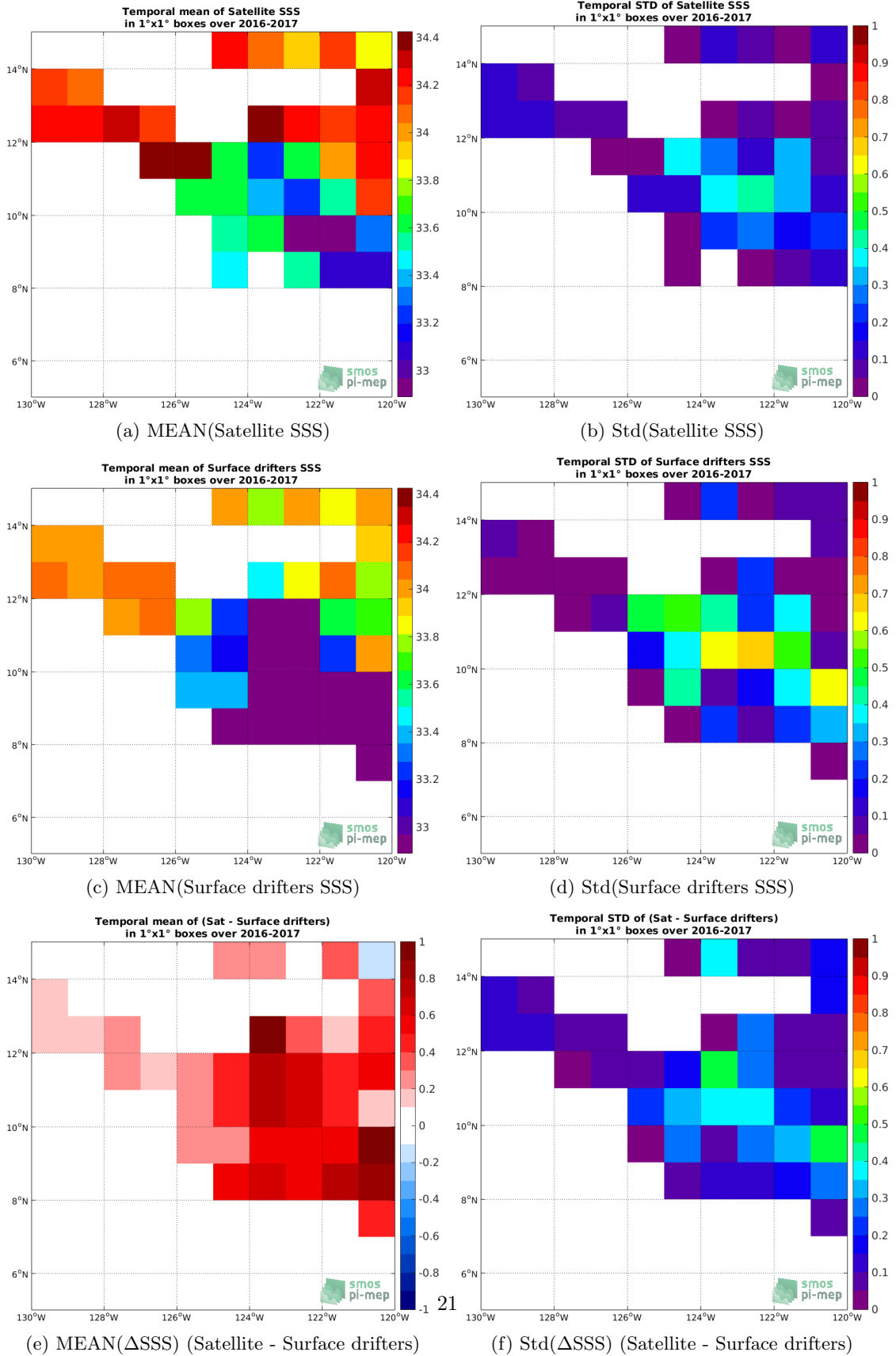
Figure 5: Temporal mean (left) and Std (right) of SSS from SMOS L3 v2 - Monthly - 0.25 Deg (CATDS-CECOS-IFREMER) (top), Surface drifters (middle), and of \Delta SSS (Satellite - Surface drifters). Only match-up pairs are used to generate these maps.
