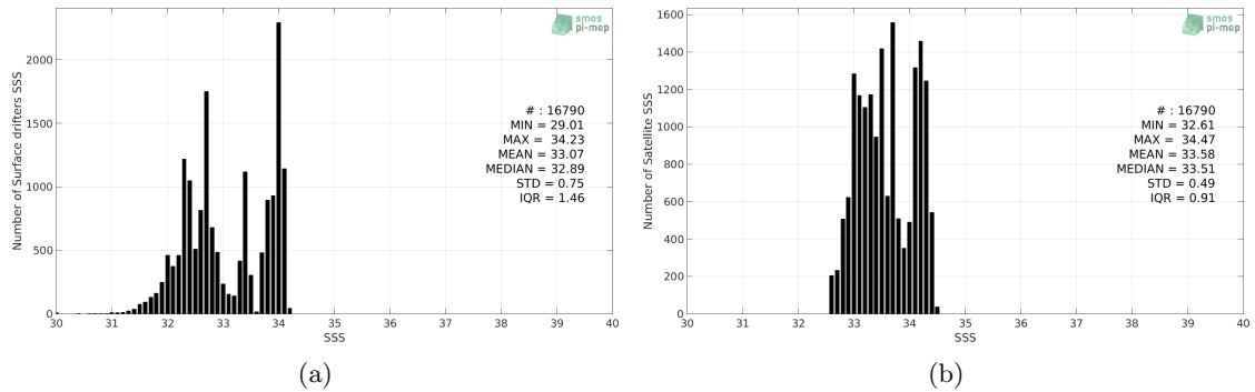
Figure 2: Histograms of SSS from Surface drifters (a) and SMOS L3 v2 - Monthly - 0.25 Deg (CATDS-CECOS-IFREMER) (b) considering all match-up pairs per bins of 0.1 over the SPURS 2 Pi-MEP region and for the full satellite product period.
