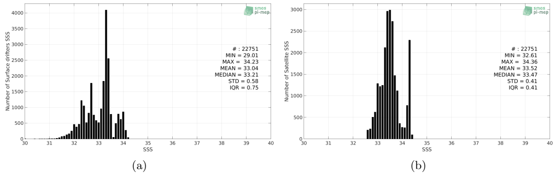
Figure 2: Histograms of SSS from Surface drifters (a) and SMOS-L3-CATDS-IFREMER-CECOS-V2-MONTHLY-0.25DEG (b) considering all match-up pairs per bins of 0.1 over the SPURS 2 Pi-MEP region and for the full satellite product period.
