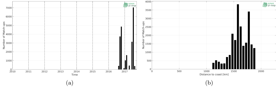
Figure 1: Number of match-ups between Surface drifters and SMOS-L3-CATDS-IFREMER-CECOS-V2-MONTHLY-0.25DEG SSS as a function of time (a) and as function of the distance to coast (b) over the SPURS 2 Pi-MEP region and for the full satellite product period.
