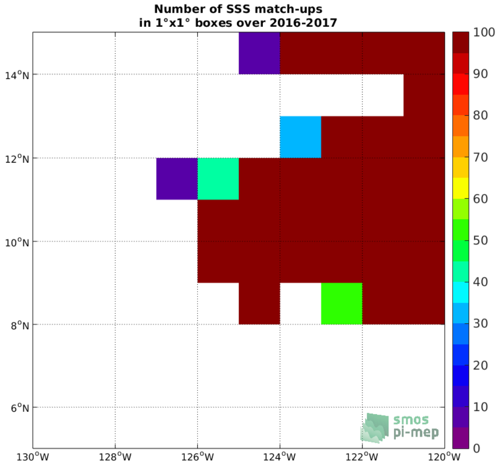
Figure 3: Number of SSS match-ups between Surface drifters SSS and the SMOS-L3-CATDS-IFREMER-CECOS-V2-MONTHLY-0.25DEG SSS product for the SPURS 2 Pi-MEP region over 1°x1° boxes and for the full satellite product period.
