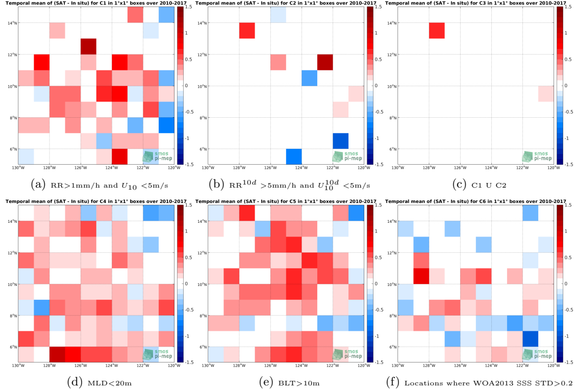
Figure 12: Temporal mean gridded over spatial boxes of size 1^\circ \times 1^\circ of \Delta\text{SSS} (SMOS-L3-CATDS-IFREMER-CECOS-V2-MONTHLY-0.25DEG - Argo) for 6 different subdatasets corresponding to: \text{RR} > 1\text{mm/h} and U_{10} < 5\text{m/s} (a), \text{RR}^{10d} > 5\text{mm/h} and U_{10}^{10d} < 5\text{m/s} (b), C1 U C2 (c), \text{MLD} < 20\text{m} (d), \text{BLT} > 10\text{m} (e), Locations where WOA2013 SSS STD > 0.2 (f).
