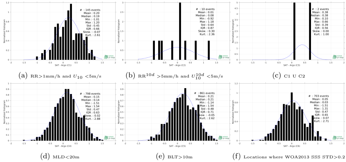
Figure 13: Normalized histogram of \Delta\text{SSS} (SMOS-L3-CATDS-IFREMER-CECOS-V2-MONTHLY-0.25DEG - Argo) for 6 different subdatasets corresponding to: RR > 1\text{mm/h} and U_{10} < 5\text{m/s} (a), RR^{10d} > 5\text{mm/h} and U_{10}^{10d} < 5\text{m/s} (b), C1 U C2 (c), MLD < 20\text{m} (d), BLT > 10\text{m} (e), Locations where WOA2013 SSS STD > 0.2 (f).
