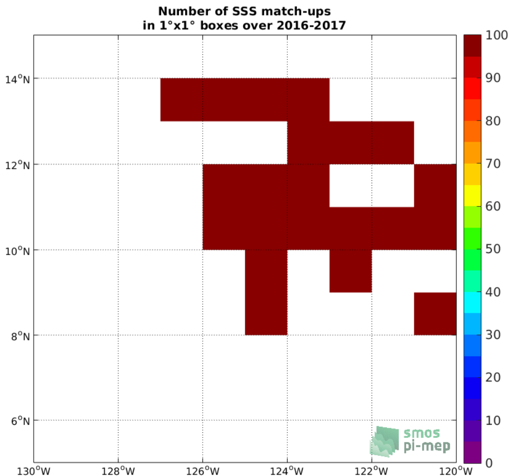
Figure 4: Number of SSS match-ups between Waveglider SSS and the SMOS SSS L3 v2 - Daily - 0.5 Deg (CATDS-CECOS-IFREMER) SSS product for the SPURS 2 Pi-MEP region over 1°x1° boxes and for the full satellite product period.
