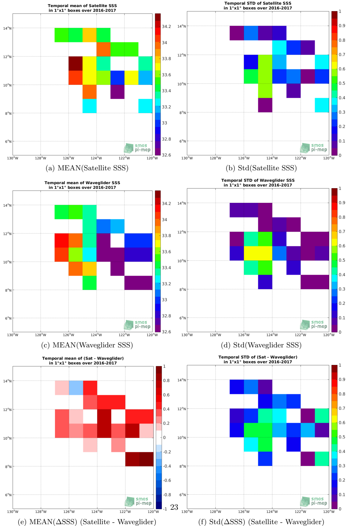
Figure 6: Temporal mean (left) and Std (right) of SSS from SMOS SSS L3 v2 - Daily - 0.5 Deg (CATDS-CECOS-IFREMER) (top), Waveglider (middle), and of \Delta SSS (Satellite - Waveglider). Only match-up pairs are used to generate these maps.
