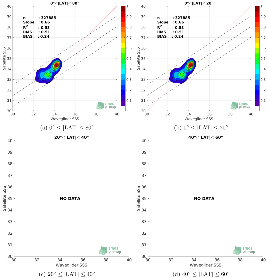
Figure 9: Contour maps of the concentration of SMOS SSS L3 v2 - Daily - 0.5 Deg (CATDS-CECOS-IFREMER) SSS (y-axis) versus Waveglider SSS (x-axis) at match-up pairs for different latitude bands. For each plot, the red line shows x=y . The black thin and dashed lines indicate a linear fit through the data cloud and the \pm 95\% confidence levels, respectively. The number match-up pairs n , the slope and R^2 coefficient of the linear fit, the root mean square (RMS) and the mean bias between satellite and in situ data are indicated for each latitude band in each plots.
