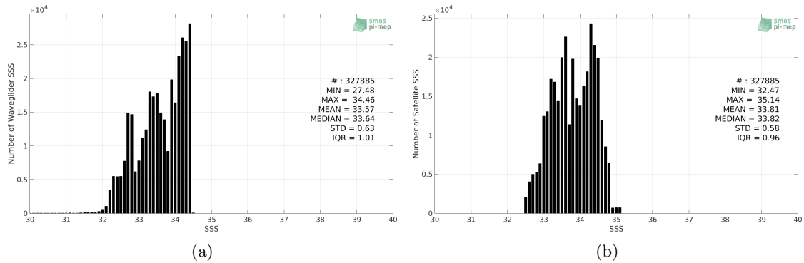
Figure 2: Histograms of SSS from Waveglider (a) and SMOS SSS L3 v2 - Daily - 0.5 Deg (CATDS-CECOS-IFREMER) (b) considering all match-up pairs per bins of 0.1 over the SPURS 2 Pi-MEP region and for the full satellite product period.
