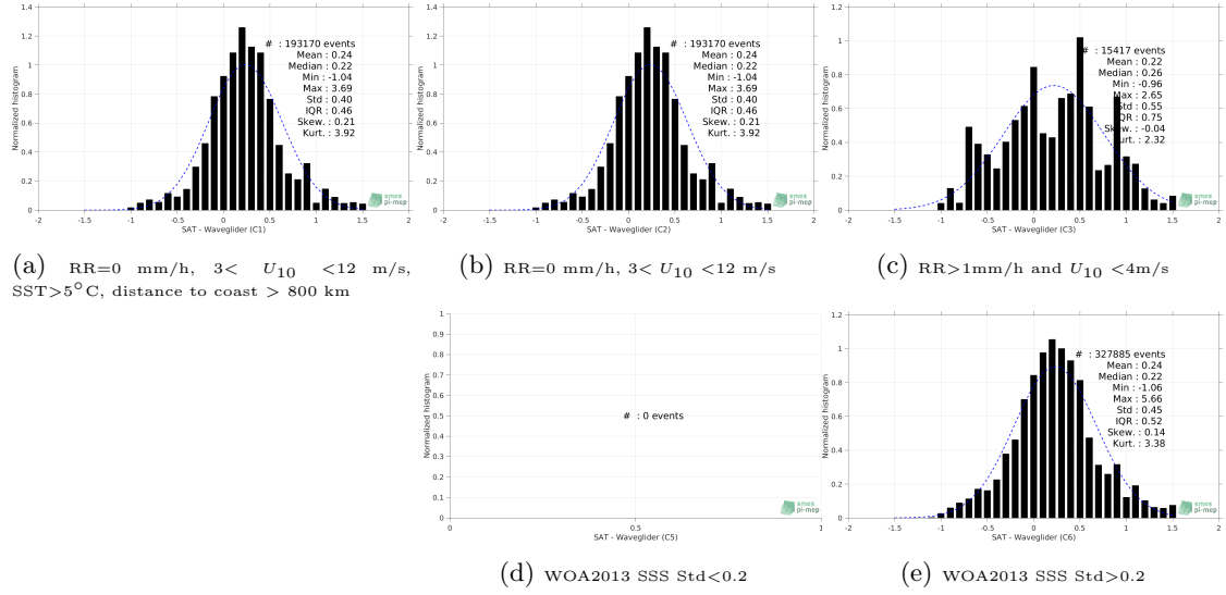
Figure 13: Normalized histogram of \Delta SSS (SMOS SSS L3 v2 - Daily - 0.5 Deg (CATDS-CECOS-IFREMER) - Waveglider) for 5 different subdatasets corresponding to: RR=0 mm/h, 3 < U_{10} < 12 m/s, SST > 5°C, distance to coast > 800 km (a), RR=0 mm/h, 3 < U_{10} < 12 m/s (b), RR > 1mm/h and U_{10} < 4 m/s (c), WOA2013 SSS Std < 0.2 (d), WOA2013 SSS Std > 0.2 (e).
