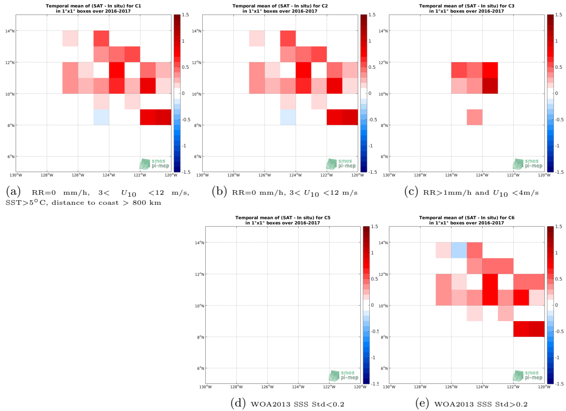
Figure 12: Temporal mean gridded over spatial boxes of size 1^{\circ}\times 1^{\circ} of \Delta\text{SSS} (SMOS SSS L3 v2 - Daily - 0.5 Deg (CATDS-CECOS-IFREMER) - Waveglider) for 5 different subdatasets corresponding to:RR=0 mm/h, 3 < U_{10} < 12 m/s, SST >5^{\circ}\text{C} , distance to coast > 800 km (a), RR=0 mm/h, 3 < U_{10} < 12 m/s (b), RR >1 mm/h and U_{10} < 4 m/s (c), WOA2013 SSS Std <0.2 (d), WOA2013 SSS Std >0.2 (e).
