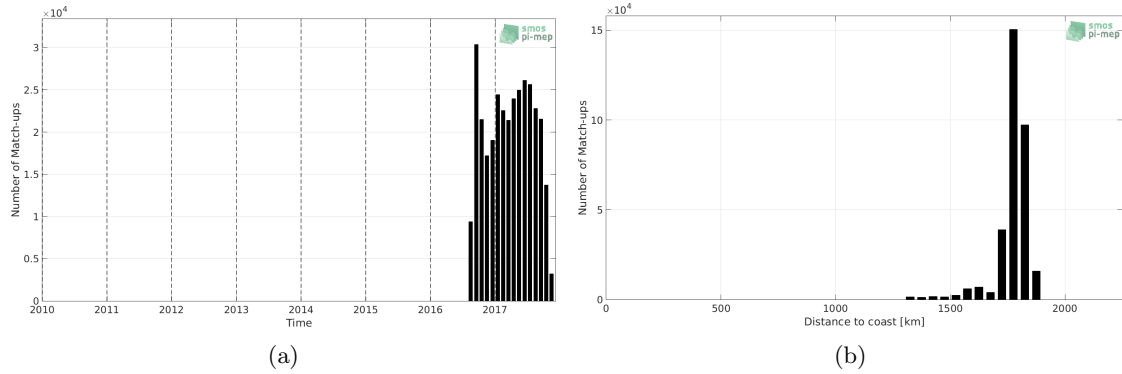
Figure 1: Number of match-ups between Waveglider and SMOS SSS L3 v2 - Daily - 0.5 Deg (CATDS-CECOS-IFREMER) SSS as a function of time (a) and as function of the distance to coast (b) over the SPURS 2 Pi-MEP region and for the full satellite product period.
