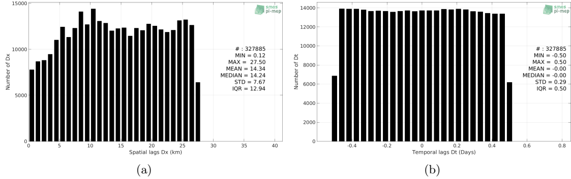
Figure 5: Histograms of the spatial (a) and temporal (b) lags between the time of the Waveglider measurements and the date of the corresponding SMOS SSS L3 v2 - Daily - 0.5 Deg (CATDS-CECOS-IFREMER) SSS product.
