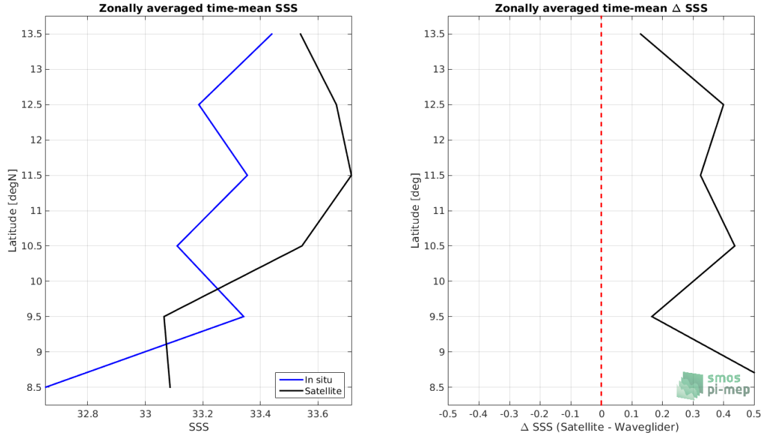
Figure 8: Left panel: Zonal mean SSS from SMOS SSS L3 v2 - Daily - 0.5 Deg (CATDS-CECOS-IFREMER) satellite product (black) and from Waveglider (blue). Right panel: Zonal mean of \Delta SSS (Satellite - Waveglider) for all the collected Pi-MEP match-up pairs estimated over the full satellite product period.
