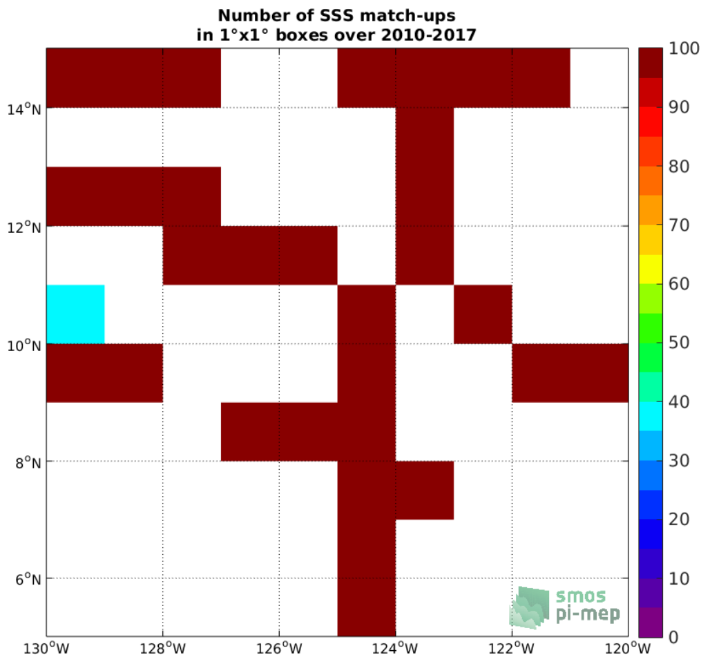
Figure 4: Number of SSS match-ups between TSG (SAMOS) SSS and the SMOS SSS L3 v2 - Daily - 0.5 Deg (CATDS-CECOS-IFREMER) SSS product for the SPURS 2 Pi-MEP region over 1°x1° boxes and for the full satellite product period.
