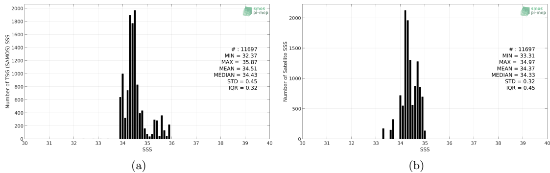
Figure 2: Histograms of SSS from TSG (SAMOS) (a) and SMOS SSS L3 v2 - Daily - 0.5 Deg (CATDS-CECOS-IFREMER) (b) considering all match-up pairs per bins of 0.1 over the SPURS 2 Pi-MEP region and for the full satellite product period.
