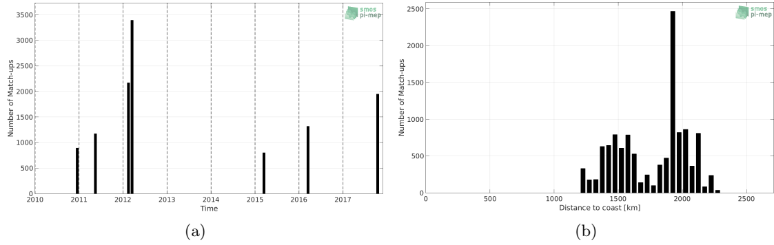
Figure 1: Number of match-ups between TSG (SAMOS) and SMOS SSS L3 v2 - Daily - 0.5 Deg (CATDS-CECOS-IFREMER) SSS as a function of time (a) and as function of the distance to coast (b) over the SPURS 2 Pi-MEP region and for the full satellite product period.
