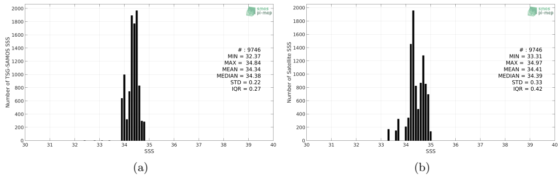
Figure 2: Histograms of SSS from TSG-SAMOS (a) and SMOS L3 v2 - Daily - 0.5 Deg (CATDS-CECOS-IFREMER) (b) considering all match-up pairs per bins of 0.1 over the SPURS 2 Pi-MEP region and for the full satellite product period.
