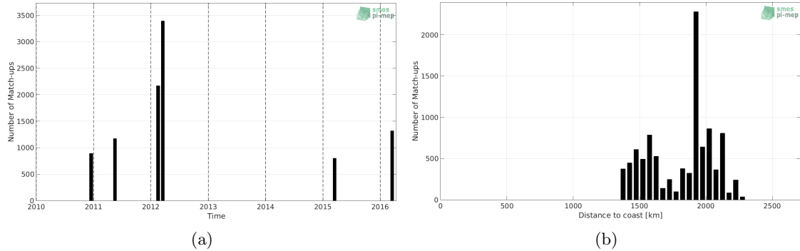
Figure 1: Number of match-ups between TSG-SAMOS and SMOS L3 v2 - Daily - 0.5 Deg (CATDS-CECOS-IFREMER) SSS as a function of time (a) and as function of the distance to coast (b) over the SPURS 2 Pi-MEP region and for the full satellite product period.
