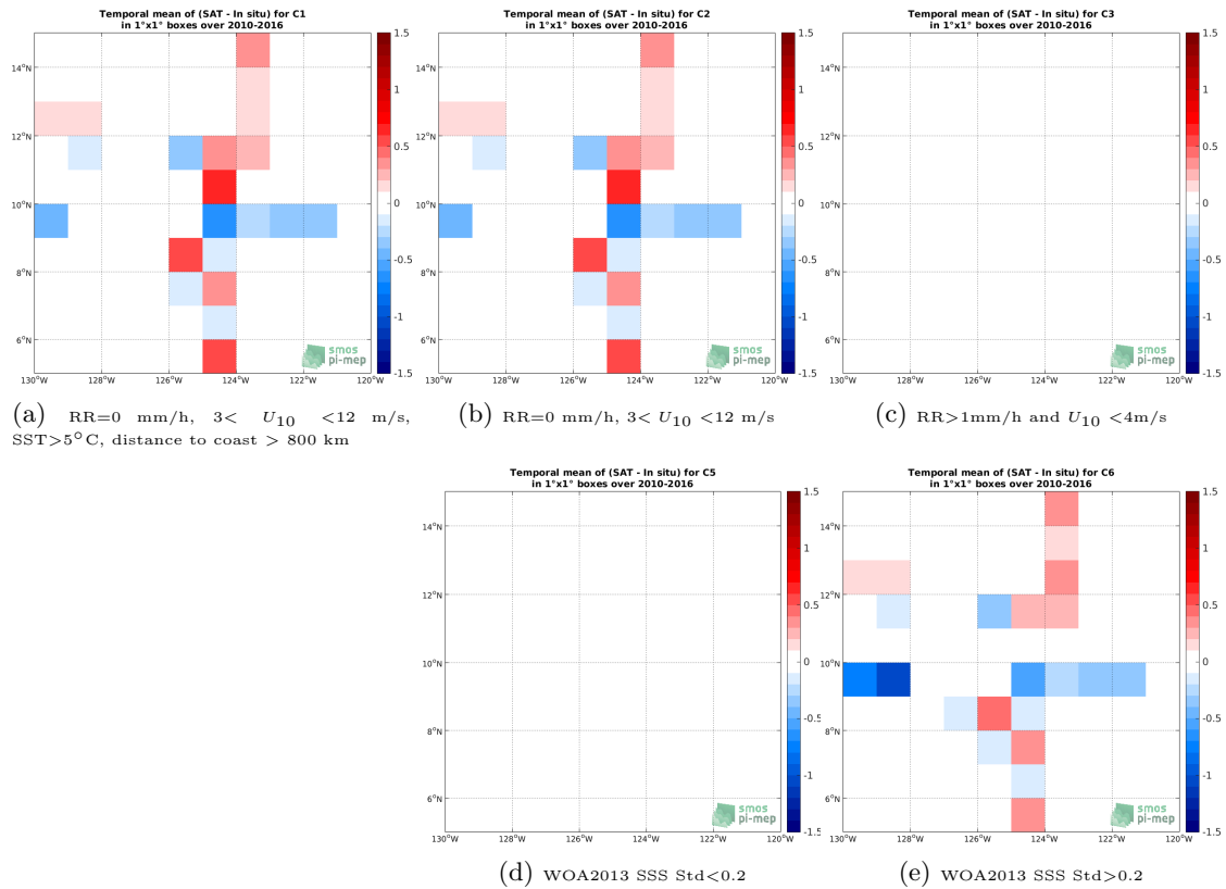
Figure 12: Temporal mean gridded over spatial boxes of size 1^\circ \times 1^\circ of \Delta SSS (SMOS L3 v2 - Daily - 0.5 Deg (CATDS-CECOS-IFREMER) - TSG-SAMOS) for 5 different subdatasets corresponding to:RR=0 mm/h, 3 < U_{10} < 12 m/s, SST >5^\circ\text{C} , distance to coast > 800 km (a), RR=0 mm/h, 3 < U_{10} < 12 m/s (b), RR >1 mm/h and U_{10} < 4 m/s (c), WOA2013 SSS Std <0.2 (d), WOA2013 SSS Std >0.2 (e).
