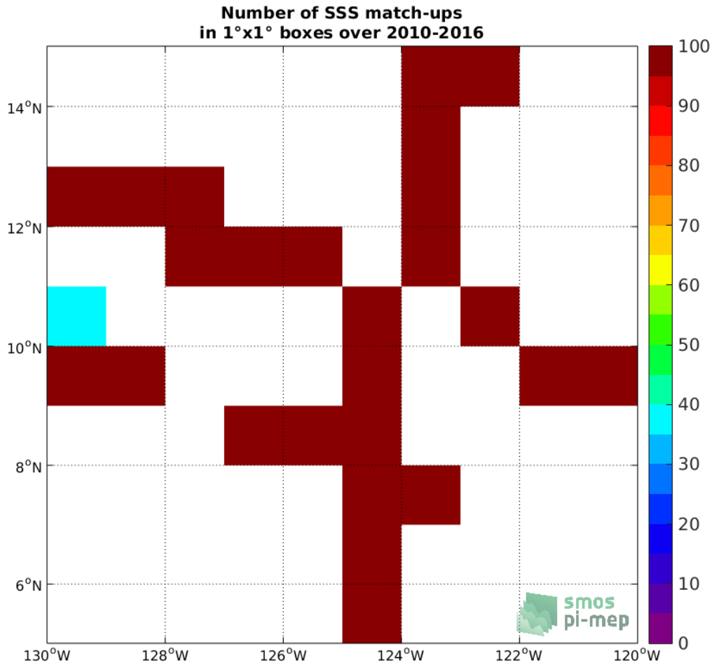
Figure 4: Number of SSS match-ups between TSG-SAMOS SSS and the SMOS L3 v2 - Daily - 0.5 Deg (CATDS-CECOS-IFREMER) SSS product for the SPURS 2 Pi-MEP region over 1°x1° boxes and for the full satellite product period.
