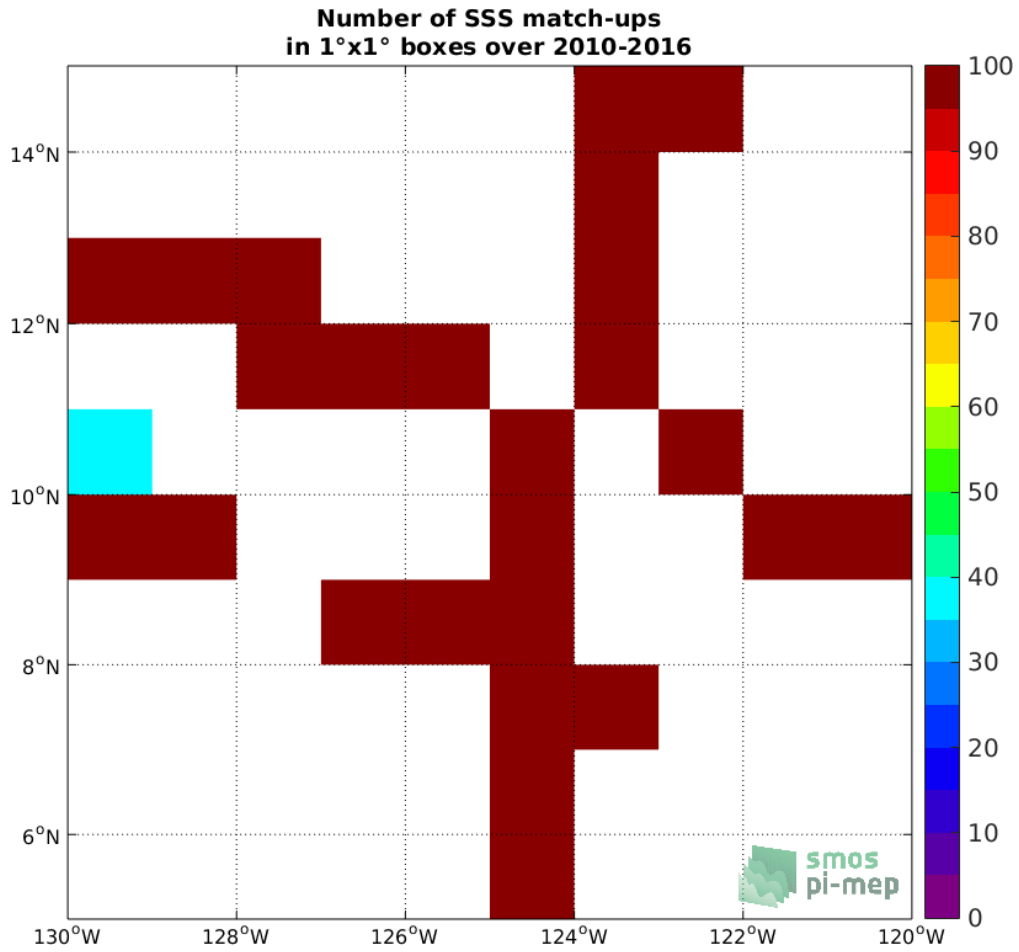
Figure 4: Number of SSS match-ups between TSG-SAMOS SSS and the SMOS-L3-CATDS-CECOS-IFREMER-V2-1DAY-0.5DEG SSS product for the SPURS 2 Pi-MEP region over 1°x1° boxes and for the full satellite product period.
