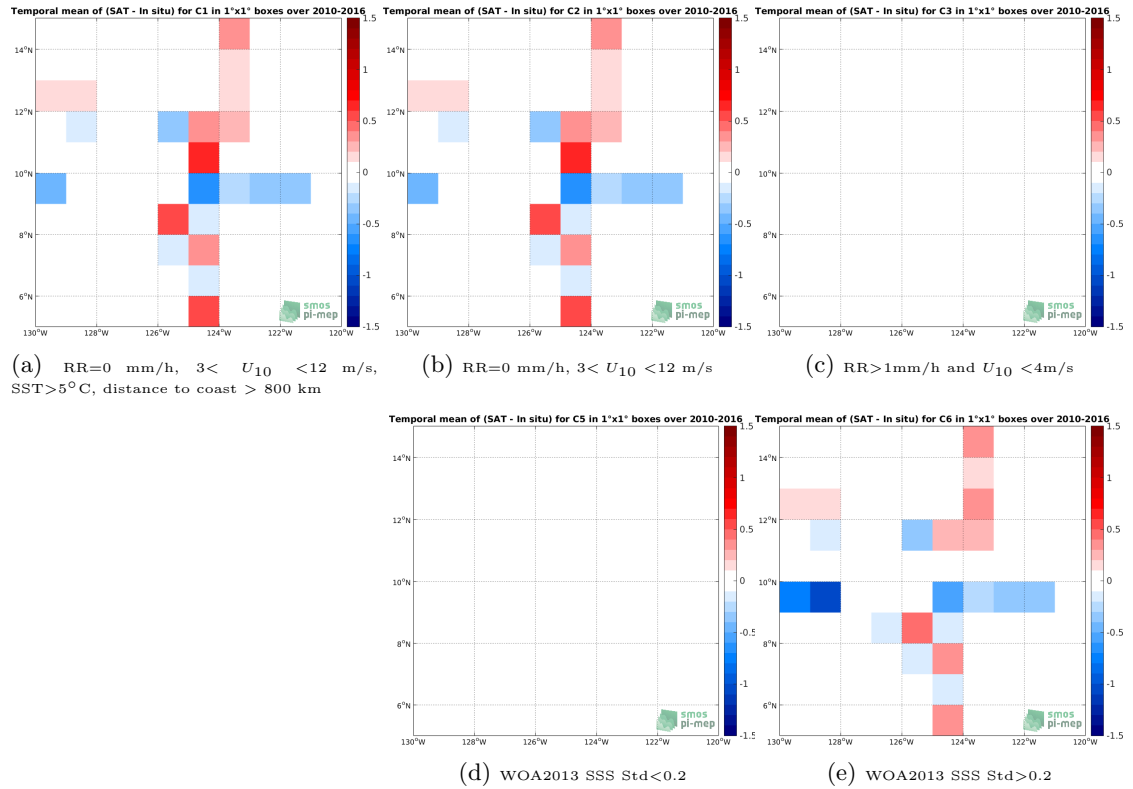
Figure 12: Temporal mean gridded over spatial boxes of size 1^\circ \times 1^\circ of \Delta SSS (SMOS-L3-CATDS-CECOS-IFREMER-V2-1DAY-0.5DEG - TSG-SAMOS) for 5 different subdatasets corresponding to:RR=0 mm/h, 3 < U_{10} < 12 m/s, SST >5^\circ C, distance to coast > 800 km (a), RR=0 mm/h, 3 < U_{10} < 12 m/s (b), RR >1 mm/h and U_{10} < 4 m/s (c), WOA2013 SSS Std <0.2 (d), WOA2013 SSS Std >0.2 (e).
