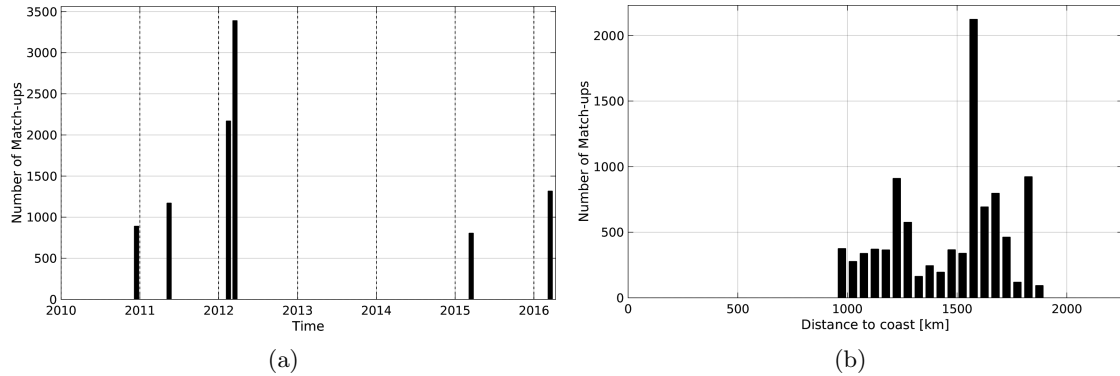
Figure 1: Number of match-ups between TSG-SAMOS and SMOS-L3-CATDS-CECOS-IFREMER-V2-1DAY-0.5DEG SSS as a function of time (a) and as function of the distance to coast (b) over the SPURS 2 Pi-MEP region and for the full satellite product period.
