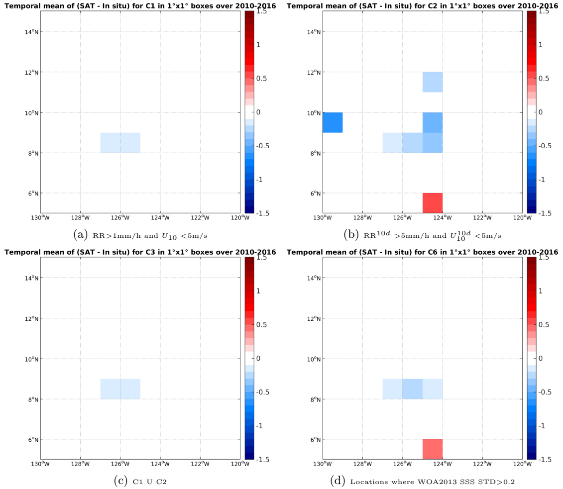
Figure 12: Temporal mean gridded over spatial boxes of size 1°x1° of \Delta SSS (SMOS-L3-CATDS-CECOS-IFREMER-V2-1DAY-0.5DEG - TSG-SAMOS) for 4 different subdatasets corresponding to: RR > 1mm/h and U_{10} < 5m/s (a), RR^{10d} > 5mm/h and U_{10}^{10d} < 5m/s (b), C1 U C2 (c), Locations where WOA2013 SSS STD > 0.2 (d).
