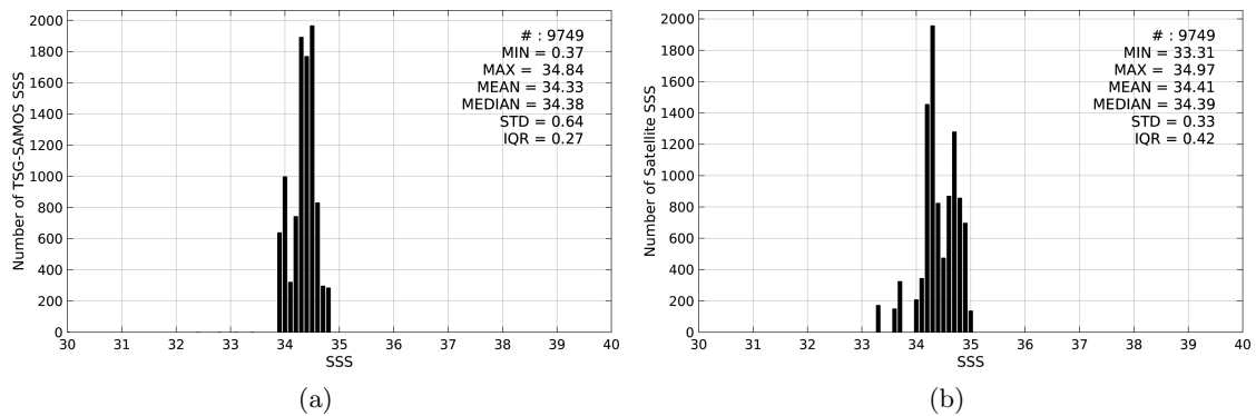
Figure 2: Histograms of SSS from TSG-SAMOS (a) and SMOS-L3-CATDS-CECOS-IFREMER-V2-1DAY-0.5DEG (b) considering all match-up pairs per bins of 0.1 over the SPURS 2 Pi-MEP region and for the full satellite product period.
