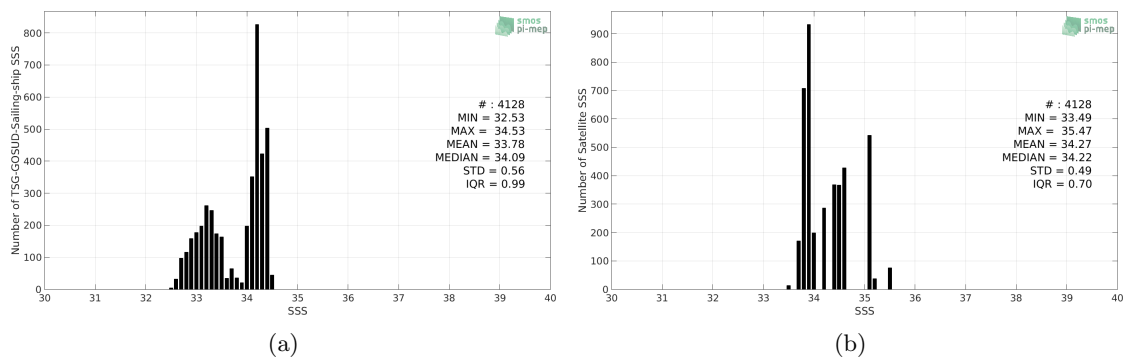
Figure 2: Histograms of SSS from TSG-GOSUD-Sailing-ship (a) and SMOS L3 v2 - Daily - 0.5 Deg (CATDS-CECOS-IFREMER) (b) considering all match-up pairs per bins of 0.1 over the SPURS 2 Pi-MEP region and for the full satellite product period.
