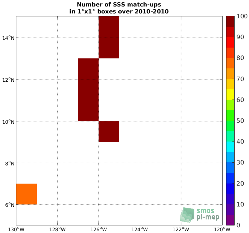
Figure 4: Number of SSS match-ups between TSG-GOSUD-Sailing-ship SSS and the SMOS L3 v2 - Daily - 0.5 Deg (CATDS-CECOS-IFREMER) SSS product for the SPURS 2 Pi-MEP region over 1°x1° boxes and for the full satellite product period.
