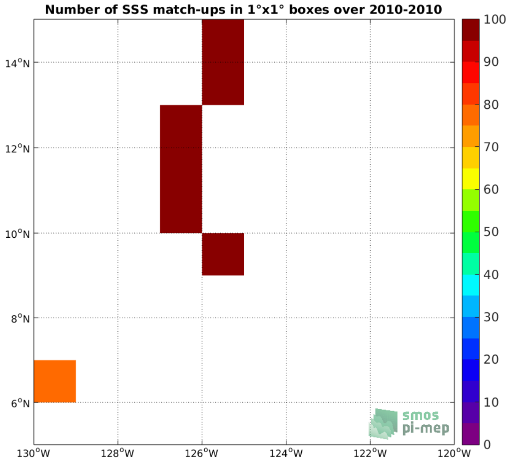
Figure 4: Number of SSS match-ups between TSG-GOSUD-Sailing-ship SSS and the SMOS-L3-CATDS-CECOS-IFREMER-V2-1DAY-0.5DEG SSS product for the SPURS 2 Pi-MEP region over 1°x1° boxes and for the full satellite product period.
