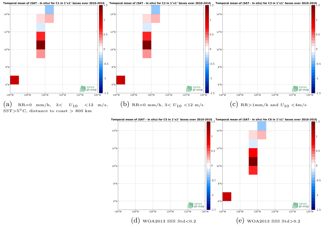
Figure 12: Temporal mean gridded over spatial boxes of size 1^\circ \times 1^\circ of \Delta SSS (SMOS-L3-CATDS-CECOS-IFREMER-V2-1DAY-0.5DEG - TSG-GOSUD-Sailing-ship) for 5 different subdatasets corresponding to:RR=0 mm/h, 3 < U_{10} < 12 m/s, SST >5^\circ C, distance to coast > 800 km (a), RR=0 mm/h, 3 < U_{10} < 12 m/s (b), RR >1 mm/h and U_{10} < 4 m/s (c), WOA2013 SSS Std <0.2 (d), WOA2013 SSS Std >0.2 (e).
