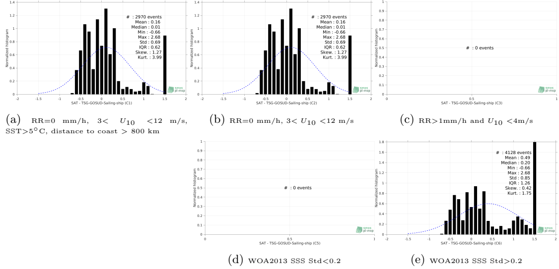
Figure 13: Normalized histogram of \Delta SSS (SMOS-L3-CATDS-CECOS-IFREMER-V2-1DAY-0.5DEG - TSG-GOSUD-Sailing-ship) for 5 different subdatasets corresponding to: RR=0 mm/h, 3 < U_{10} < 12 m/s, SST > 5°C, distance to coast > 800 km (a), RR=0 mm/h, 3 < U_{10} < 12 m/s (b), RR > 1mm/h and U_{10} < 4 m/s (c), WOA2013 SSS Std < 0.2 (d), WOA2013 SSS Std > 0.2 (e).
