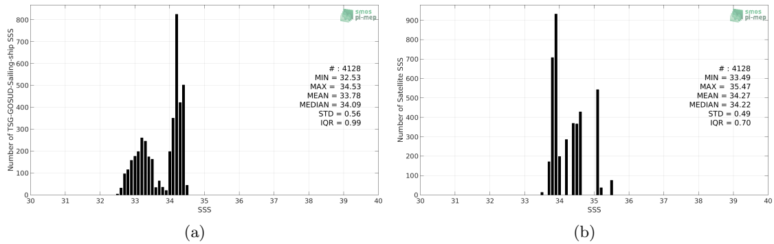
Figure 2: Histograms of SSS from TSG-GOSUD-Sailing-ship (a) and SMOS-L3-CATDS-CECOS-IFREMER-V2-1DAY-0.5DEG (b) considering all match-up pairs per bins of 0.1 over the SPURS 2 Pi-MEP region and for the full satellite product period.
