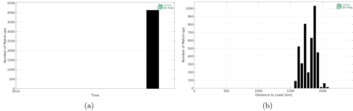
Figure 1: Number of match-ups between TSG-GOSUD-Sailing-ship and SMOS-L3-CATDS-CECOS-IFREMER-V2-1DAY-0.5DEG SSS as a function of time (a) and as function of the distance to coast (b) over the SPURS 2 Pi-MEP region and for the full satellite product period.
