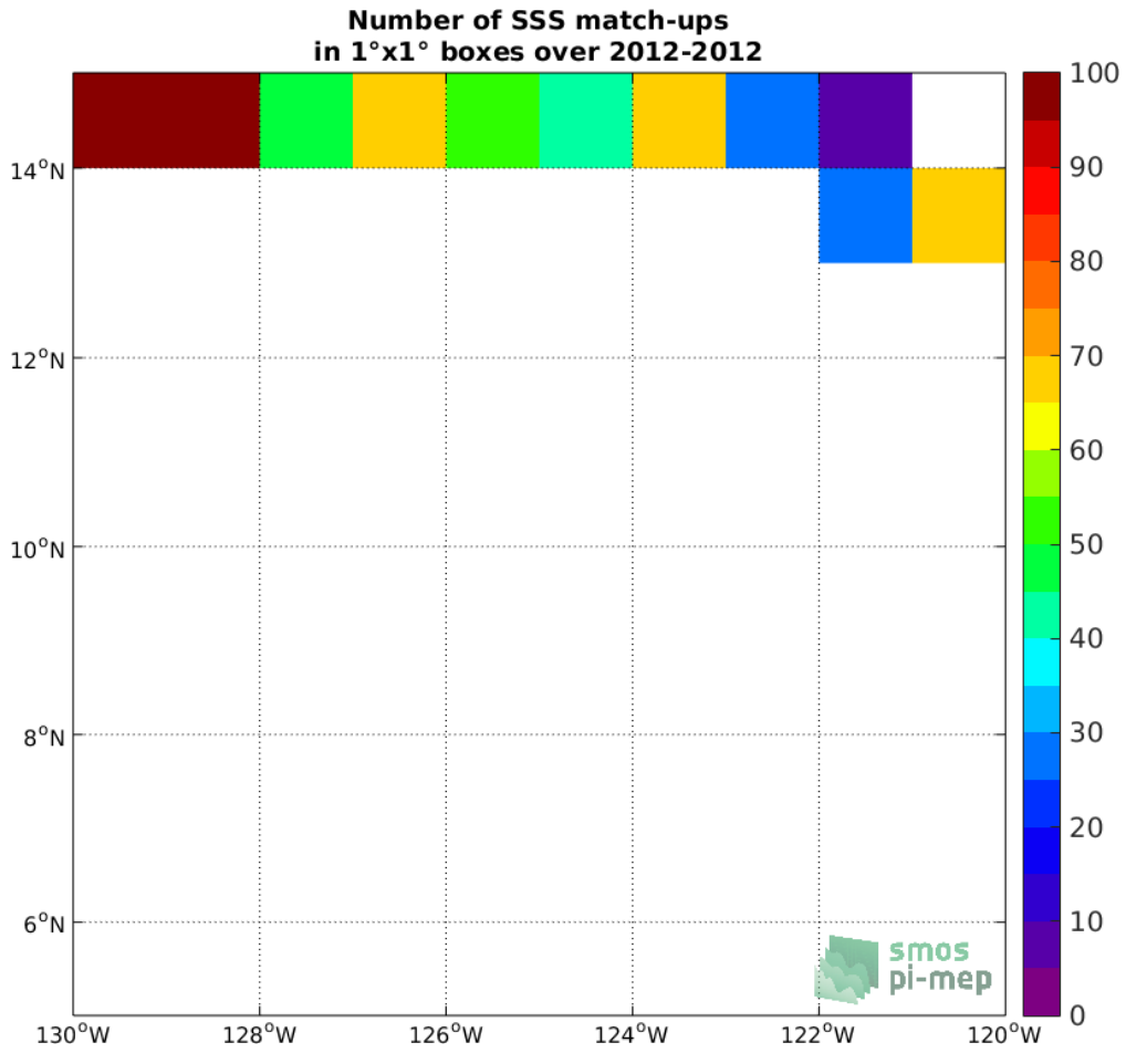
Figure 4: Number of SSS match-ups between TSG-GOSUD-Research-vessel SSS and the SMOS-L3-CATDS-CECOS-IFREMER-V2-1DAY-0.5DEG SSS product for the SPURS 2 Pi-MEP region over 1°x1° boxes and for the full satellite product period.
