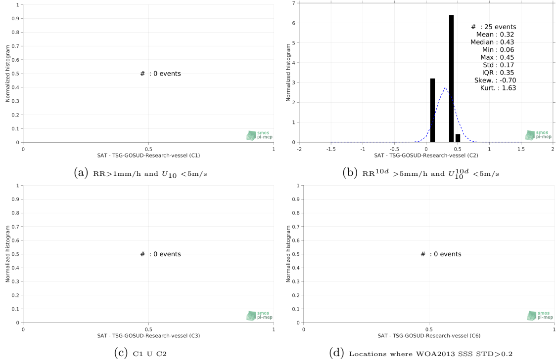
Figure 13: Normalized histogram of \Delta\text{SSS} (SMOS-L3-CATDS-CECOS-IFREMER-V2-1DAY-0.5DEG - TSG-GOSUD-Research-vessel) for 6 different subdatasets corresponding to: RR > 1\text{mm/h} and U_{10} < 5\text{m/s} (a), RR^{10d} > 5\text{mm/h} and U_{10}^{10d} < 5\text{m/s} (b), C1 U C2 (c), Locations where WOA2013 SSS STD > 0.2 (d).
