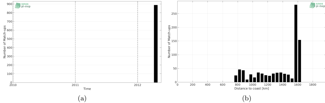
Figure 1: Number of match-ups between TSG-GOSUD-Research-vessel and SMOS-L3-CATDS-CECOS-IFREMER-V2-1DAY-0.5DEG SSS as a function of time (a) and as function of the distance to coast (b) over the SPURS 2 Pi-MEP region and for the full satellite product period.
