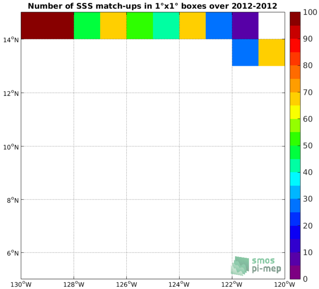
Figure 4: Number of SSS match-ups between TSG-GOSUD-Research-vessel SSS and the SMOS-L3-CATDS-CECOS-IFREMER-V2-1DAY-0.5DEG SSS product for the SPURS 2 Pi-MEP region over 1°x1° boxes and for the full satellite product period.
