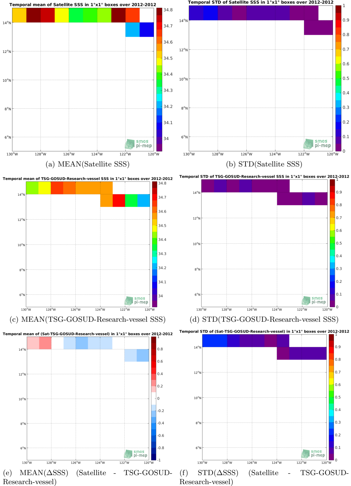
Figure 6: Temporal mean (left) and STD (right) of SSS from SMOS-L3-CATDS-CECOS-IFREMER-V2-1DAY-0.5DEG (top), TSG-GOSUD-Research-vessel (middle), and of \Delta SSS (Satellite - TSG-GOSUD-Research-vessel). Only match-up pairs are used to generate these maps.
