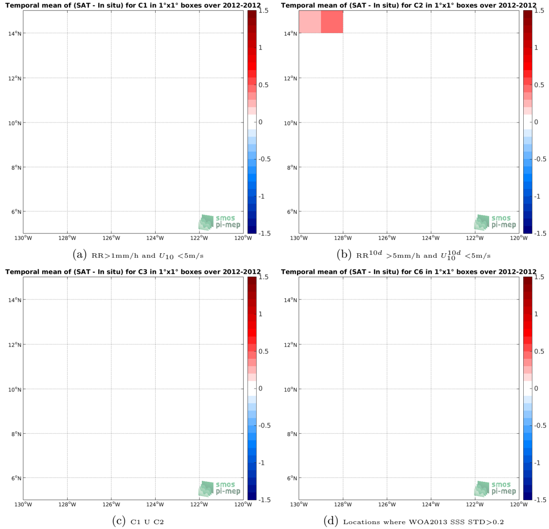
Figure 12: Temporal mean gridded over spatial boxes of size 1^\circ \times 1^\circ of \Delta SSS (SMOS-L3-CATDS-CECOS-IFREMER-V2-1DAY-0.5DEG - TSG-GOSUD-Research-vessel) for 4 different subdatasets corresponding to: RR > 1\text{mm/h} and U_{10} < 5\text{m/s} (a), RR^{10d} > 5\text{mm/h} and U_{10}^{10d} < 5\text{m/s} (b), C1 U C2 (c), Locations where WOA2013 SSS STD > 0.2 (d).
