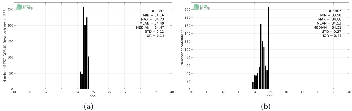
Figure 2: Histograms of SSS from TSG-GOSUD-Research-vessel (a) and SMOS-L3-CATDS-CECOS-IFREMER-V2-1DAY-0.5DEG (b) considering all match-up pairs per bins of 0.1 over the SPURS 2 Pi-MEP region and for the full satellite product period.
