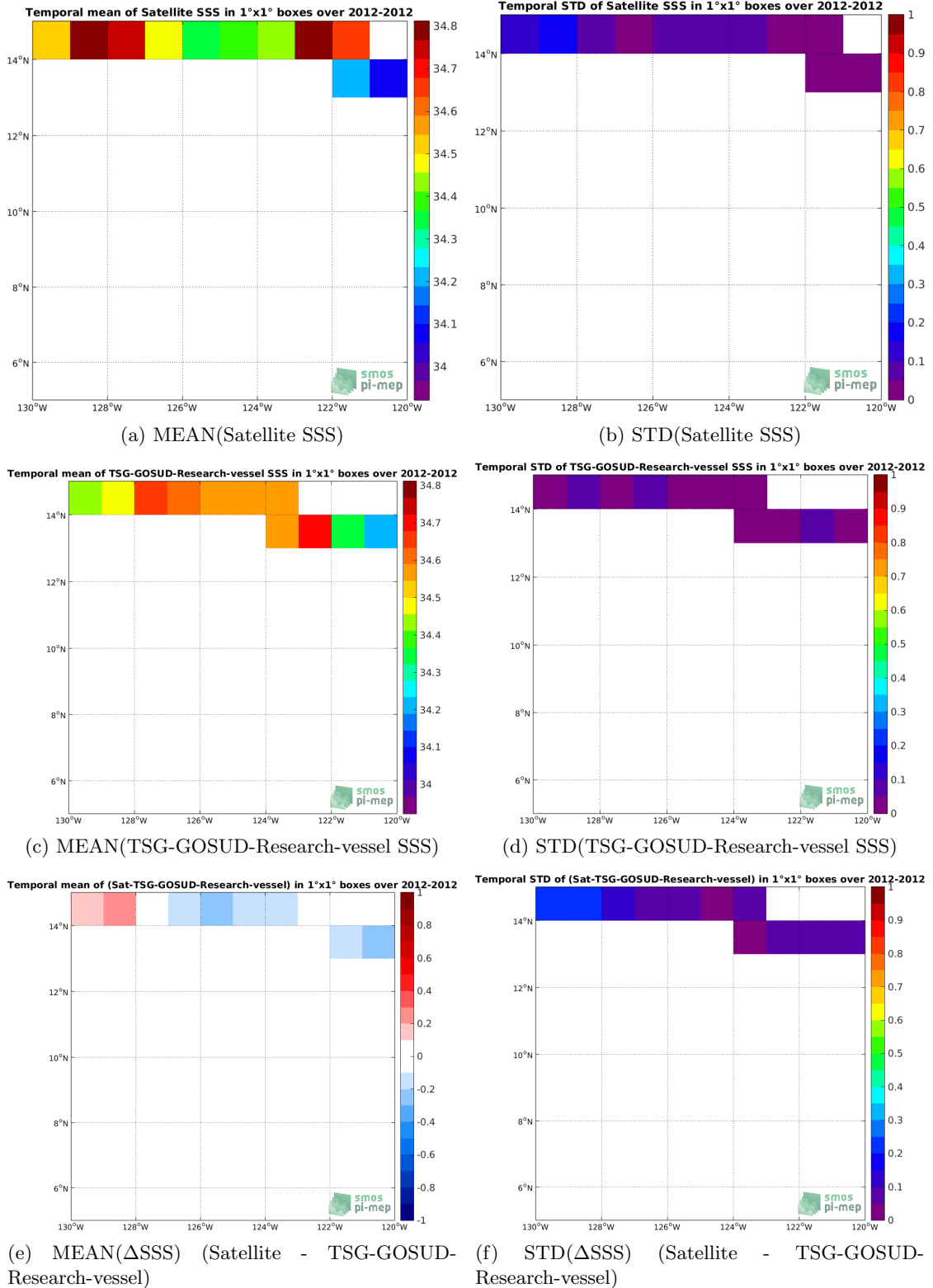
Figure 6: Temporal mean (left) and STD (right) of SSS from SMOS-L3-CATDS-CECOS-IFREMER-V2-1DAY-0.5DEG (top), TSG-GOSUD-Research-vessel (middle), and of \Delta SSS (Satellite - TSG-GOSUD-Research-vessel). Only match-up pairs are used to generate these maps.
