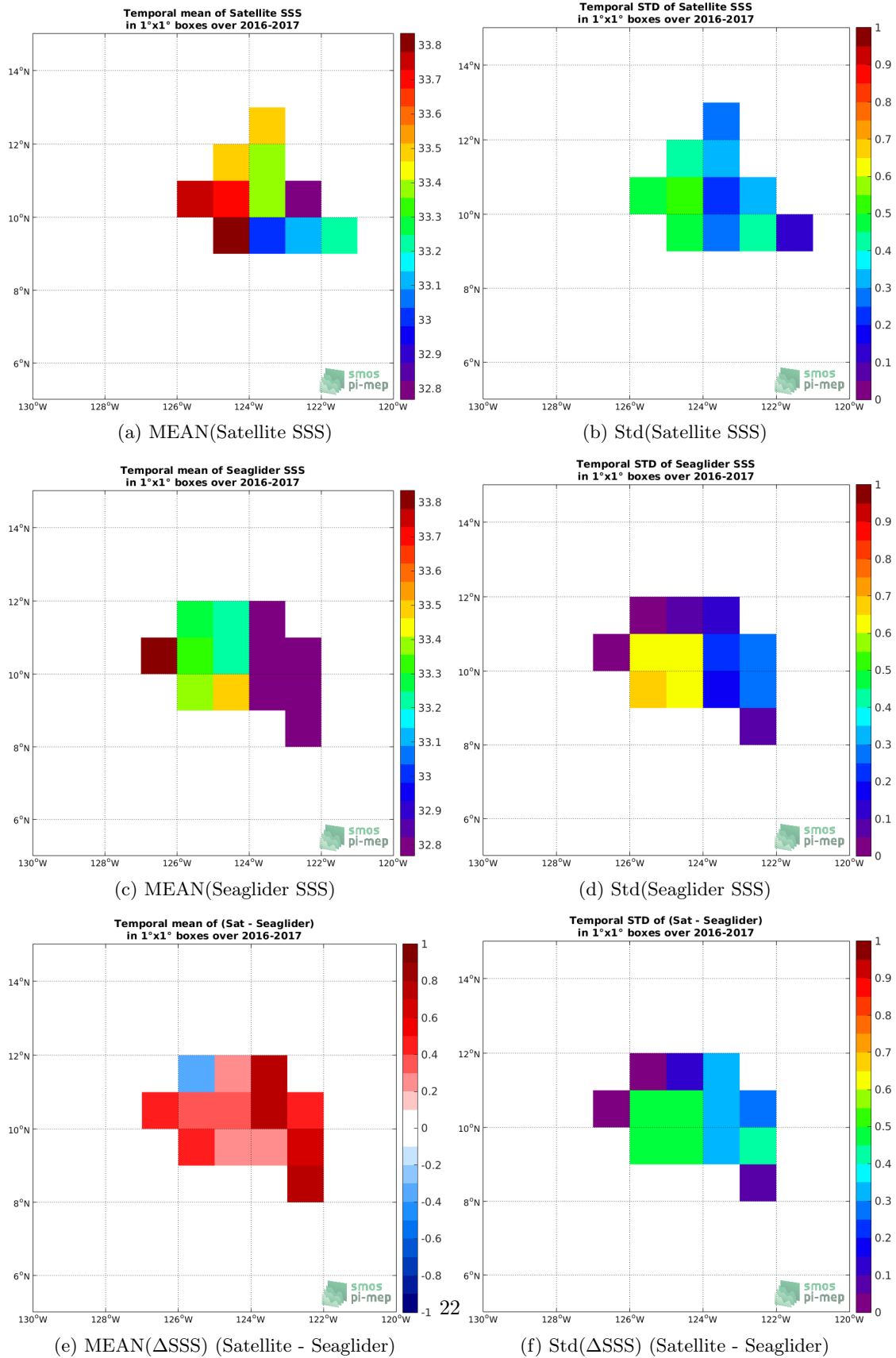
Figure 6: Temporal mean (left) and Std (right) of SSS from SMOS SSS L3 v2 - Daily - 0.5 Deg (CATDS-CECOS-IFREMER) (top), Seaglider (middle), and of \Delta SSS (Satellite - Seaglider). Only match-up pairs are used to generate these maps.
