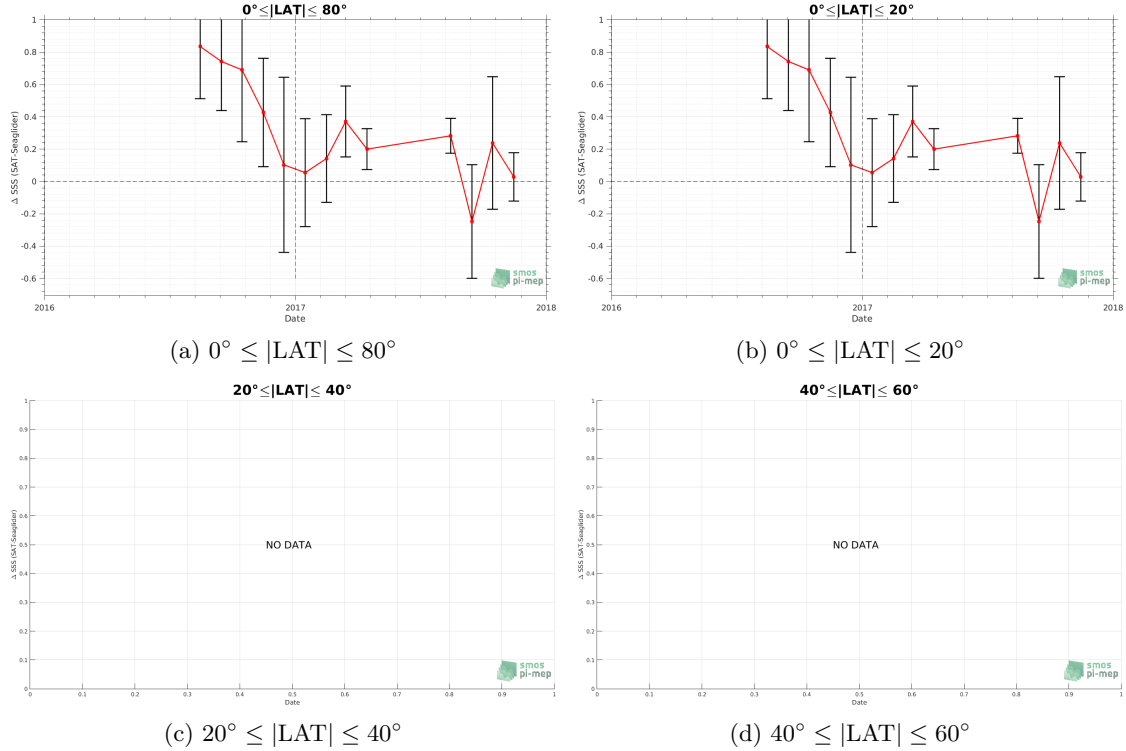
Figure 10: Monthly median (red curves) of \Delta SSS (Satellite - Seaglider) and \pm 1 Std (black vertical thick bars) as function of time for all the collected Pi-MEP match-up pairs estimated over the SPURS 2 Pi-MEP region and for the full satellite product period are shown for different latitude bands: (a) 80^\circ\text{S}-80^\circ\text{N} , (b) 20^\circ\text{S}-20^\circ\text{N} , (c) 40^\circ\text{S}-20^\circ\text{S} and 20^\circ\text{N}-40^\circ\text{N} and (d) 60^\circ\text{S}-40^\circ\text{S} and 40^\circ\text{N}-60^\circ\text{N} .
