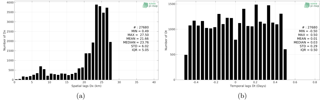
Figure 5: Histograms of the spatial (a) and temporal (b) lags between the time of the Seaglider measurements and the date of the corresponding SMOS SSS L3 v2 - Daily - 0.5 Deg (CATDS-CECOS-IFREMER) SSS product.
