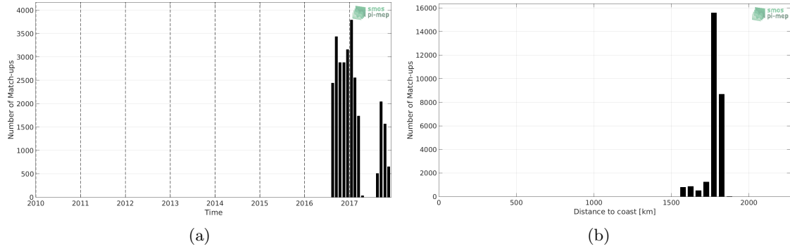
Figure 1: Number of match-ups between Seaglider and SMOS SSS L3 v2 - Daily - 0.5 Deg (CATDS-CECOS-IFREMER) SSS as a function of time (a) and as function of the distance to coast (b) over the SPURS 2 Pi-MEP region and for the full satellite product period.
