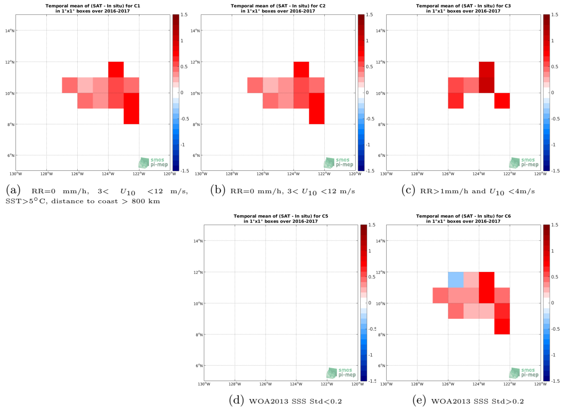
Figure 12: Temporal mean gridded over spatial boxes of size 1^{\circ}\times 1^{\circ} of \Delta\text{SSS} (SMOS SSS L3 v2 - Daily - 0.5 Deg (CATDS-CECOS-IFREMER) - Seaglider) for 5 different subdatasets corresponding to:RR=0 mm/h, 3 < U_{10} < 12 m/s, SST >5^{\circ}\text{C} , distance to coast > 800 km (a), RR=0 mm/h, 3 < U_{10} < 12 m/s (b), RR >1 mm/h and U_{10} < 4 m/s (c), WOA2013 SSS Std <0.2 (d), WOA2013 SSS Std >0.2 (e).
