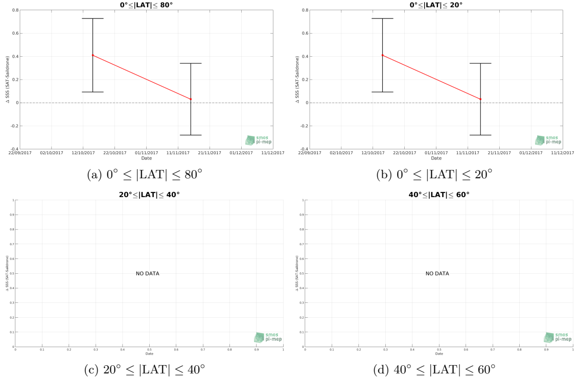
Figure 10: Monthly median (red curves) of \Delta SSS (Satellite - Sairdrone) and \pm 1 Std (black vertical thick bars) as function of time for all the collected Pi-MEP match-up pairs estimated over the SPURS 2 Pi-MEP region and for the full satellite product period are shown for different latitude bands: (a) 80^{\circ}\text{S}-80^{\circ}\text{N} , (b) 20^{\circ}\text{S}-20^{\circ}\text{N} , (c) 40^{\circ}\text{S}-20^{\circ}\text{S} and 20^{\circ}\text{N}-40^{\circ}\text{N} and (d) 60^{\circ}\text{S}-40^{\circ}\text{S} and 40^{\circ}\text{N}-60^{\circ}\text{N} .
