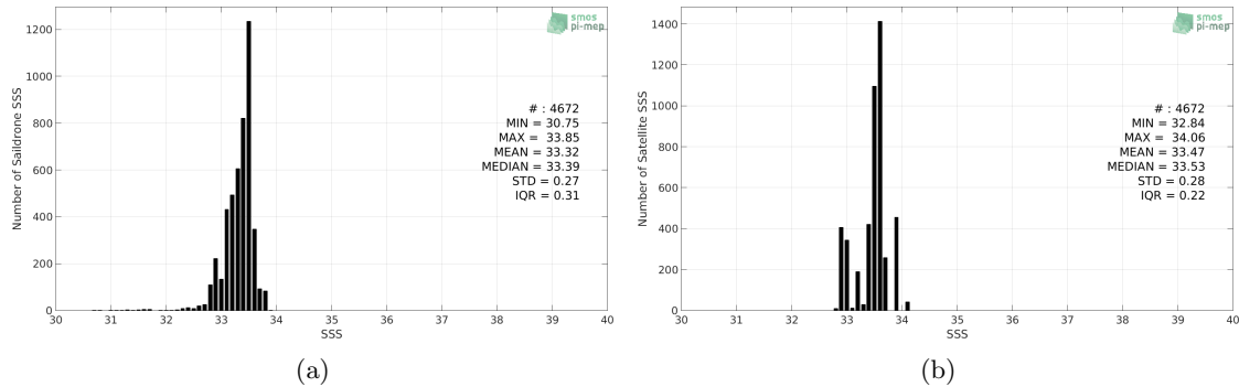
Figure 2: Histograms of SSS from Saildrone (a) and SMOS SSS L3 v2 - Daily - 0.5 Deg (CATDS-CECOS-IFREMER) (b) considering all match-up pairs per bins of 0.1 over the SPURS 2 Pi-MEP region and for the full satellite product period.
