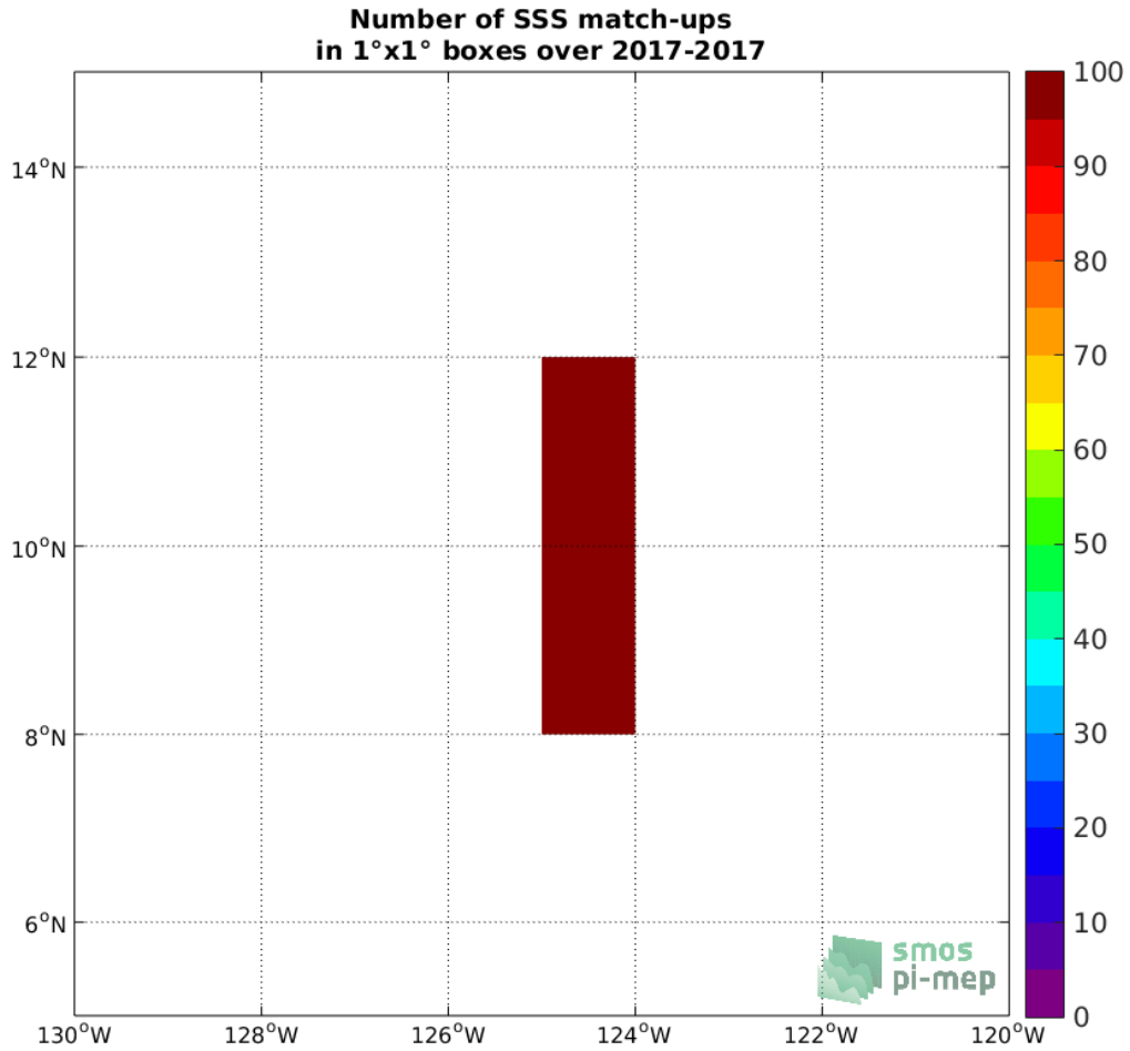
Figure 4: Number of SSS match-ups between Saildrone SSS and the SMOS SSS L3 v2 - Daily - 0.5 Deg (CATDS-CECOS-IFREMER) SSS product for the SPURS 2 Pi-MEP region over 1°x1° boxes and for the full satellite product period.
