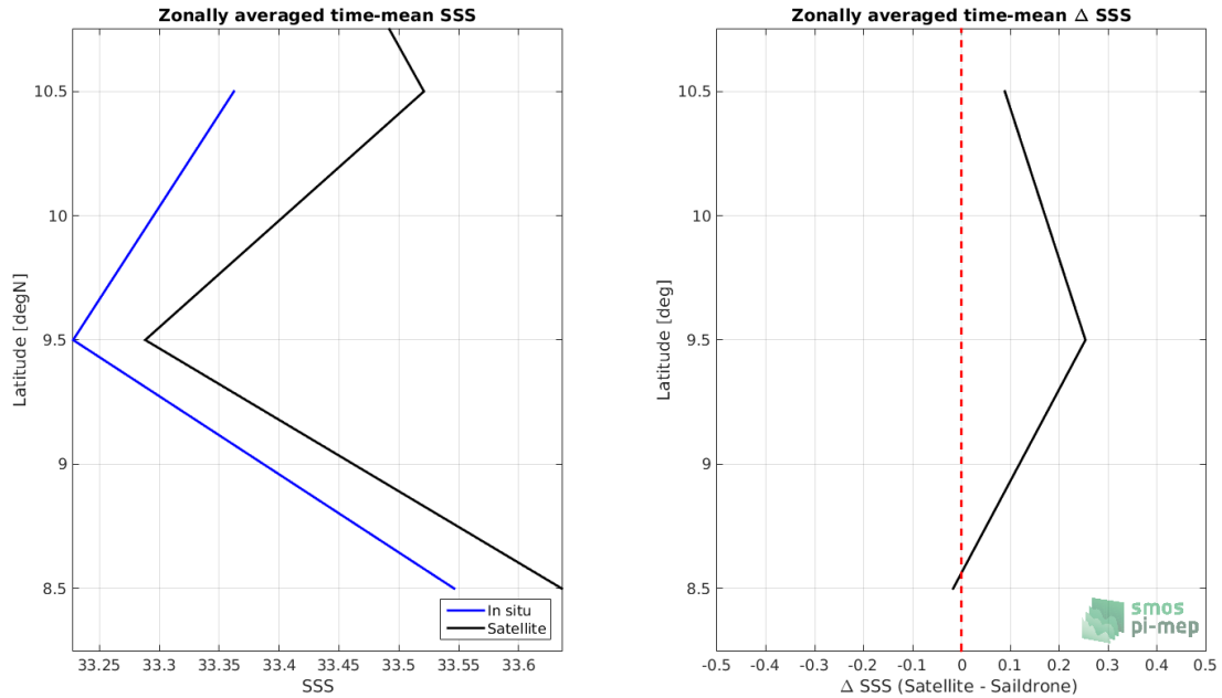
Figure 8: Left panel: Zonal mean SSS from SMOS SSS L3 v2 - Daily - 0.5 Deg (CATDS-CECOS-IFREMER) satellite product (black) and from Sairdrone (blue). Right panel: Zonal mean of \Delta SSS (Satellite - Sairdrone) for all the collected Pi-MEP match-up pairs estimated over the full satellite product period.
