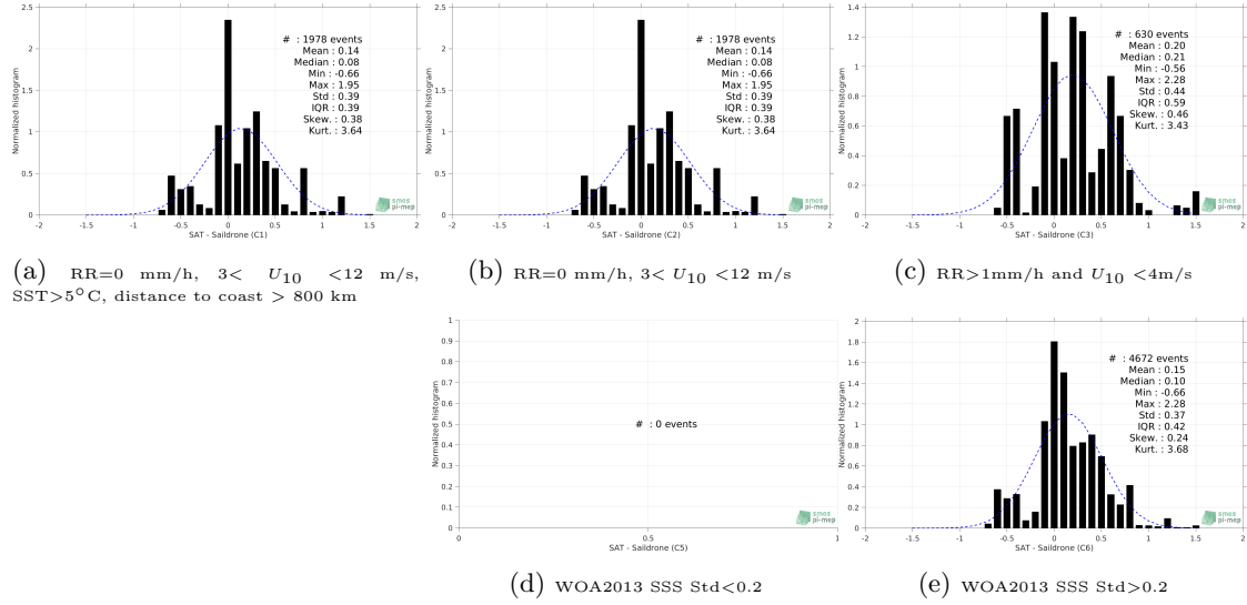
Figure 13: Normalized histogram of \Delta\text{SSS} (SMOS SSS L3 v2 - Daily - 0.5 Deg (CATDS-CECOS-IFREMER) - Saildrone) for 5 different subdatasets corresponding to: RR=0 mm/h, 3 < U_{10} < 12 m/s, SST > 5^\circ\text{C} , distance to coast > 800 km (a), RR=0 mm/h, 3 < U_{10} < 12 m/s (b), RR > 1\text{mm/h} and U_{10} < 4\text{m/s} (c), WOA2013 SSS Std < 0.2 (d), WOA2013 SSS Std > 0.2 (e).
