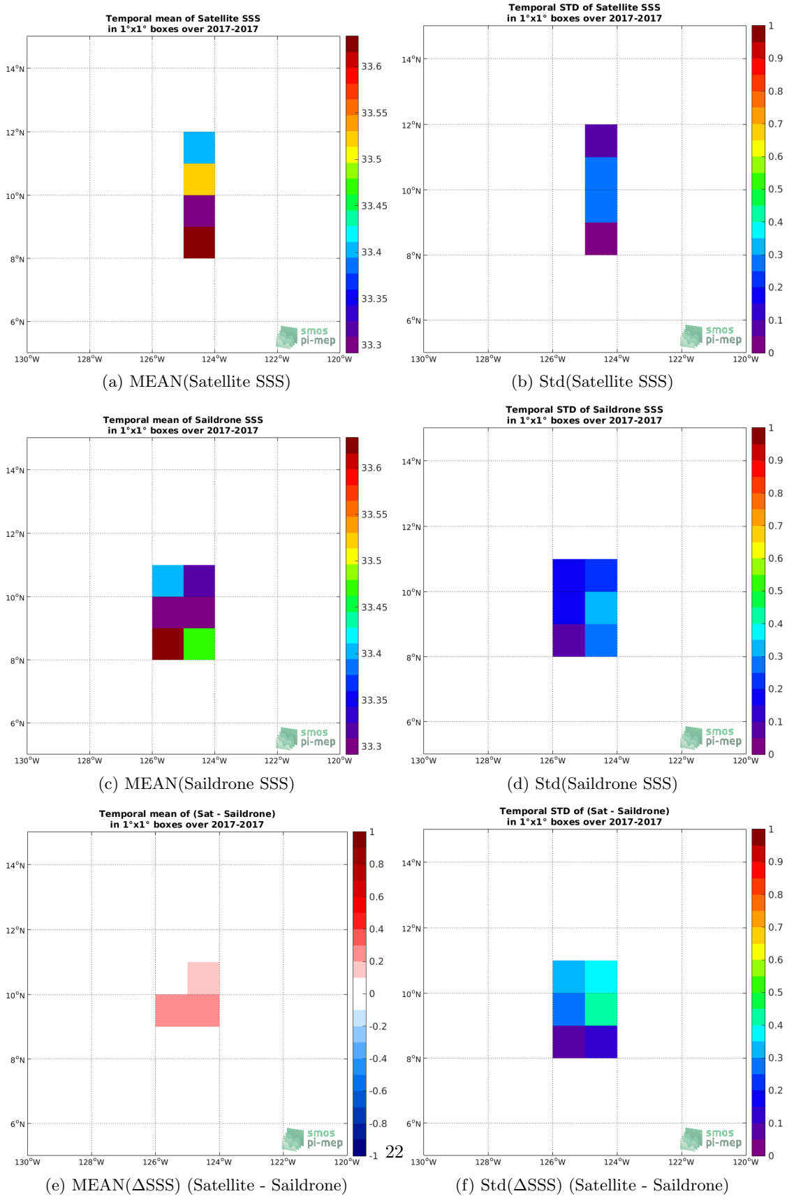
Figure 6: Temporal mean (left) and Std (right) of SSS from SMOS SSS L3 v2 - Daily - 0.5 Deg (CATDS-CECOS-IFREMER) (top), Saildrone (middle), and of \Delta SSS (Satellite - Saildrone). Only match-up pairs are used to generate these maps.
