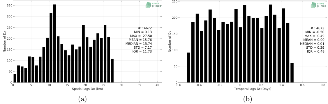
Figure 5: Histograms of the spatial (a) and temporal (b) lags between the time of the Saildrone measurements and the date of the corresponding SMOS SSS L3 v2 - Daily - 0.5 Deg (CATDS-CECOS-IFREMER) SSS product.
