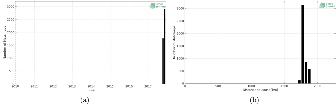
Figure 1: Number of match-ups between Saildrone and SMOS SSS L3 v2 - Daily - 0.5 Deg (CATDS-CECOS-IFREMER) SSS as a function of time (a) and as function of the distance to coast (b) over the SPURS 2 Pi-MEP region and for the full satellite product period.
