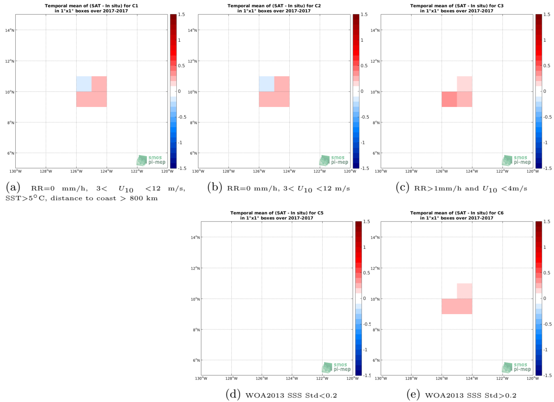
Figure 12: Temporal mean gridded over spatial boxes of size 1^{\circ}\times 1^{\circ} of \Delta\text{SSS} (SMOS SSS L3 v2 - Daily - 0.5 Deg (CATDS-CECOS-IFREMER) - Saifdrone) for 5 different subdatasets corresponding to:RR=0 mm/h, 3 < U_{10} < 12 m/s, SST >5^{\circ}\text{C} , distance to coast > 800 km (a), RR=0 mm/h, 3 < U_{10} < 12 m/s (b), RR >1 mm/h and U_{10} < 4 m/s (c), WOA2013 SSS Std <0.2 (d), WOA2013 SSS Std >0.2 (e).
