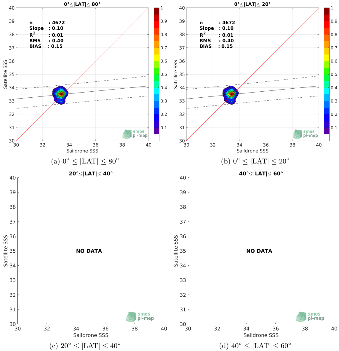
Figure 9: Contour maps of the concentration of SMOS SSS L3 v2 - Daily - 0.5 Deg (CATDS-CECOS-IFREMER) SSS (y-axis) versus Saildrone SSS (x-axis) at match-up pairs for different latitude bands. For each plot, the red line shows x=y . The black thin and dashed lines indicate a linear fit through the data cloud and the \pm 95\% confidence levels, respectively. The number match-up pairs n , the slope and R^2 coefficient of the linear fit, the root mean square (RMS) and the mean bias between satellite and in situ data are indicated for each latitude band in each plots.
