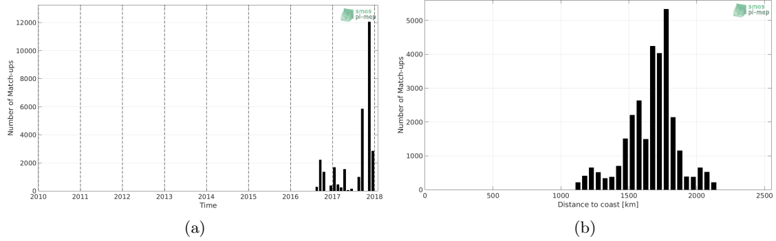
Figure 1: Number of match-ups between Surface drifters and SMOS SSS L3 v2 - Daily - 0.5 Deg (CATDS-CECOS-IFREMER) SSS as a function of time (a) and as function of the distance to coast (b) over the SPURS 2 Pi-MEP region and for the full satellite product period.
