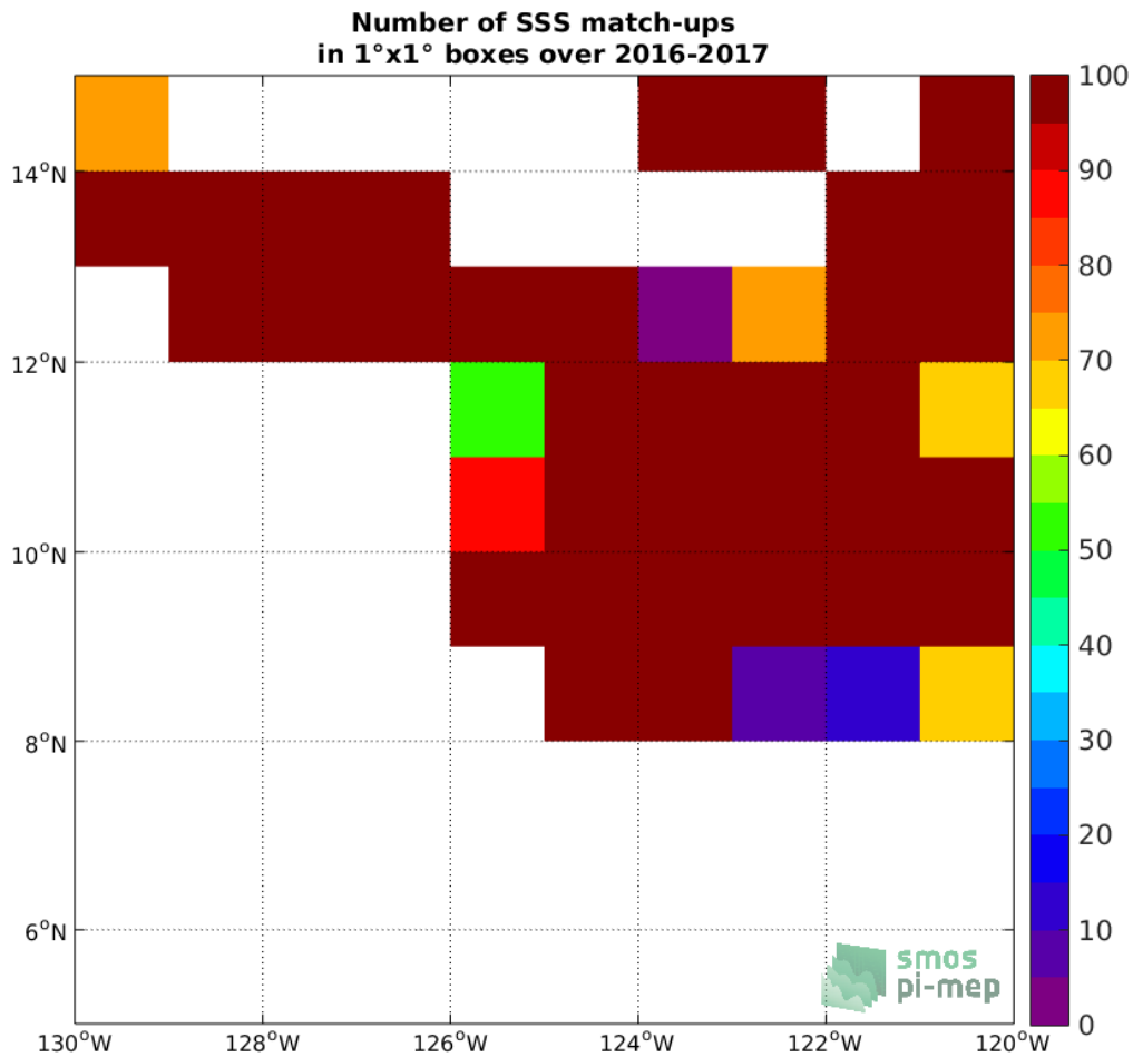
Figure 3: Number of SSS match-ups between Surface drifters SSS and the SMOS SSS L3 v2 - Daily - 0.5 Deg (CATDS-CECOS-IFREMER) SSS product for the SPURS 2 Pi-MEP region over 1°x1° boxes and for the full satellite product period.
