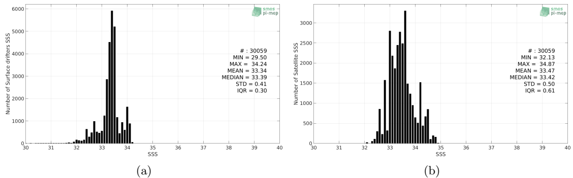
Figure 2: Histograms of SSS from Surface drifters (a) and SMOS SSS L3 v2 - Daily - 0.5 Deg (CATDS-CECOS-IFREMER) (b) considering all match-up pairs per bins of 0.1 over the SPURS 2 Pi-MEP region and for the full satellite product period.
