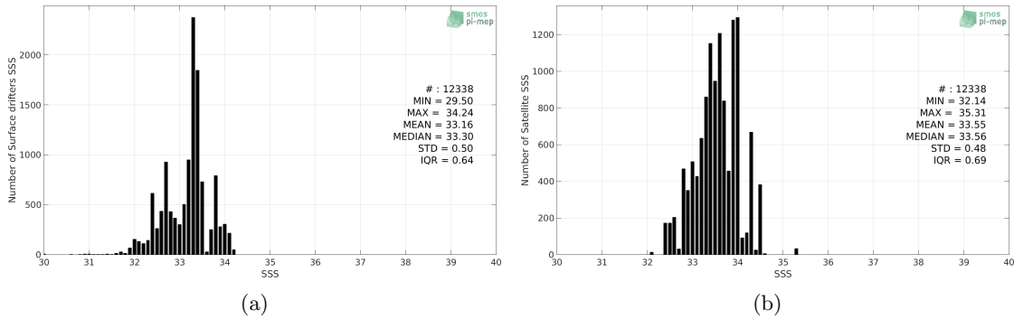
Figure 2: Histograms of SSS from Surface drifters (a) and SMOS-L3-CATDS-CECOS-IFREMER-V2-1DAY-0.5DEG (b) considering all match-up pairs per bins of 0.1 over the SPURS 2 Pi-MEP region and for the full satellite product period.
