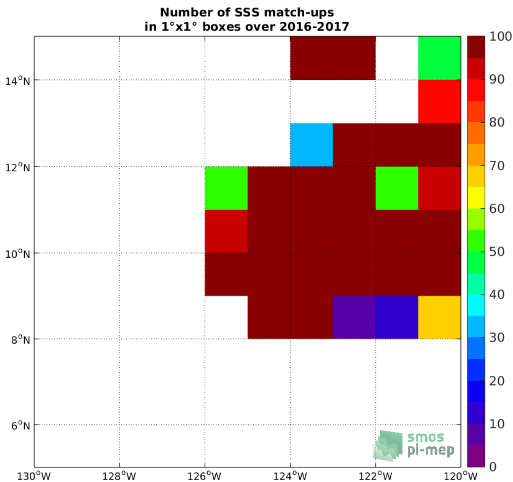
Figure 3: Number of SSS match-ups between Surface drifters SSS and the SMOS-L3-CATDS-CECOS-IFREMER-V2-1DAY-0.5DEG SSS product for the SPURS 2 Pi-MEP region over 1°x1° boxes and for the full satellite product period.
