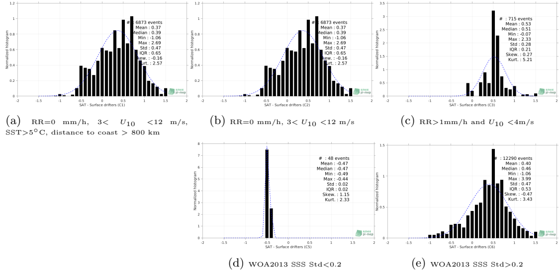
Figure 12: Normalized histogram of \Delta SSS (SMOS-L3-CATDS-CECOS-IFREMER-V2-1DAY-0.5DEG - Surface drifters) for 5 different subdatasets corresponding to: RR=0 mm/h, 3 < U_{10} < 12 m/s, SST > 5°C, distance to coast > 800 km (a), RR=0 mm/h, 3 < U_{10} < 12 m/s (b), RR > 1mm/h and U_{10} < 4 m/s (c), WOA2013 SSS Std < 0.2 (d), WOA2013 SSS Std > 0.2 (e).
