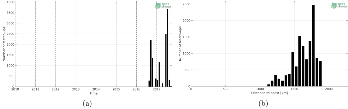
Figure 1: Number of match-ups between Surface drifters and SMOS-L3-CATDS-CECOS-IFREMER-V2-1DAY-0.5DEG SSS as a function of time (a) and as function of the distance to coast (b) over the SPURS 2 Pi-MEP region and for the full satellite product period.
