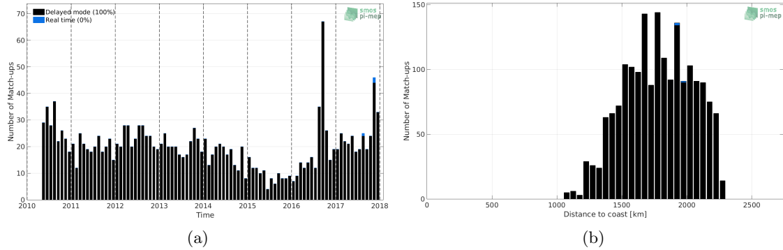
Figure 1: Number of match-ups between Argo and SMOS SSS L3 v2 - Daily - 0.5 Deg (CATDS-CECOS-IFREMER) SSS as a function of time (a) and as function of the distance to coast (b) over the SPURS 2 Pi-MEP region and for the full satellite product period.
