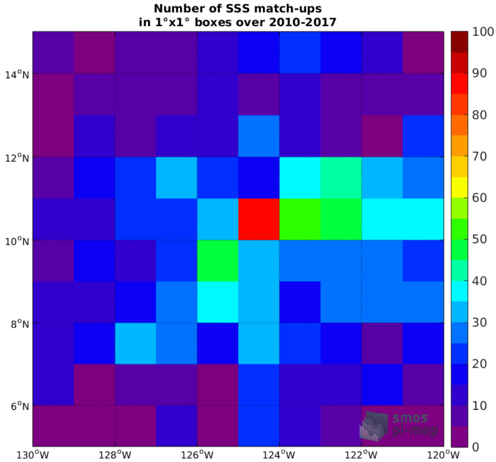
Figure 4: Number of SSS match-ups between Argo SSS and the SMOS SSS L3 v2 - Daily - 0.5 Deg (CATDS-CECOS-IFREMER) SSS product for the SPURS 2 Pi-MEP region over 1°x1° boxes and for the full satellite product period.
