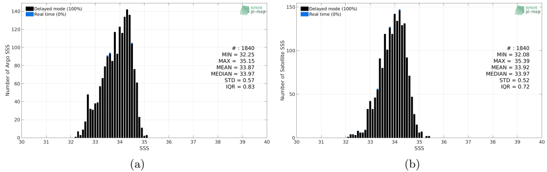
Figure 2: Histograms of SSS from Argo (a) and SMOS SSS L3 v2 - Daily - 0.5 Deg (CATDS-CECOS-IFREMER) (b) considering all match-up pairs per bins of 0.1 over the SPURS 2 Pi-MEP region and for the full satellite product period.
