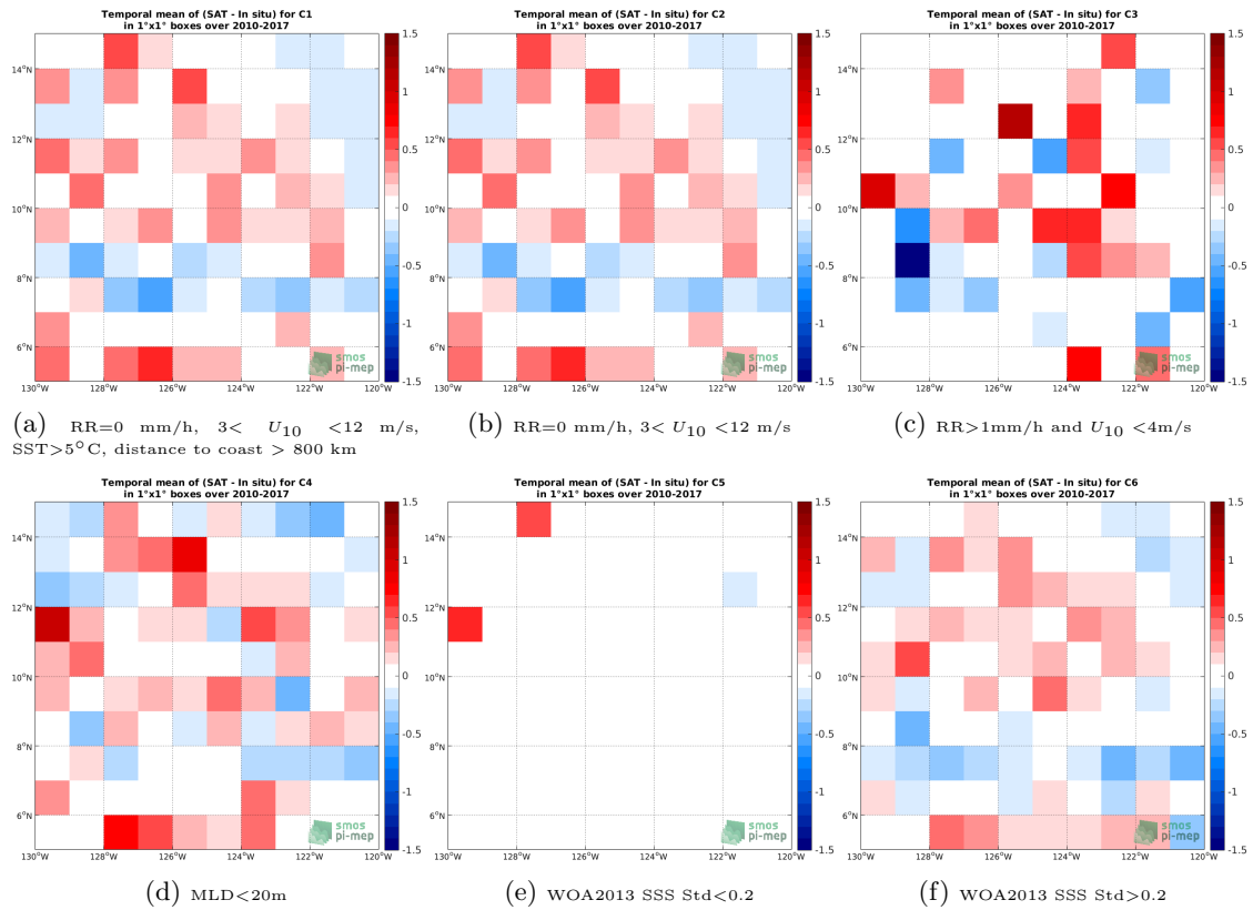
Figure 12: Temporal mean gridded over spatial boxes of size 1^\circ \times 1^\circ of \Delta SSS (SMOS SSS L3 v2 - Daily - 0.5 Deg (CATDS-CECOS-IFREMER) - Argo) for 6 different subdatasets corresponding to:RR=0 mm/h, 3 < U_{10} < 12 m/s, SST >5^\circ C, distance to coast > 800 km (a), RR=0 mm/h, 3 < U_{10} < 12 m/s (b), RR >1 mm/h and U_{10} < 4 m/s (c),MLD <20 m (d),WOA2013 SSS Std <0.2 (e),WOA2013 SSS Std >0.2 (f).
