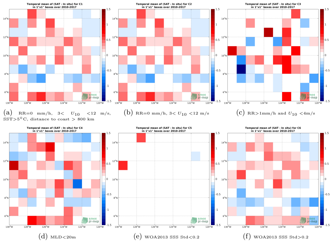
Figure 12: Temporal mean gridded over spatial boxes of size 1^\circ \times 1^\circ of \Delta SSS (SMOS L3 v2 - Daily - 0.5 Deg (CATDS-CECOS-IFREMER) - Argo) for 6 different subdatasets corresponding to:RR=0 mm/h, 3 < U_{10} < 12 m/s, SST >5^\circ C, distance to coast > 800 km (a), RR=0 mm/h, 3 < U_{10} < 12 m/s (b), RR >1 mm/h and U_{10} < 4 m/s (c),MLD <20 m (d),WOA2013 SSS Std <0.2 (e),WOA2013 SSS Std >0.2 (f).
