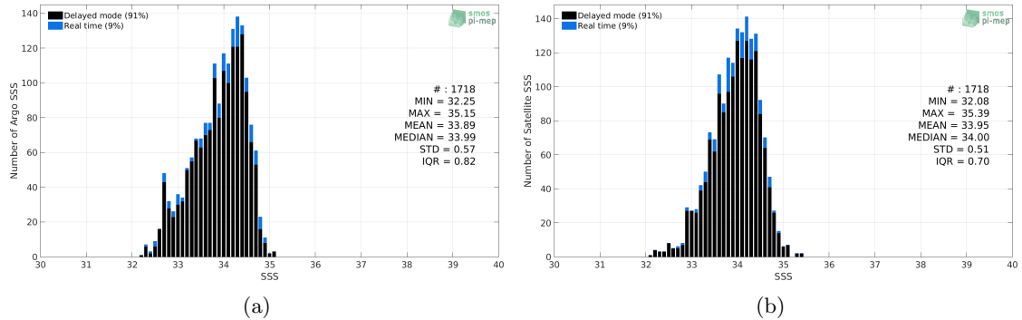
Figure 2: Histograms of SSS from Argo (a) and SMOS L3 v2 - Daily - 0.5 Deg (CATDS-CECOS-IFREMER) (b) considering all match-up pairs per bins of 0.1 over the SPURS 2 Pi-MEP region and for the full satellite product period.
