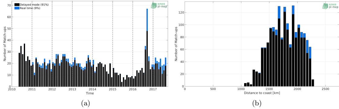
Figure 1: Number of match-ups between Argo and SMOS L3 v2 - Daily - 0.5 Deg (CATDS-CECOS-IFREMER) SSS as a function of time (a) and as function of the distance to coast (b) over the SPURS 2 Pi-MEP region and for the full satellite product period.
