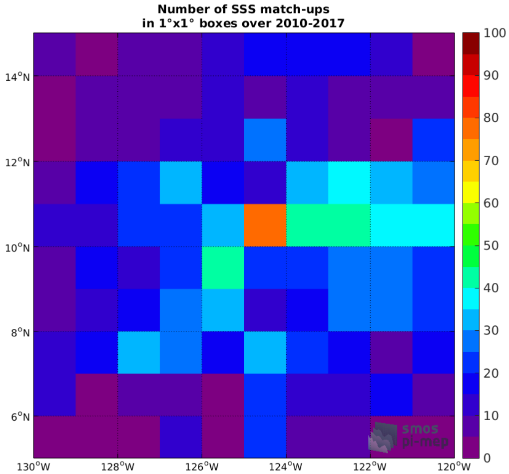
Figure 4: Number of SSS match-ups between Argo SSS and the SMOS L3 v2 - Daily - 0.5 Deg (CATDS-CECOS-IFREMER) SSS product for the SPURS 2 Pi-MEP region over 1°x1° boxes and for the full satellite product period.
