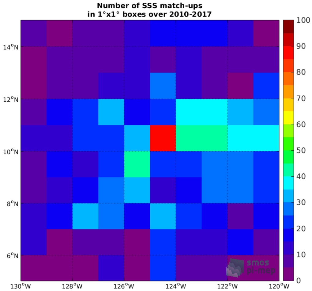
Figure 4: Number of SSS match-ups between Argo SSS and the SMOS-L3-CATDS-CECOS-IFREMER-V2-1DAY-0.5DEG SSS product for the SPURS 2 Pi-MEP region over 1°x1° boxes and for the full satellite product period.
