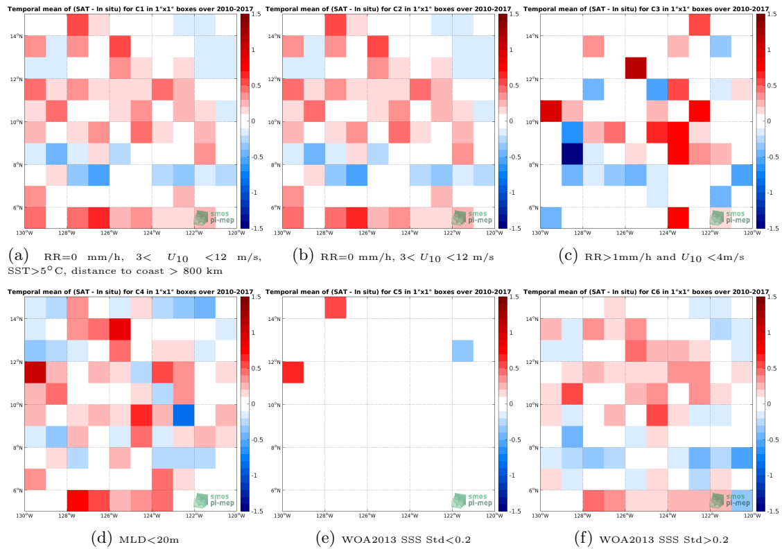
Figure 12: Temporal mean gridded over spatial boxes of size 1^\circ \times 1^\circ of \Delta SSS (SMOS-L3-CATDS-CECOS-IFREMER-V2-1DAY-0.5DEG - Argo) for 6 different subdatasets corresponding to: RR=0 mm/h, 3 < U_{10} < 12 m/s, SST > 5^\circ\text{C} , distance to coast > 800 km (a), RR=0 mm/h, 3 < U_{10} < 12 m/s (b), RR > 1 mm/h and U_{10} < 4 m/s (c), MLD < 20 m (d), WOA2013 SSS Std < 0.2 (e), WOA2013 SSS Std > 0.2 (f).
