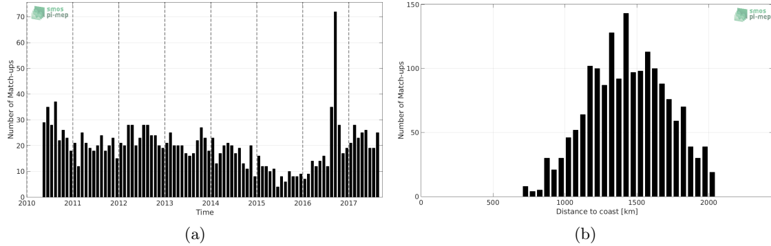
Figure 1: Number of match-ups between Argo and SMOS-L3-CATDS-CECOS-IFREMER-V2-1DAY-0.5DEG SSS as a function of time (a) and as function of the distance to coast (b) over the SPURS 2 Pi-MEP region and for the full satellite product period.
