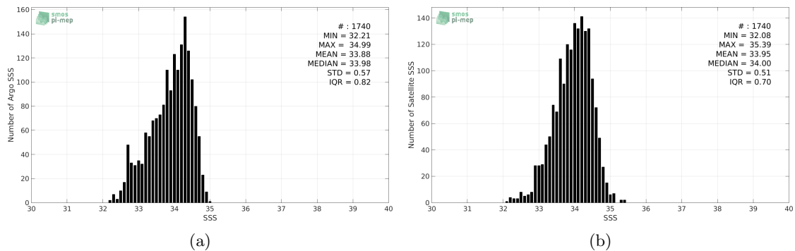
Figure 2: Histograms of SSS from Argo (a) and SMOS-L3-CATDS-CECOS-IFREMER-V2-1DAY-0.5DEG (b) considering all match-up pairs per bins of 0.1 over the SPURS 2 Pi-MEP region and for the full satellite product period.
