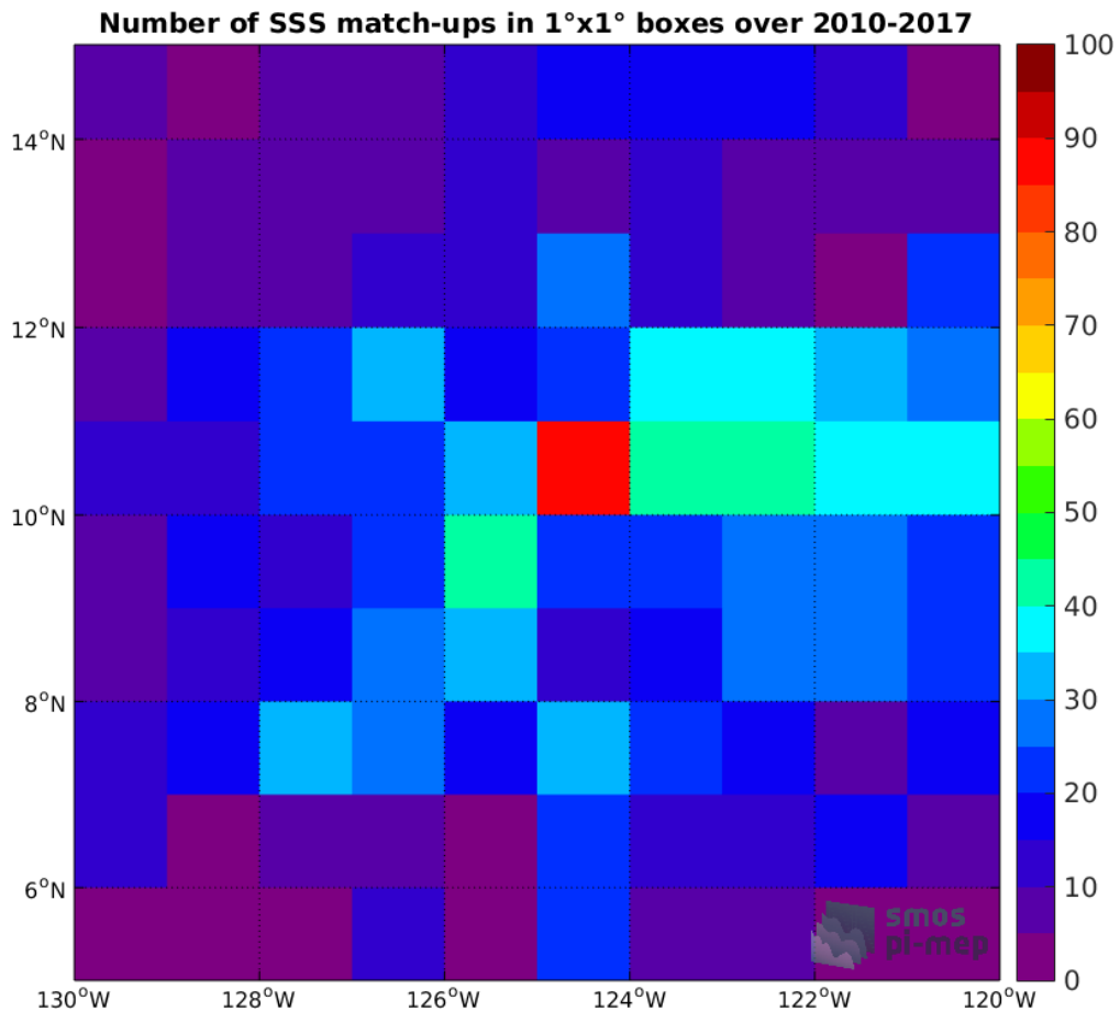
Figure 4: Number of SSS match-ups between Argo SSS and the SMOS-L3-CATDS-CECOS-IFREMER-V2-1DAY-0.5DEG SSS product for the SPURS 2 Pi-MEP region over 1°x1° boxes and for the full satellite product period.
