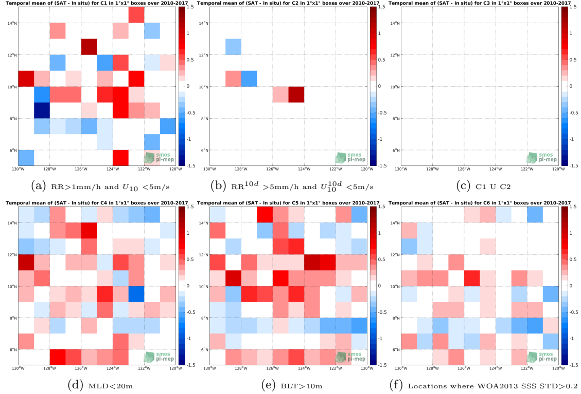
Figure 12: Temporal mean gridded over spatial boxes of size 1^\circ \times 1^\circ of \Delta\text{SSS} (SMOS-L3-CATDS-CECOS-IFREMER-V2-1DAY-0.5DEG - Argo) for 6 different subdatasets corresponding to: \text{RR} > 1\text{mm/h} and U_{10} < 5\text{m/s} (a), \text{RR}^{10d} > 5\text{mm/h} and U_{10}^{10d} < 5\text{m/s} (b), C1 U C2 (c), \text{MLD} < 20\text{m} (d), \text{BLT} > 10\text{m} (e), Locations where WOA2013 SSS STD > 0.2 (f).
