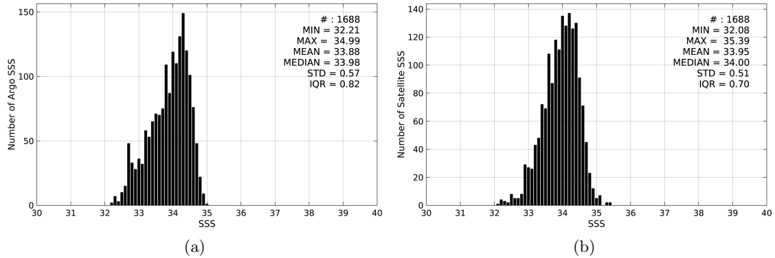
Figure 2: Histograms of SSS from Argo (a) and SMOS-L3-CATDS-CECOS-IFREMER-V2-1DAY-0.5DEG (b) considering all match-up pairs per bins of 0.1 over the SPURS 2 Pi-MEP region and for the full satellite product period.
