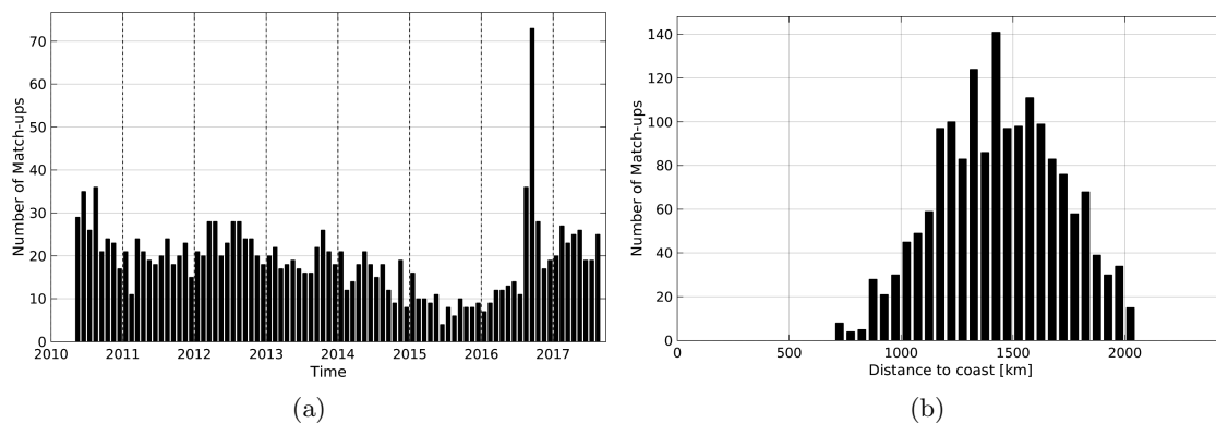
Figure 1: Number of match-ups between Argo and SMOS-L3-CATDS-CECOS-IFREMER-V2-1DAY-0.5DEG SSS as a function of time (a) and as function of the distance to coast (b) over the SPURS 2 Pi-MEP region and for the full satellite product period.
