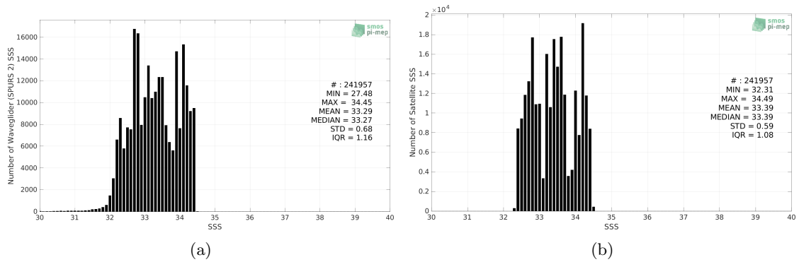
Figure 2: Histograms of SSS from Waveglider (SPURS 2) (a) and SMOS SSS L3 v335 - Monthly - 25 km (CATDS-CPDC) (b) considering all match-up pairs per bins of 0.1 over the SPURS 2 Pi-MEP region and for the full satellite product period.
