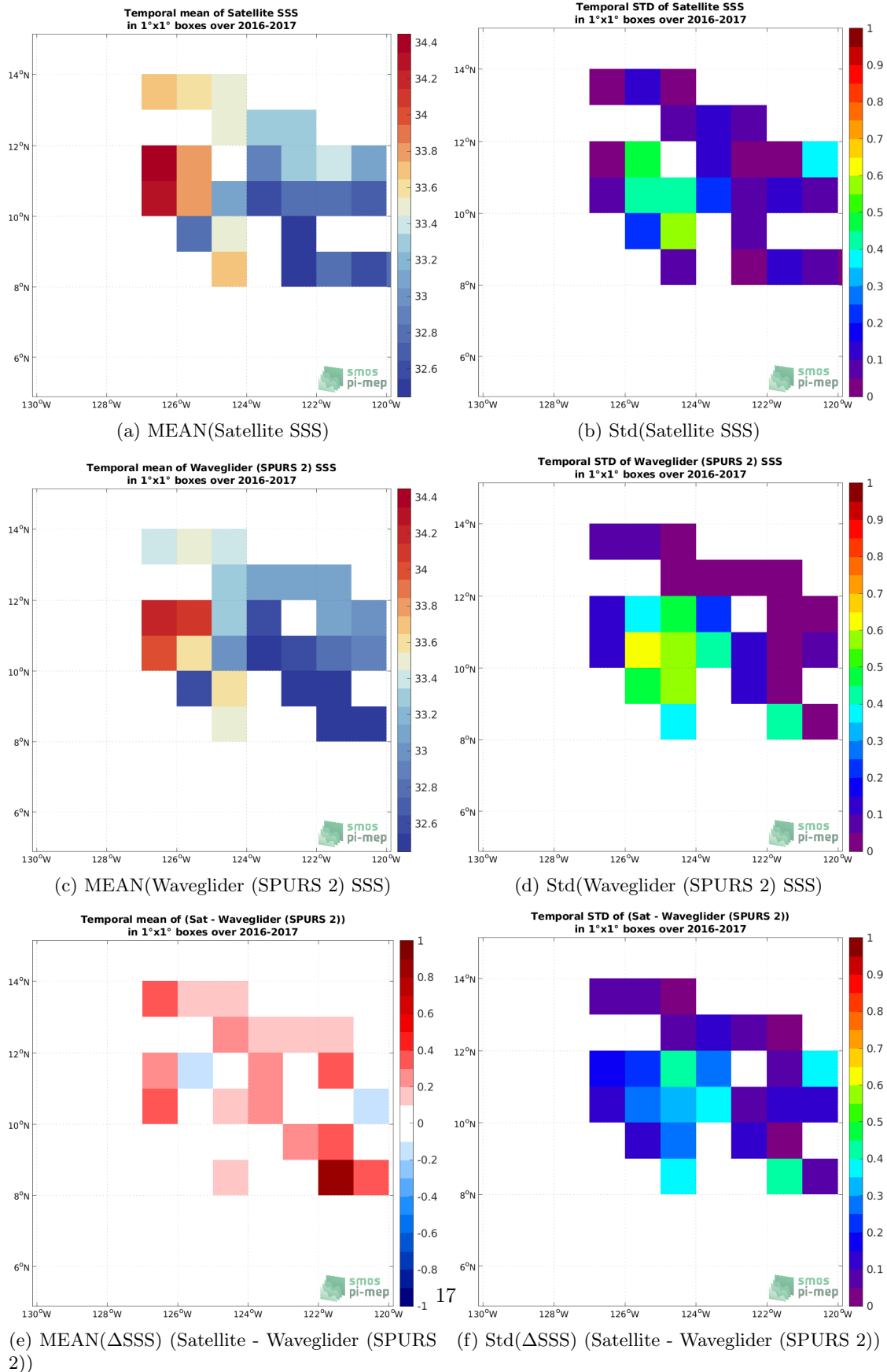
Figure 6: Temporal mean (left) and Std (right) of SSS from SMOS SSS L3 v335 - Monthly - 25 km (CATDS-CPDC) (top), Waveglider (SPURS 2) (middle), and of \Delta SSS (Satellite - Waveglider (SPURS 2)). Only match-up pairs are used to generate these maps.
