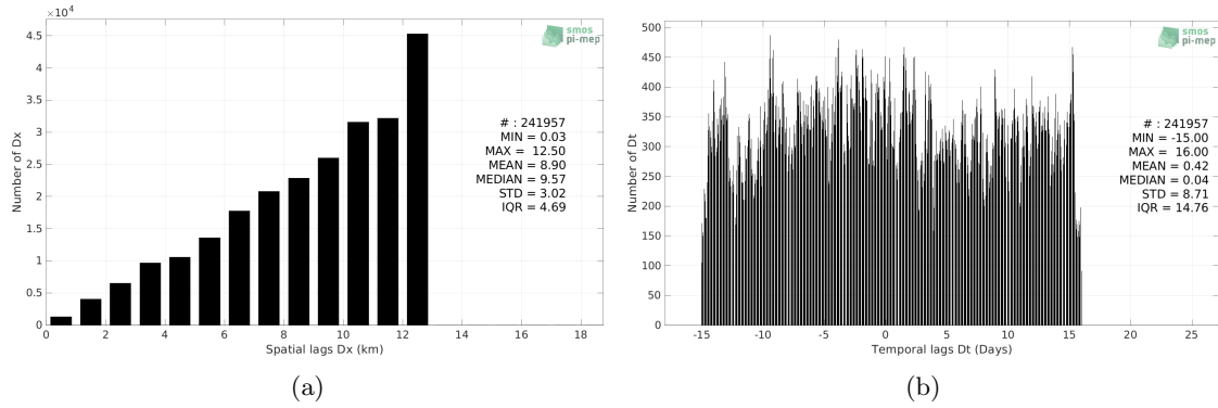
Figure 5: Histograms of the spatial (a) and temporal (b) lags between the location/time of the Waveglider (SPURS 2) measurement and the date of the corresponding SMOS SSS L3 v335 - Monthly - 25 km (CATDS-CPDC) SSS pixel.
