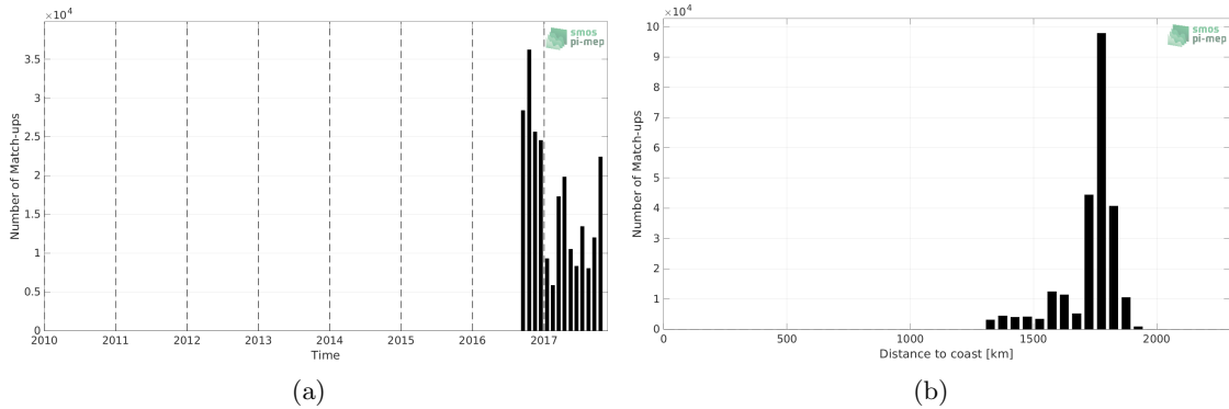
Figure 1: Number of match-ups between Waveglider (SPURS 2) and SMOS SSS L3 v335 - Monthly - 25 km (CATDS-CPDC) SSS as a function of time (a) and as function of the distance to coast (b) over the SPURS 2 Pi-MEP region and for the full satellite product period.
