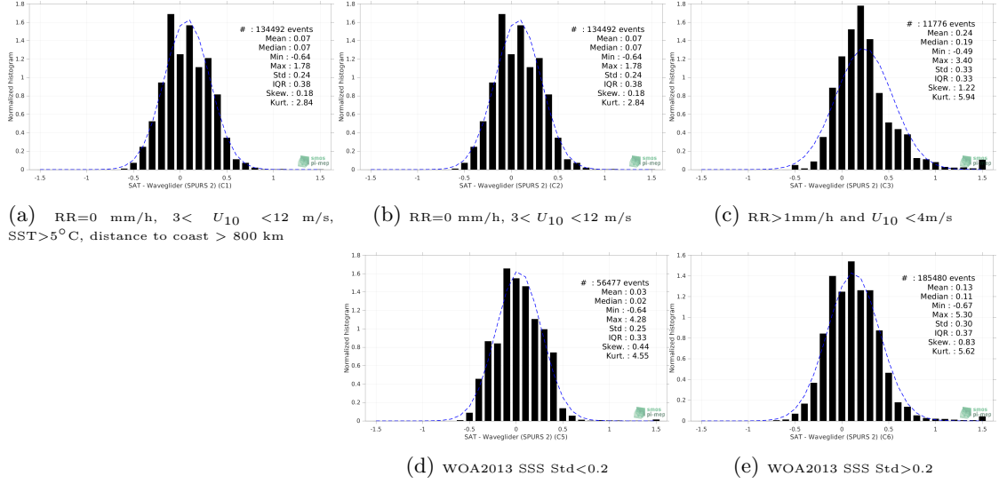
Figure 13: Normalized histogram of \Delta SSS (SMOS SSS L3 v335 - Monthly - 25 km (CATDS-CPDC) - Waveglider (SPURS 2)) for 5 different subdatasets corresponding to: RR=0 mm/h, 3 < U_{10} < 12 m/s, SST>5°C, distance to coast > 800 km (a), RR=0 mm/h, 3 < U_{10} < 12 m/s (b), RR>1mm/h and U_{10} < 4 m/s (c), WOA2013 SSS Std<0.2 (d), WOA2013 SSS Std>0.2 (e).
