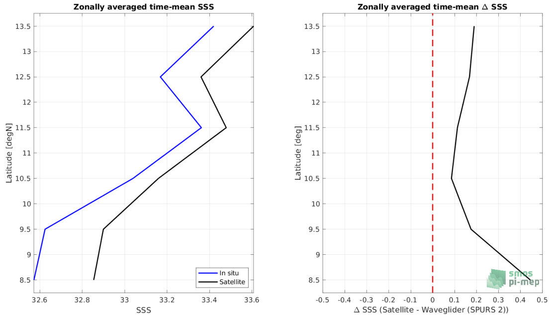
Figure 8: Left panel: Zonal mean SSS from SMOS SSS L3 v335 - Monthly - 25 km (CATDS-CPDC) satellite product (black) and from Waveglider (SPURS 2) (blue). Right panel: Zonal mean of \Delta SSS (Satellite - Waveglider (SPURS 2)) for all the collected Pi-MEP match-up pairs estimated over the full satellite product period.
