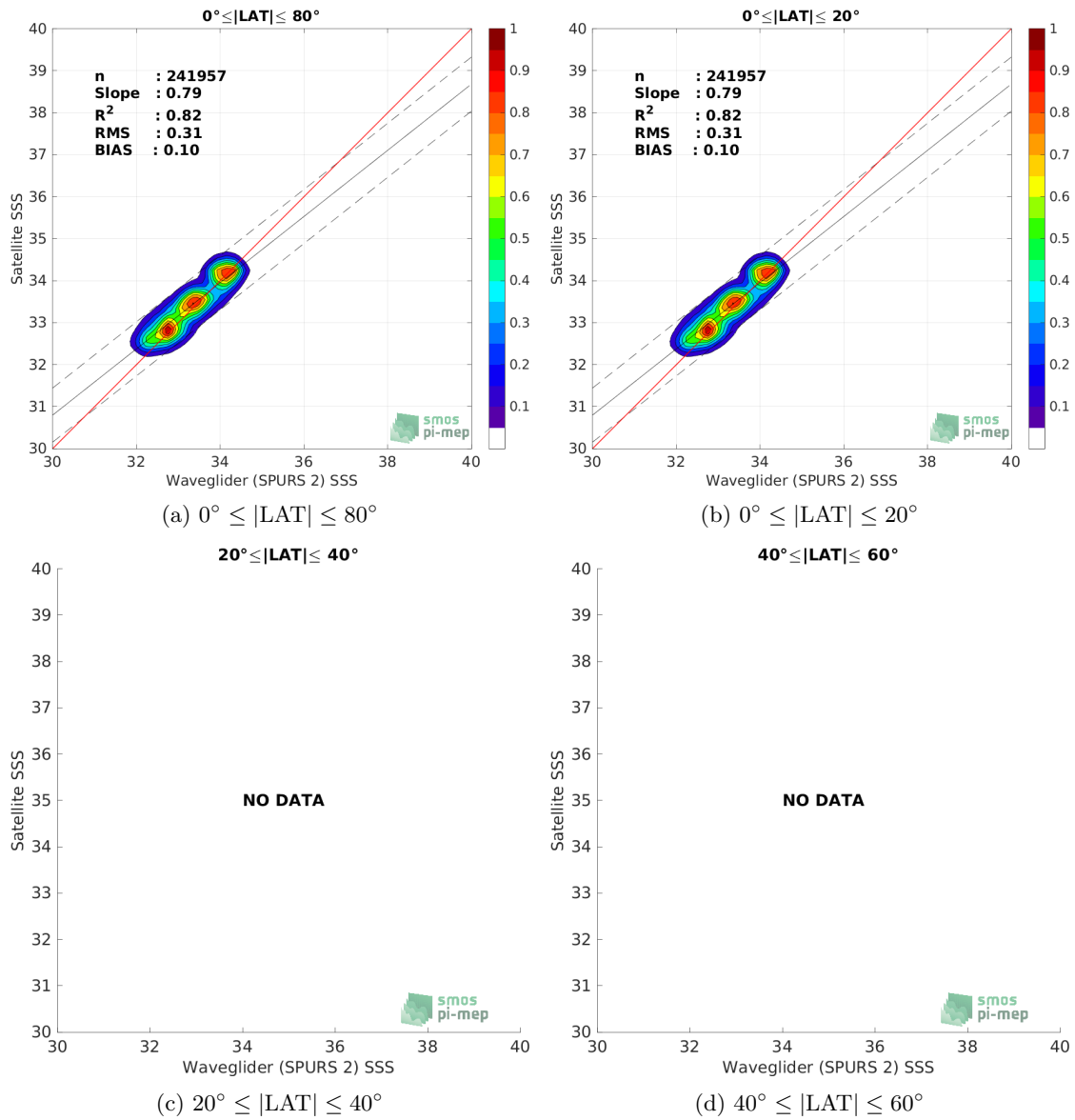
Figure 9: Contour maps of the concentration of SMOS SSS L3 v335 - Monthly - 25 km (CATDS-CPDC) SSS (y-axis) versus Waveglider (SPURS 2) SSS (x-axis) at match-up pairs for different latitude bands. For each plot, the red line shows x=y . The black thin and dashed lines indicate a linear fit through the data cloud and the \pm 95\% confidence levels, respectively. The number match-up pairs n , the slope and R^2 coefficient of the linear fit, the root mean square (RMS) and the mean bias between satellite and in situ data are indicated for each latitude band in each plots.
