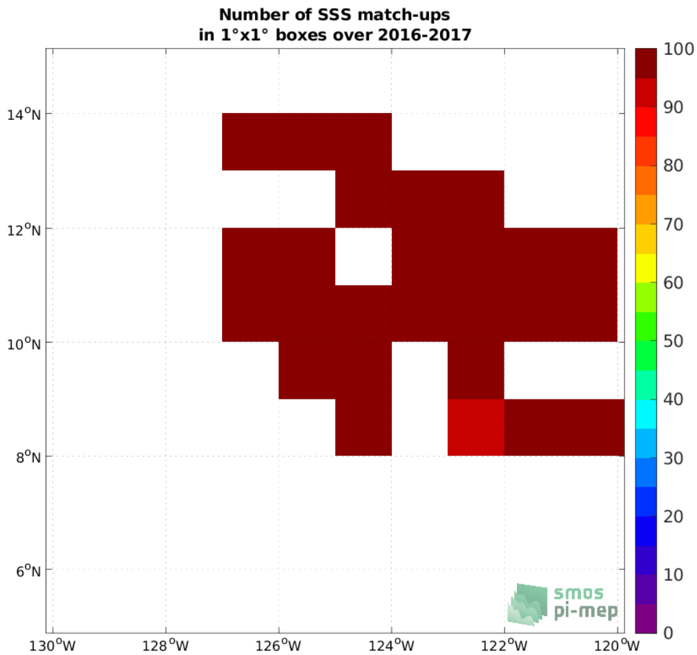
Figure 4: Number of SSS match-ups between Waveglider (SPURS 2) SSS and the SMOS SSS L3 v335 - Monthly - 25 km (CATDS-CPDC) SSS product for the SPURS 2 Pi-MEP region over 1^\circ \times 1^\circ boxes and for the full satellite product period.
