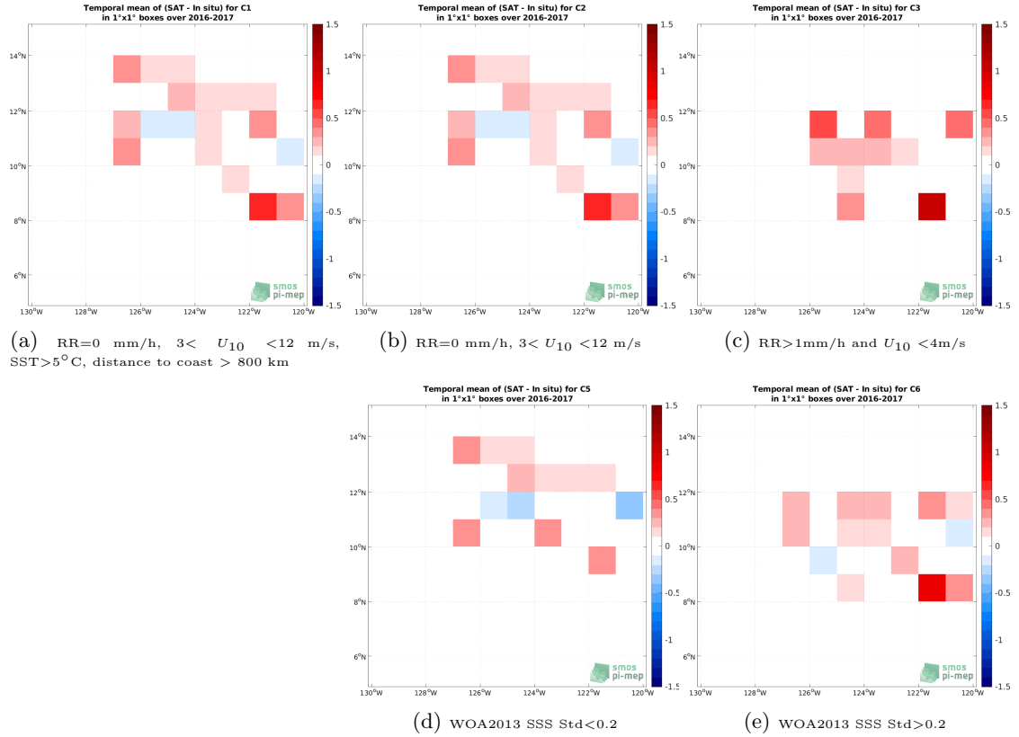
Figure 12: Temporal mean gridded over spatial boxes of size 1^{\circ}\times 1^{\circ} of \Delta\text{SSS} (SMOS SSS L3 v335 - Monthly - 25 km (CATDS-CPDC) - Waveglider (SPURS 2)) for 5 different subdatasets corresponding to:RR=0 mm/h, 3 < U_{10} < 12 m/s, SST > 5^{\circ}\text{C} , distance to coast > 800 km (a), RR=0 mm/h, 3 < U_{10} < 12 m/s (b), RR > 1 mm/h and U_{10} < 4 m/s (c), WOA2013 SSS Std < 0.2 (d), WOA2013 SSS Std > 0.2 (e).
