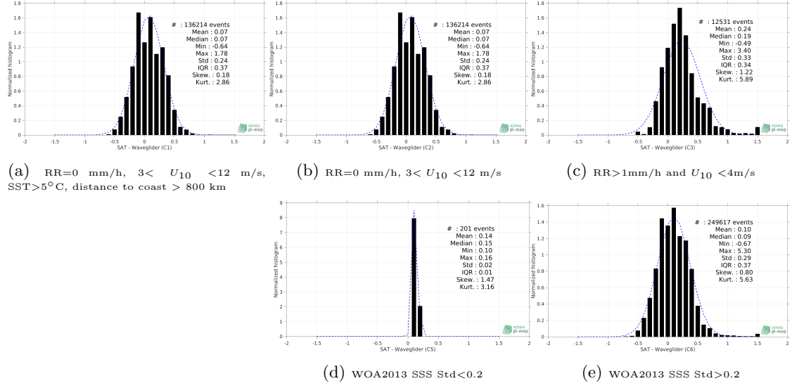
Figure 12: Normalized histogram of \Delta SSS (SMOS SSS L3 v335 - Monthly - 25 km (CATDS-CPDC) - Waveglider) for 5 different subdatasets corresponding to: RR=0 mm/h, 3 < U_{10} < 12 m/s, SST>5°C, distance to coast > 800 km (a), RR=0 mm/h, 3 < U_{10} < 12 m/s (b), RR>1mm/h and U_{10} < 4 m/s (c), WOA2013 SSS Std<0.2 (d), WOA2013 SSS Std>0.2 (e).
