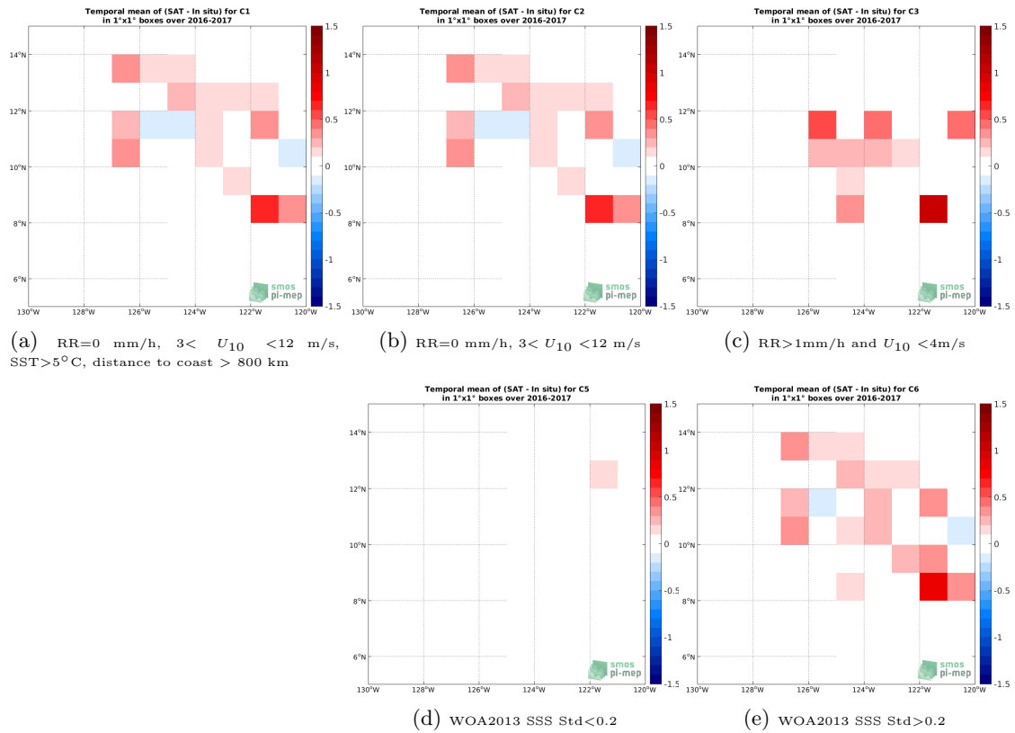
Figure 11: Temporal mean gridded over spatial boxes of size 1^\circ \times 1^\circ of \Delta SSS (SMOS SSS L3 v335 - Monthly - 25 km (CATDS-CPDC) - Waveglider) for 5 different subdatasets corresponding to:RR=0 mm/h, 3 < U_{10} < 12 m/s, SST >5^\circ\text{C} , distance to coast > 800 km (a), RR=0 mm/h, 3 < U_{10} < 12 m/s (b), RR >1 mm/h and U_{10} < 4 m/s (c), WOA2013 SSS Std <0.2 (d), WOA2013 SSS Std >0.2 (e).
